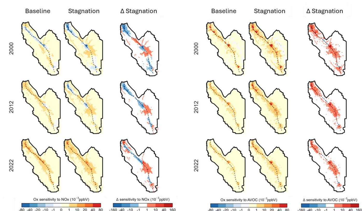
(a) Sensitivity to NO_x
