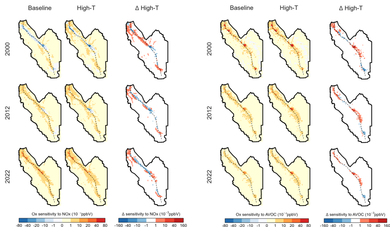
Figure 4. Sensitivities of the SJV O x receptor to (a) NO x and (b) AVOC emissions under baseline and high-T conditions for 2000, 2012, and 2022. Each panel shows sensitivities under baseline (left column), high-T (middle column), and the difference (high-T minus baseline, right column), with each row corresponding to a different emission inventory year. Higher values indicate larger contributions from the corresponding source locations to the SJV O x receptor.
