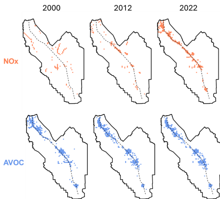
Figure 8. Optimal SJV emission source locations to target for control where sensitivities to NO_x (top row) and AVOC (bottom row) emissions consistently rank in the top 10% across meteorological scenarios in 2000, 2012, and 2022. The dashed line represents Highway 99.
