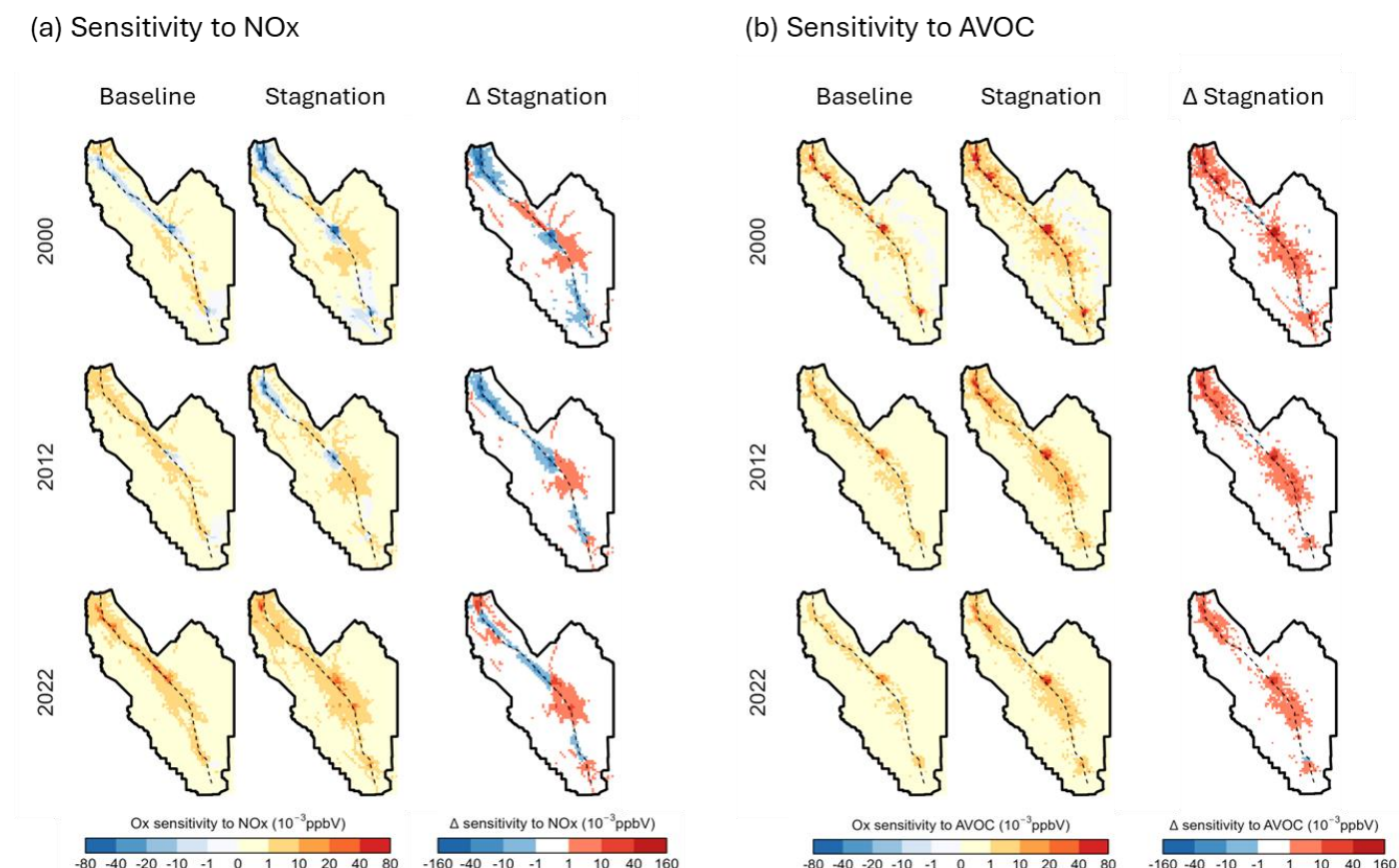
Figure 7. Sensitivities of SJV O_x to (a) NO_x and (b) AVOC emissions under baseline and stagnant conditions. Each panel shows sensitivities under baseline (left column), stagnation (middle column), and the difference (stagnation minus baseline, right column), with each row corresponding to different emission inventory scenarios. Higher values indicate larger contributions from the corresponding source locations to SJV O_x .
