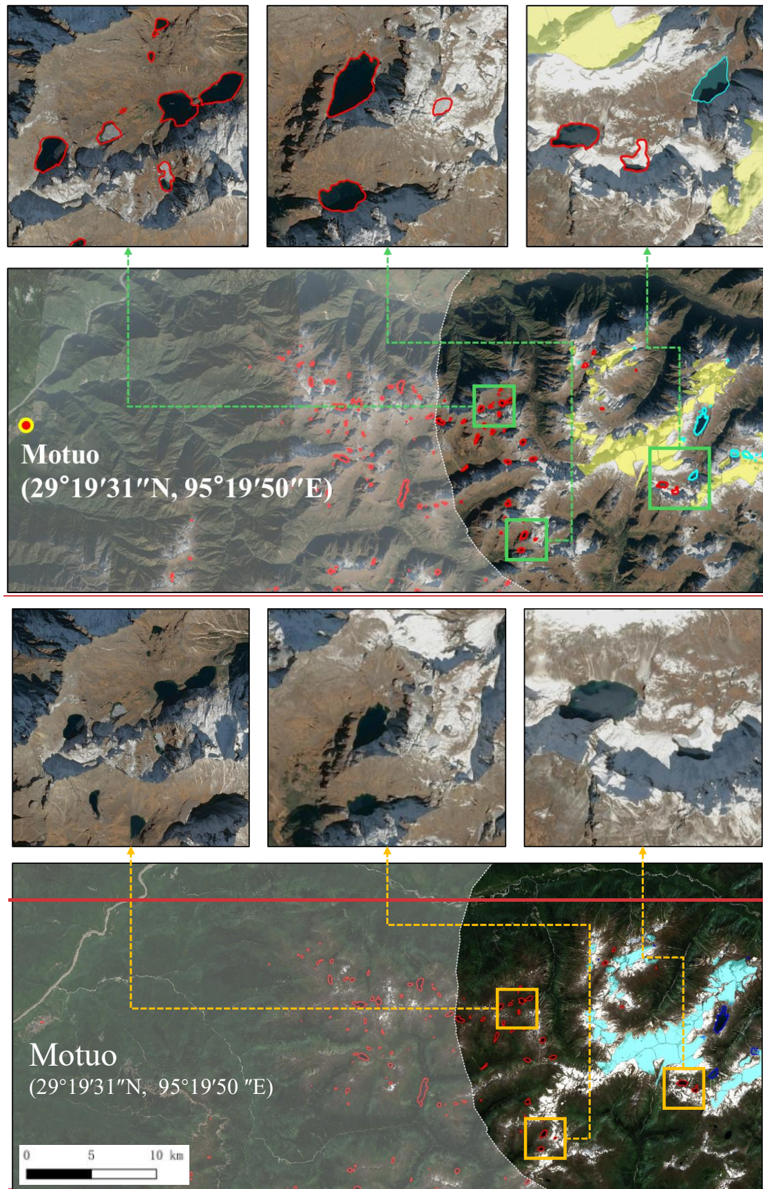
625 Figure 9. Example illustrating the limitation of a glacier-distance threshold, shown here using a 10 km buffer, in an area approximately 30 km Distribution of lakes in alpine periglacial environments in an area
