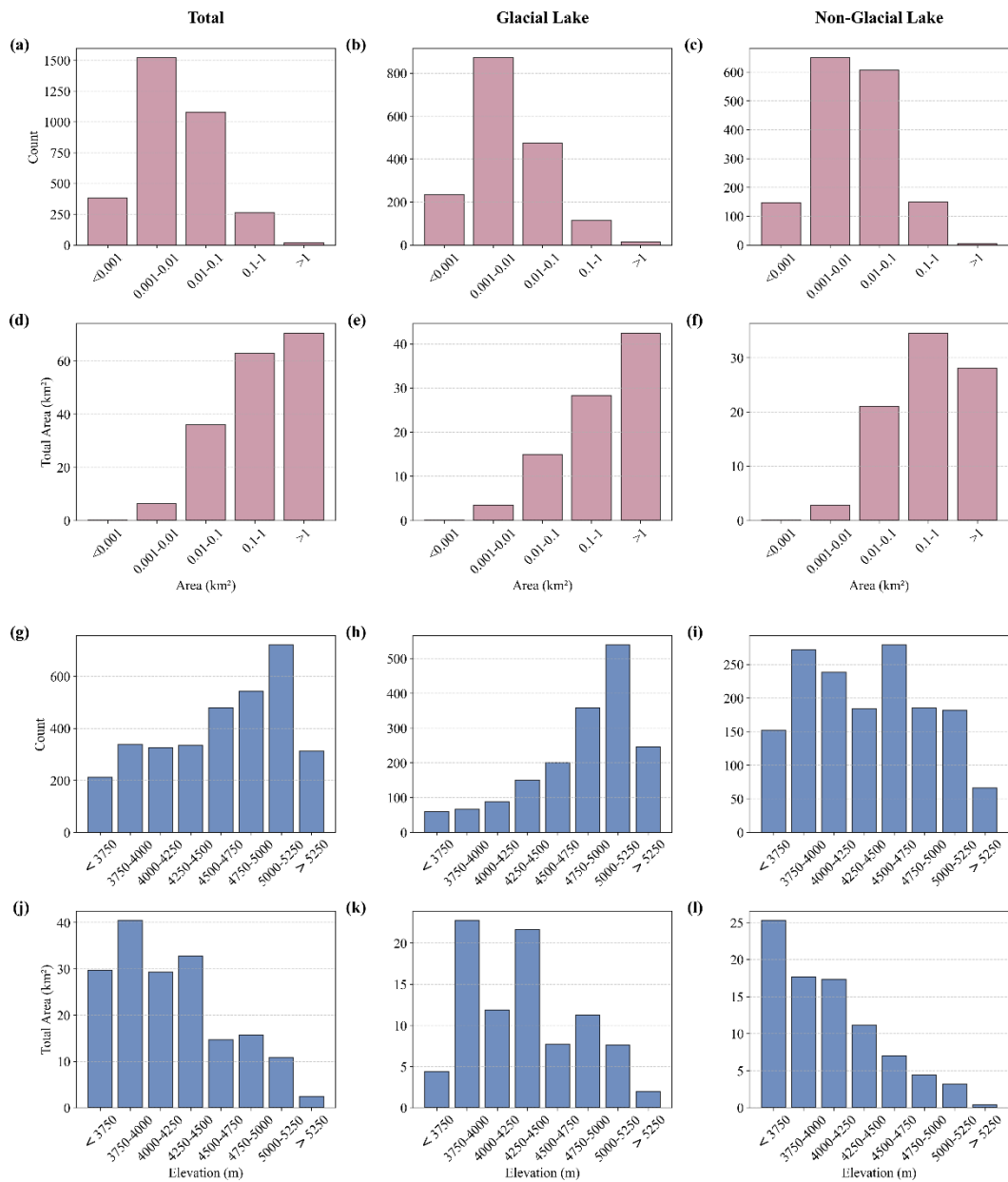
Figure 7. Size- and elevation-classified distributions of lakes in alpine periglacial environments of the STPG. Panels (a–c) show lake counts by size class for all lakes, glacial lakes, and non-glacial lakes, respectively, while panels (d–f) show the corresponding total lake area. Panels (g–i) present lake counts by elevation band, and panels (j–l) show the corresponding total lake area for all lakes, glacial lakes, and
