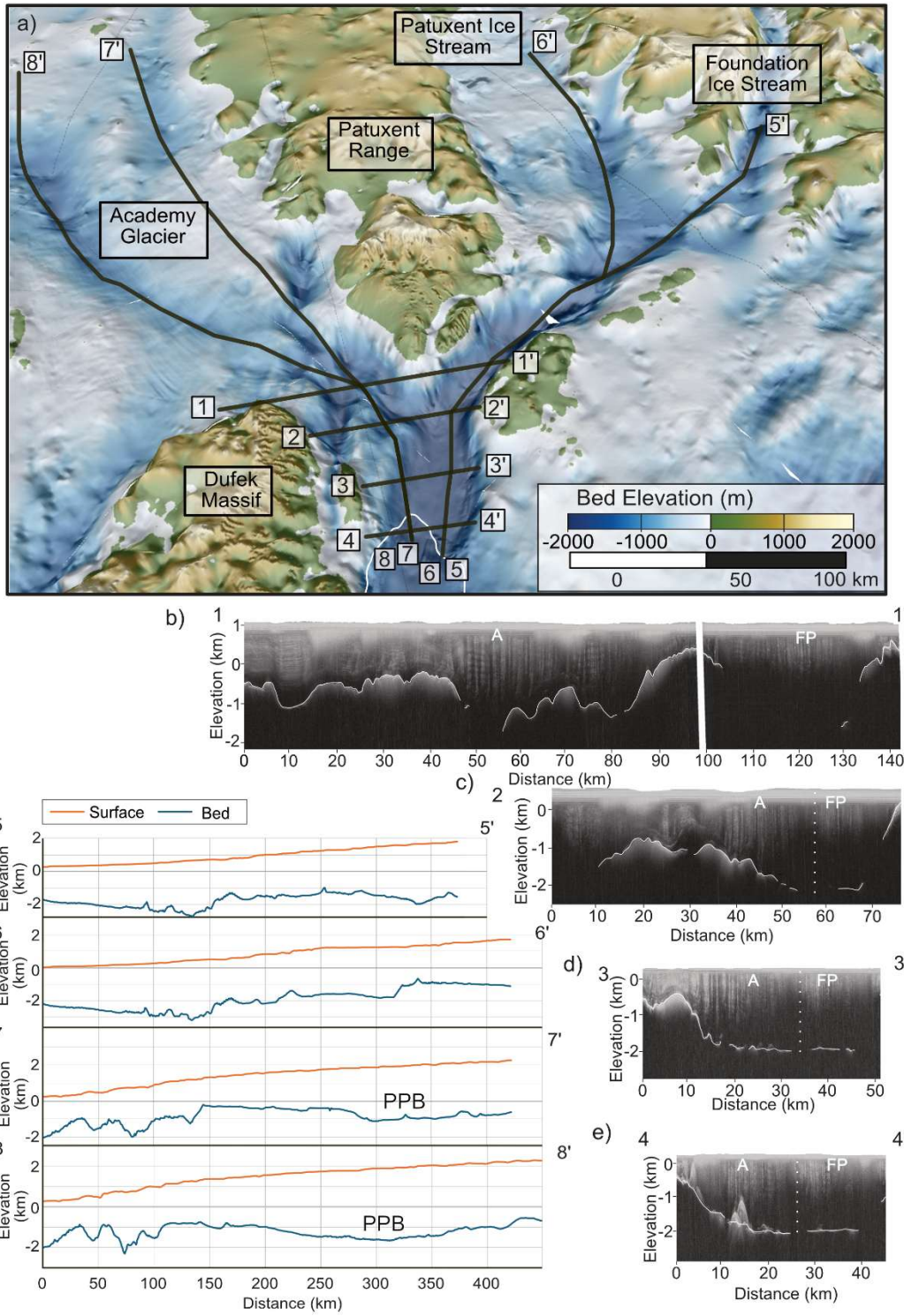
160 Figure 2: Perspective view of topography and geometry of lower trunk of FPAS, illustrating low ice surface elevation, and extent, size and depth (> 2 km below sea level) of the Foundation-Thiel trough beneath the FPAS trunk. (a) 3D bed topography (Bedmap3, Pritchard et al., 2025) with profile lines shown in subplots b-i. Bedmap3 is used in this figure as this product emphasises the deep troughs beneath the FPAS. View is into the ice sheet from the grounding zone. Grounding line (Pritchard et al., 2025) is white line; Black lines are approximate locations of radar profiles shown in b-e and topographic profiles in f-i; (b-e) radargrams, with ice thickness picks (white lines) overlain, from the Filchner Ice Shelf System (FISS) survey (profiles 1-4 on 'a' - radar transect names: FISS2015_FOU1 (b), FISS2015_FOU2 (c), FISS2015_FOU4 (d), FISS2015_FOU6 (e)) (Nicholls et al., 2024). The bright 'englacial' reflections ~12-16 km along 4-4' represent ice shelf channels; (f-i) Glacier surface (orange) and bed (blue) profile elevations (Bedmap3) for Foundation Ice Stream (profile 5 on 'a'), Patuxent Ice Stream (profile 6 on 'a') and Academy Glacier (profiles 7 & 8 on 'a'). 0 m on x-axes of f-i represents position of Bedmap3 grounding line. On b-e: A = Academy Glacier, FP = Foundation-Patuxent (vertical dashed lines mark boundary between the two flow zones). On h-i: PPB = Pensacola-Pole Basin. 165
