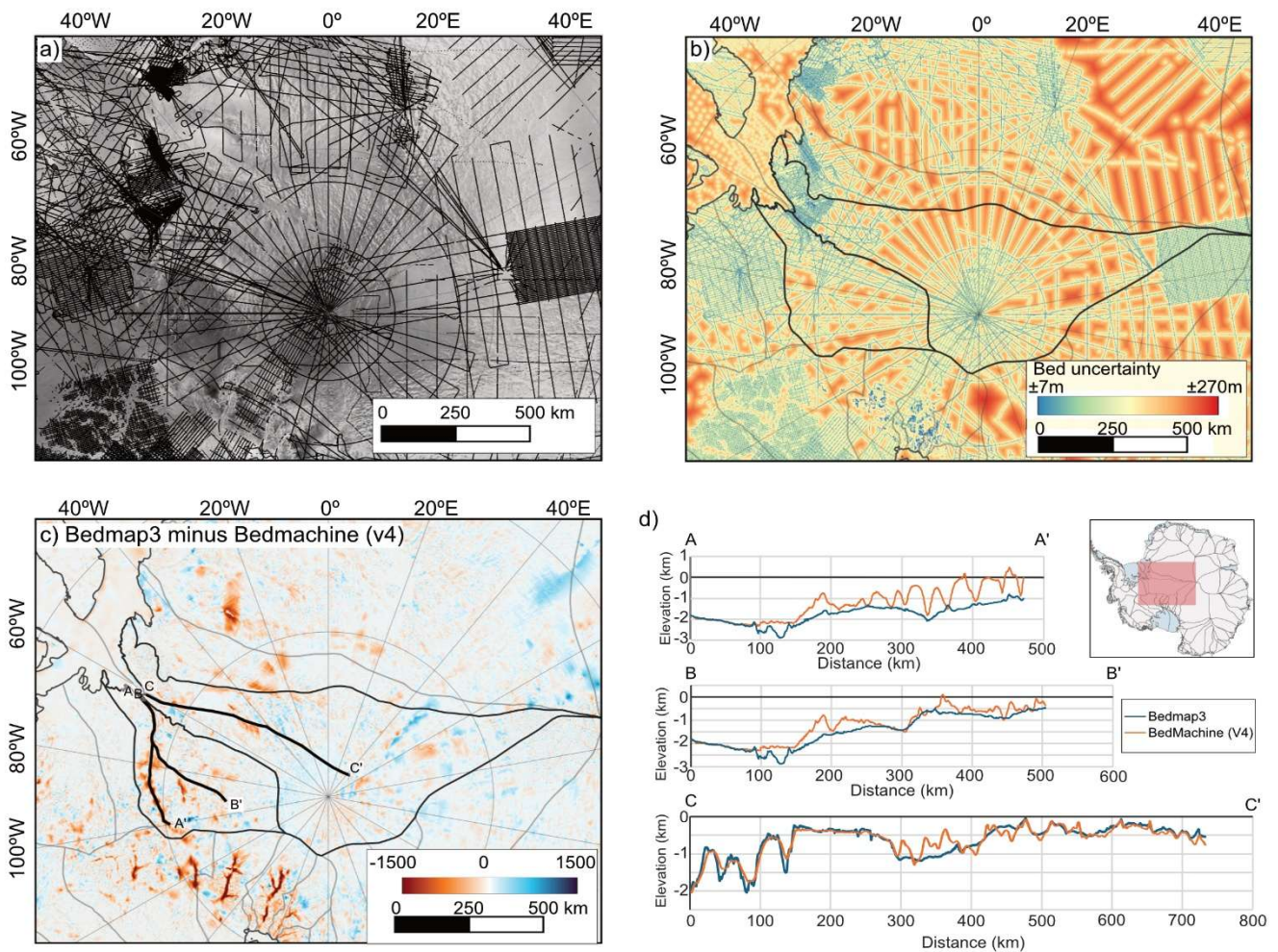
270 Figure 3: FPAS bed topography data and uncertainty demonstrating: (i) remaining uncertainty in bed topography for the FPAS; (ii) substantive differences between Bedmap3 (Pritchard et al., 2025) and BedMachine (v4) (Morlighem, 2025) bed topography datasets; and (iii) the impact of manual modification of the Bedmap3 gridded product via ‘streamlines’: a) location of the ice thickness measurements (black lines) used to derive Bedmap3 (Pritchard et al., 2025) underlain by RADARSAT-1 Antarctic Mapping Project (RAMP) SAR Image Mosaic of Antarctica (Jezek et al., 2013); b) Uncertainty in the elevation of the grounded bed (Bedmap3) (Pritchard et al., 2025); c) Difference in bed topography between Bedmap3 and BedMachine (v4) (blue indicates that the Bedmap3 bed is higher, red that it is lower). Profile lines for panel ‘d’ (thick black lines) follow Bedmap3 streamlines generated to ‘burn-in’ troughs into the dataset (Pritchard et al., 2025); d) Along-streamline topographic profiles from Bedmap3 (blue) and BedMachine (v4) (orange) of Foundation Ice Stream (A), Patuxent Ice Stream (B) and Academy Glacier (C). Location of the three profiles is shown in ‘c’. In ‘b-c’ black line is the Bedmap3 grounding line (Pritchard et al., 2025) and the grey lines are the IMBIE mass balance basins (Mouginot et al., 2017), with FPAS sub-catchments outlined in black. Inset map shows extent of a-c (pink rectangle). 275
