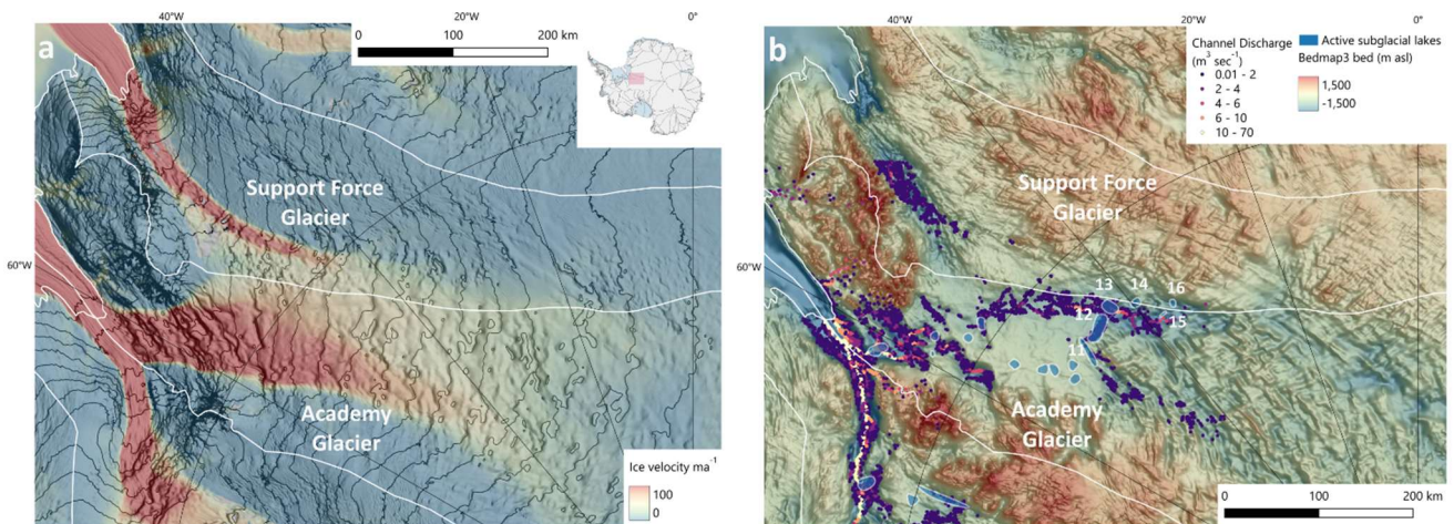
430 Figure 7: Ice catchment boundary zone between Academy and Support Force glaciers showing potential for ice-flow switching (i.e. for Academy to capture part of the Support Force Glacier catchment, or vice versa) and for water piracy due to geometry of both ice surface and bed topography. (a) Ice velocity (Mouginot et al., 2019) overlain on hillshade of Bedmap3 ice surface DEM (Pritchard et al., 2025). Black lines are ice surface contours at 100 m intervals. White lines are Ice Sheet Mass Balance Inter-comparison Exercise (IMBIE) catchments (Mouginot et al., 2017); (b) BedMachine v4 bed topography (Morlighem et al., 2025), overlain by modelled subglacial channel discharge (Ehrenfeucht et al., 2025). White lines are Ice Sheet Mass Balance Inter-comparison Exercise (IMBIE) catchments (Mouginot et al., 2017) and Bedmap3 grounding zones (Pritchard et al., 2025). Active subglacial lakes (Smith et al., 2009) are shown for the FPAS catchment. Lakes (Academy 12-16) proximal to, or below, the Support Force-Academy ‘shear margin’ as defined by the IMBIE catchment boundary are labelled. Bed topography in ‘b’ is transparent with a hillshade of the 435
