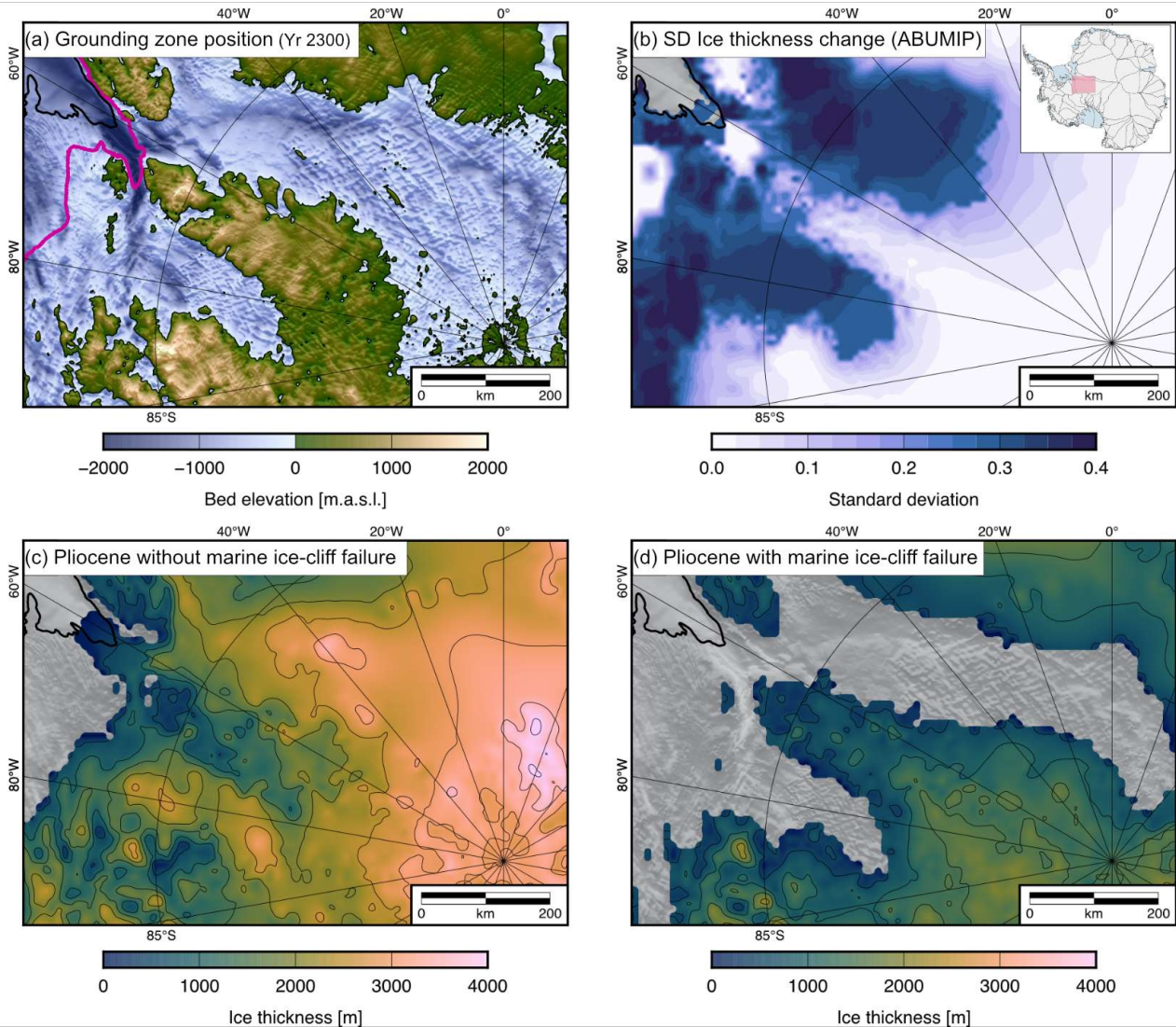
565 Figure 9: Numerical ice-sheet modelling of past and future FPAS retreat. (a) Potential 2300 CE grounding zone position (magenta line) under RCP8.5 climate forcing from ice-sheet model simulations (Hill et al., 2021) using a high-impact, low-likelihood combination of input parameters. Present-day BedMachine v4 bed topography (Morlighem et al., 2025) is shown for reference. (b) Standard deviation of the percentage ice thickness change across a multi-model ensemble from the Antarctic BUTtressing Model Intercomparison Project (ABUMIP); simulations are run for 500 model-years, with high melt rates applied beneath ice shelves to force rapid loss and debuttressing (Sun et al., 2020). (c) Simulated ice thickness under Pliocene conditions (DeConto et al., 2021); marine ice-sheet instability feedbacks are incorporated, but marine ice-cliff failure physics are switched off. (d) Simulated ice thickness during the warmth of the Pliocene (DeConto et al., 2021), with marine ice-cliff failure physics switched on. Modelled grounding zone position in c and d are indicated by the boundary between the grey and thickness-coloured parts of these subplots. Modern-day grounding zone position in a-d indicated by black line (Pritchard et al., 2025). Inset map shows extent of a-d (pink rectangle). 570 575
