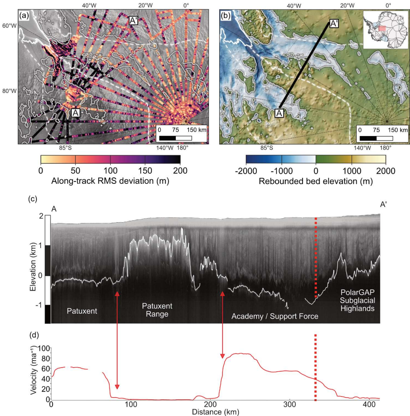
320 Figure 4: Roughness and ice-free bed topography beneath lower parts of FPAS. (a) Along-track root mean square deviation of bed 325 elevation within a moving window of 2 km (a proxy for roughness) from PolarGAP, FISS, and Operation IceBridge RES profiles (Corr et al., 2021; Nicholls et al., 2021; CReSIS 2025; MacGregor et al., 2021), showing relatively smooth (pale yellow) zones beneath parts of Academy Glacier and Patuxent Ice Stream; (b) Rebounded ('ice-free') topography of lower FPAS derived from BedMachine 330 v2 (Paxman et al., 2022). In 'a' and 'b' the grey contour lines represent the rebounded 0 m contour, the thick white line is the Bedmap3 grounding line (Pritchard et al., 2025) and the white dashed lines are the IMBIE mass balance basins (Mouginot et al., 2017). The smoothest bed topography beneath FPAS is located below the 0 m contour (grey line) for both Academy and Foundation- Patuxent tributaries. These 'smooth' zones correspond to the model-derived low basal shear stress zones of Joughin et al. (2006), based on the BEDMAP DEM; (c) example radargram (radar transect name: POLARGAP_P13A), with ice thickness picks overlain, from the PolarGAP survey (profile A-A' on 'b') (Ferraccioli et al., 2021). Ice flow direction is into page; (d) ice velocity (Mouginot et al., 2019) along profile A-A'. Vertical dashed red line on 'c' and 'd' is the boundary between Academy and Support Force glaciers. Vertical red arrows on 'c' and 'd' denote the shear margins where Patuxent Ice Stream and Academy Glacier abut the Patuxent Range. These correspond to scattering zones in the overlying radargram. Inset map shows extent (pink rectangle) of 'a' and 'b'.
