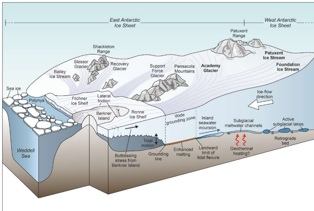
635 Figure 10: Visualisation of the Foundation Patuxent Academy System (FPAS), showing its pattern of ice flow, landscape setting, and subglacial and grounding zone processes. Also shown is the FPAS’s relationship to surrounding outlet glaciers in the Weddell Sea sector, the Filchner-Ronne Ice Shelf (including the grounded Berkner Island), the Southern Ocean, and major mountain ranges. Note that the visualisation is not true to scale, with some features exaggerated relative to others for display purposes.
