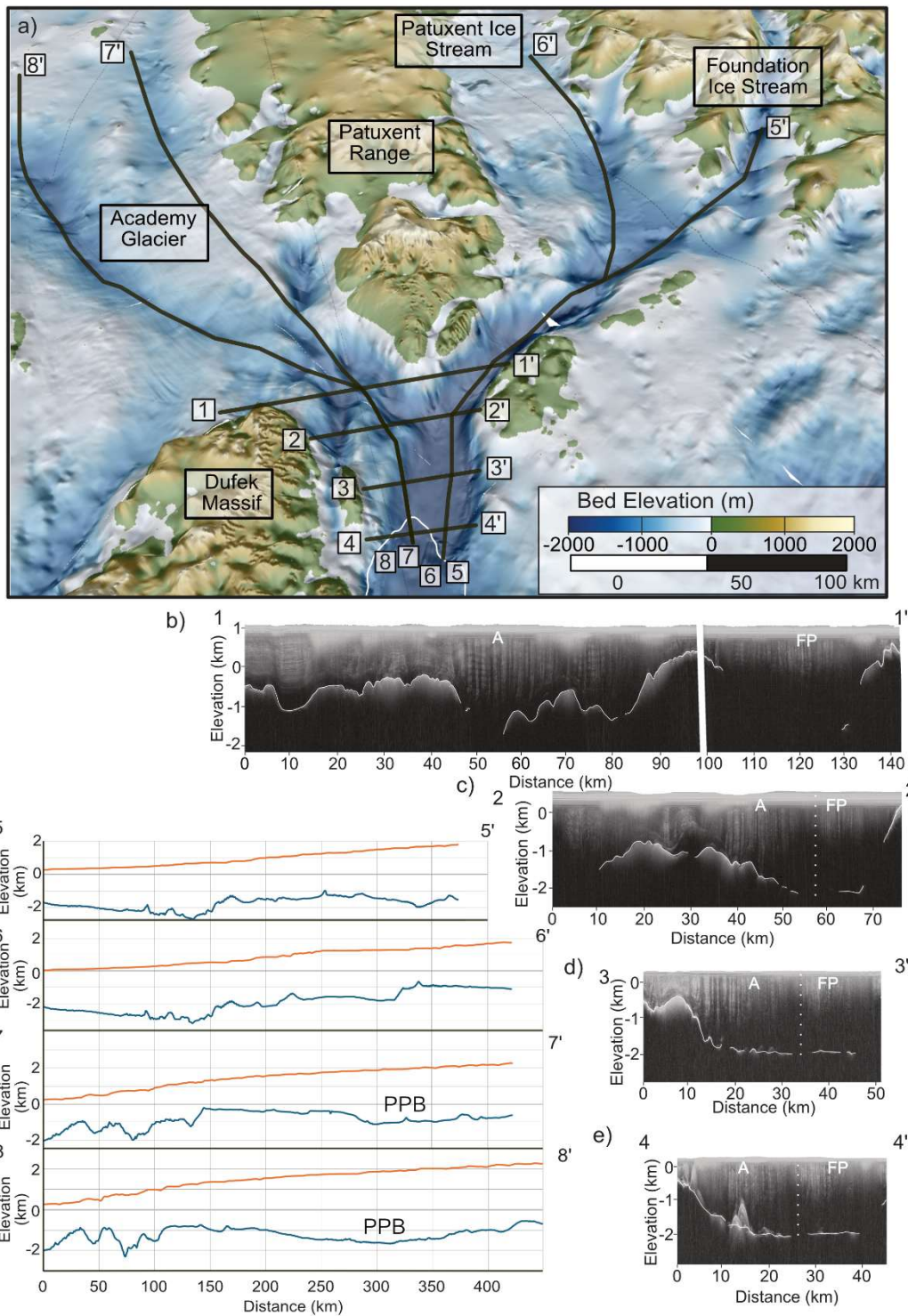
Figure 2: Perspective view of topography and geometry of lower trunk of FPAS, illustrating low ice surface elevation, and extent, size and depth ( > 2 km below sea level) of the Foundation-Thiel trough beneath the FPAS trunk. (a) 3D bed topography (Bedmap3, Pritchard et al., 2025) with profile lines shown in subplots b-i. View is into the ice sheet from the grounding zone. Grounding line (Pritchard et al., 2025) is white line; Black lines are approximate locations of radar profiles shown in b-e and topographic profiles in f-i; (b-e) radargrams, with ice thickness picks (white lines) overlain, from the Filchner Ice Shelf System (FISS) survey (profiles 1-4 on 'a' - radar transect names: FISS2015_FOU1 (b), FISS2015_FOU2 (c), FISS2015_FOU4 (d), FISS2015_FOU6 (e)) (Nicholls et al., 2024). The bright 'englacial' reflections ~12-16 km along 4-4' represent ice shelf channels; (f-i) Glacier surface (orange) and bed (blue) profile elevations (Bedmap3) for Foundation Ice Stream (profile 5 on 'a'), Patuxent Ice Stream (profile 6 on 'a') and Academy Glacier (profiles 7 & 8 on 'a'). 0 m on x-axes of f-i represents position of Bedmap3 grounding line. On b-e: A = Academy Glacier, FP = Foundation-Patuxent (vertical dashed lines mark boundary between the two flow zones). On h-i: PPB = Pensacola-Pole Basin.
