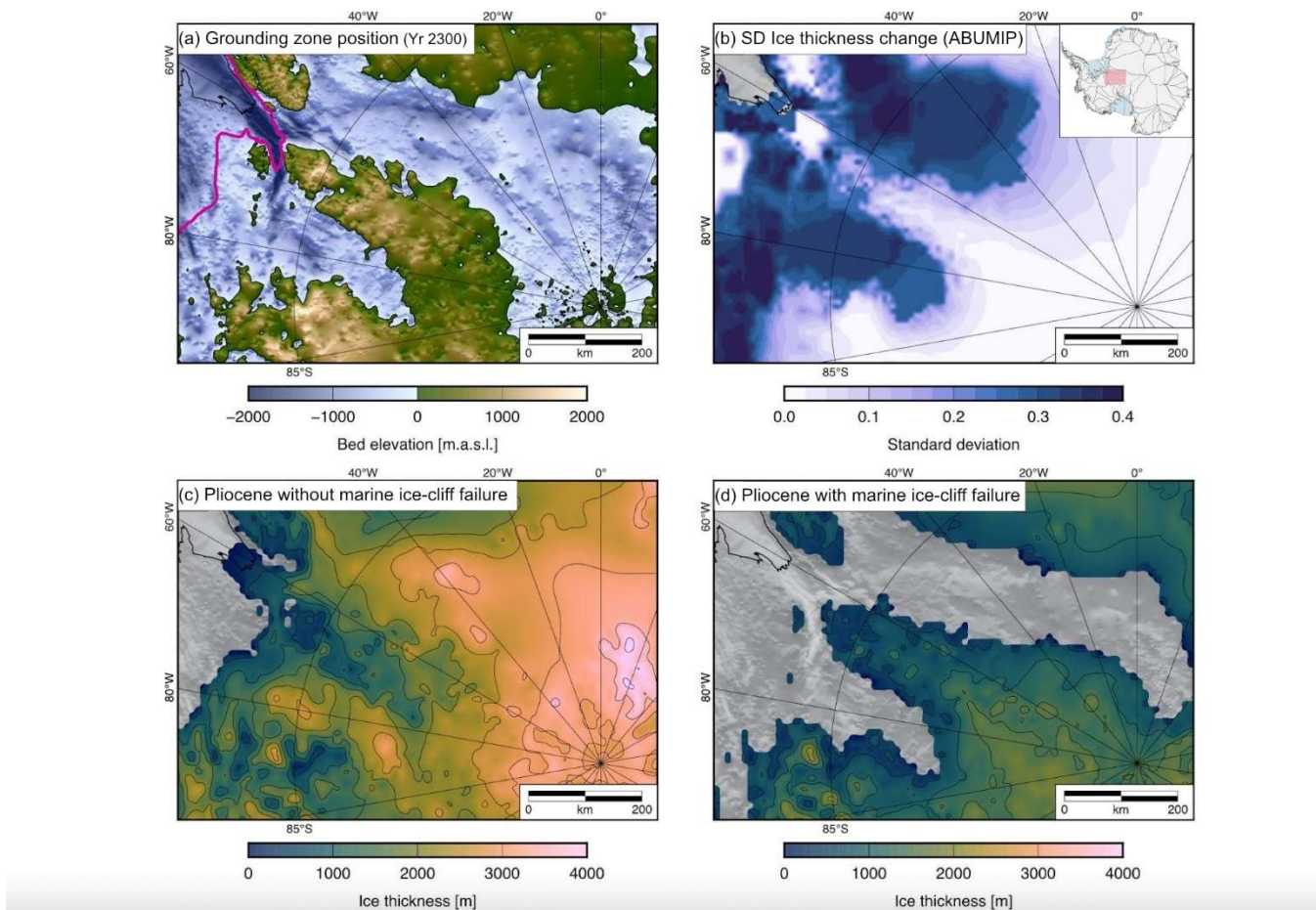
555 Figure 9: Numerical ice-sheet modelling of past and future FPAS retreat. (a) Potential 2300 CE grounding zone position (magenta line) under RCP8.5 climate forcing from ice-sheet model simulations (Hill et al., 2021) using a high-impact, low-likelihood combination of input parameters. Present-day bed topography (Morlighem et al., 2020) is shown for reference. (b) Standard deviation of the percentage ice thickness change across a multi-model ensemble from the Antarctic BUttrressing Model Intercomparison Project (ABUMIP); simulations are run for 500 model-years, with high melt rates applied beneath ice shelves to force rapid loss and debuttrressing (Sun et al., 2020). (c) Simulated ice thickness under Pliocene conditions (DeConto et al., 2021); marine ice-sheet instability feedbacks are incorporated, but marine ice-cliff failure physics are switched off. (d) Simulated ice thickness during the warmth of the Pliocene (DeConto et al., 2021), with marine ice-cliff failure physics switched on. Modelled grounding zone position in c and d are indicated by the boundary between the grey and thickness-coloured parts of these subplots. Modern-day grounding zone position in a-d indicated by black line (Rignot et al., 2016). Inset map shows extent of a-d (pink rectangle). 560 565
