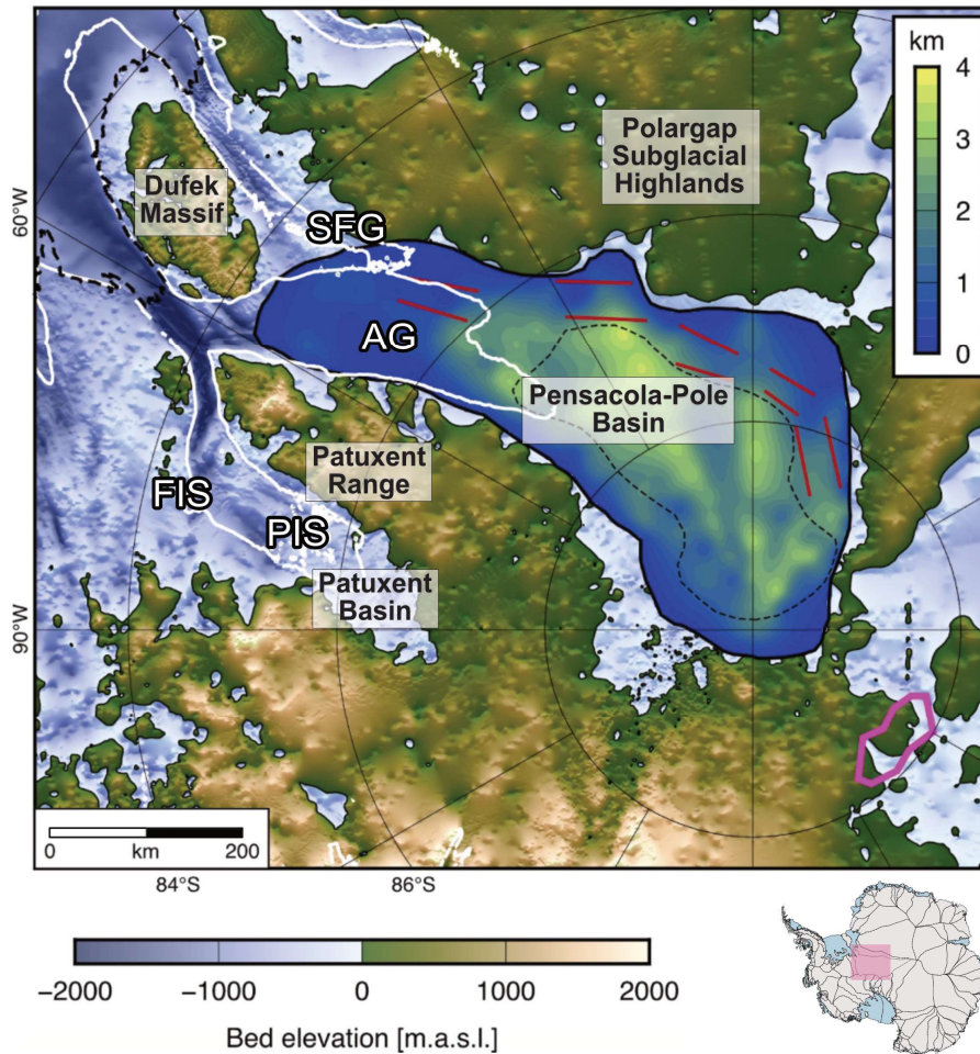
Figure 5: Geological structure of the FPAS catchment. Gravity anomaly modelling indicates that the Pensacola-Pole Basin (PPB) is underlain by a sedimentary basin 2–3 km thick in places (Paxman et al., 2019; see interior colour scale); the potential sedimentary infill within the Patuxent Basin was not analysed in Paxman et al., (2019). The southern part of the PPB (thin black dashed line) is characterised by the largest thicknesses of sedimentary fill and also exhibits topography and high-frequency magnetic anomalies characteristic of Jurassic dolerite sills, which are commonly intruded into Beacon Supergroup sediments (Paxman et al., 2019). Red lines mark a series of deep (1–2 km below sea level) troughs located along the eastern margin of the PPB. Magenta polygon demarcates a zone of basal melting attributed to elevated geothermal heat flux (Jordan et al., 2018). White line marks the 50 m/yr ice-surface velocity contour (Mouginot et al., 2019). Thick black dashed line marks the grounding zone (Rignot et al., 2016). Bed topography is from BedMachine v3 (Morlighem et al., 2020). Outlet glaciers are: Foundation Ice Stream (FIS), Academy Glacier (AG), Patuxent Ice Streams (PIS), Support Force Glacier (SFG). Inset map shows extent of figure (pink rectangle).
