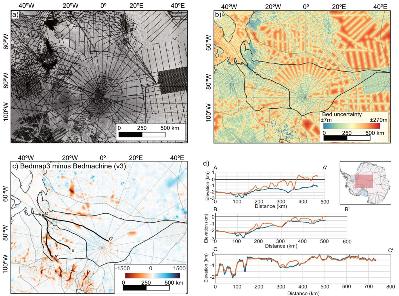
Figure 3: FPAS bed topography data and uncertainty demonstrating: (i) remaining uncertainty in bed topography for the FPAS; (ii) substantive differences between Bedmap3 and BedMachine (v3) bed topography datasets; and (iii) the impact of manual modification of the Bedmap3 gridded product via ‘streamlines’: a) location of the ice thickness measurements (black lines) used to derive Bedmap3 (Pritchard et al., 2025) underlain by RADARSAT-1 Antarctic Mapping Project (RAMP) SAR Image Mosaic of Antarctica (Jezek et al., 2013); b) Uncertainty in the elevation of the grounded bed (Bedmap3) (Pritchard et al., 2025); c) Difference in bed topography between Bedmap3 and BedMachine (v3) (blue indicates that the Bedmap3 bed is higher, red that it is lower). Profile lines for panel ‘d’ (thick black lines) follow Bedmap3 streamlines generated to ‘burn-in’ troughs into the dataset (Pritchard et al., 2025); d) Along-streamline topographic profiles from Bedmap3 (blue) and BedMachine (v3) (orange) of Foundation Ice Stream (A), Patuxent Ice Stream (B) and Academy Glacier (C). Location of the three profiles is shown in ‘c’. In ‘b-c’ black line is the Bedmap3 grounding line (Pritchard et al., 2025) and the grey lines are the IMBIE mass balance basins (Mouginot et al., 2017), with FPAS sub-catchments outlined in black. Inset map shows extent of a-c (pink rectangle).
