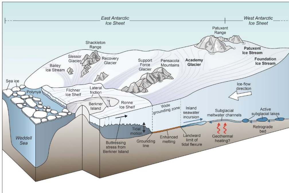
625 Figure 10: Visualisation of the Foundation Patuxent Academy System (FPAS), showing its pattern of ice flow, landscape setting, and subglacial and grounding zone processes. Also shown is the FPAS’s relationship to surrounding outlet glaciers in the Weddell Sea sector, the Filchner-Ronne Ice Shelf (including the grounded Berkner Island), the Southern Ocean, and major mountain ranges. Note that the visualisation is not true to scale, with some features exaggerated relative to others for display purposes.
