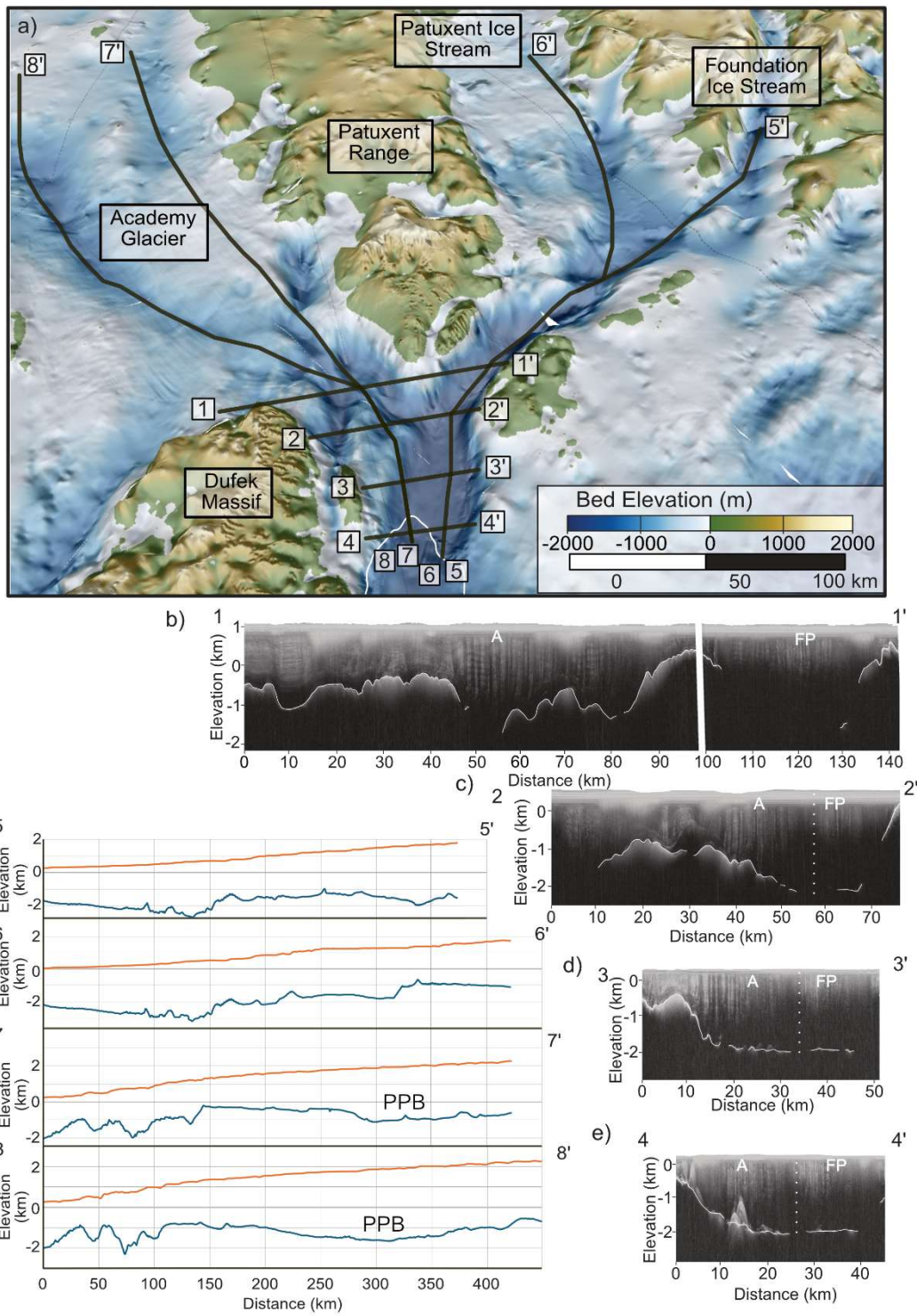
165 Figure 2: Perspective view of topography and geometry of lower trunk of FPAS, illustrating low ice surface elevation, and extent, size and depth (> 2 km below sea level) of the Foundation-Thiel trough beneath the FPAS trunk. (a) 3D bed topography (Bedmap3, Pritchard et al., 2025) with profile lines shown in subplots b-i. View is into the ice sheet from the grounding zone. Grounding line (Pritchard et al., 2025) is white line; Black lines are approximate locations of radar profiles shown in b-e and topographic profiles 170 in f-i; (b-e) radargrams, with ice thickness picks (white lines) overlain, from the Filchner Ice Shelf System (FISS) survey (profiles 1- 4 on 'a' - radar transect names: FISS2015 FOU1 (b), FISS2015 FOU2 (c), FISS2015 FOU4 (d), FISS2015 FOU6 (e) ) (Nicholls et al., 2024). The bright 'englacial' reflections ~12-16 km along 4-4' represent ice shelf channels; (f-i) Glacier surface (orange) and bed (blue) profile elevations (Bedmap3) for Foundation Ice Stream (profile 5 on 'a'), Patuxent Ice Stream (profile 6 on 'a') and Academy Glacier (profiles 7 & 8 on 'a'). 0 m on x-axes of f-i represents position of Bedmap3 grounding line. On b-e: A = Academy Glacier, FP = Foundation-Patuxent (vertical dashed lines mark boundary between the two flow zones). On h-i: PPB = Pensacola-Pole Basin.
