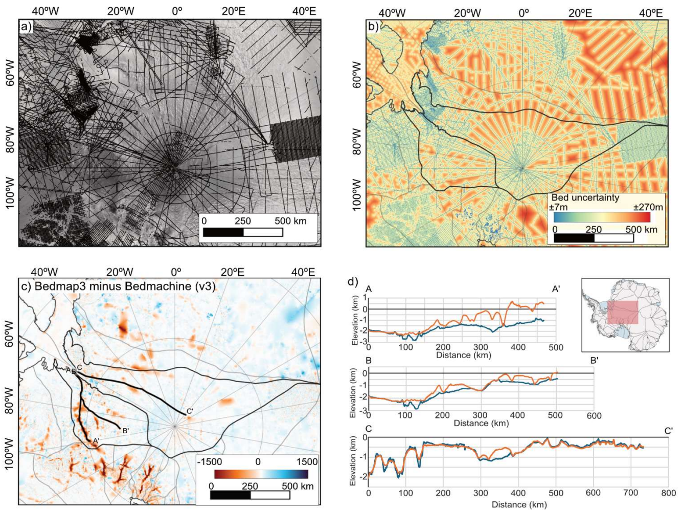
Figure 3: Evolution of the FPAS bed topography data and uncertainty over time demonstrating: (i) remaining uncertainty in bed topography for the FPAS; (ii) substantive differences between published Bedmap3 and BedMachine (v3) bed topography datasets (i.e. Bedmap2 , Bedmap3 and Bedmachine (v3) ); and (iii) the impact of manual modification of the Bedmap3 gridded product via ‘streamlines’: a) location of the ice thickness measurements (black lines) used to derive Bedmap3 (Pritchard et al., 2025) underlain by RADARSAT-1 Antarctic Mapping Project (RAMP) SAR Image Mosaic of Antarctica (Jezek et al., 2013); b) Uncertainty in the elevation of the grounded bed (Bedmap3) (Pritchard et al., 2025); c) Differences in bed topography DEMs between available products: (c) Bedmachine (v3) minus Bedmap2 (blue indicates that the Bedmachine (V3) bed is higher, red that it is lower), d) Bedmap3 minus and BedMachine (v3) (blue indicates that the Bedmap3 bed is higher, red that it is lower). Profile lines for panel ‘d’ (thick black lines) follow Bedmap3 streamlines generated to ‘burn-in’ troughs into the dataset (Pritchard et al., 2025); e) Bedmap3 minus Bedmap2 ; f) Along-streamline topographic profiles from Bedmap3 (blue) and Bedmachine-BedMachine (v3) (orange) of Foundation Ice Stream (A), Patuxent Ice Stream (B) and Academy Glacier (C). Location of the three profiles is shown in ‘d’c’. Geographic features are: Foundation Ice Stream (FIS) , Patuxent Ice Stream (PIS) , Academy Glacier (AG) and Support Foree Glacier (SFG) . In ‘b-e’c’ thick black line is the Bedmap3 grounding line (Pritchard et al., 2025) and the grey dashed lines are the IMBIE mass balance basins (Mouginot et al., 2017), with FPAS sub-catchments outlined in black. Inset map shows extent of a-c (pink rectangle).
