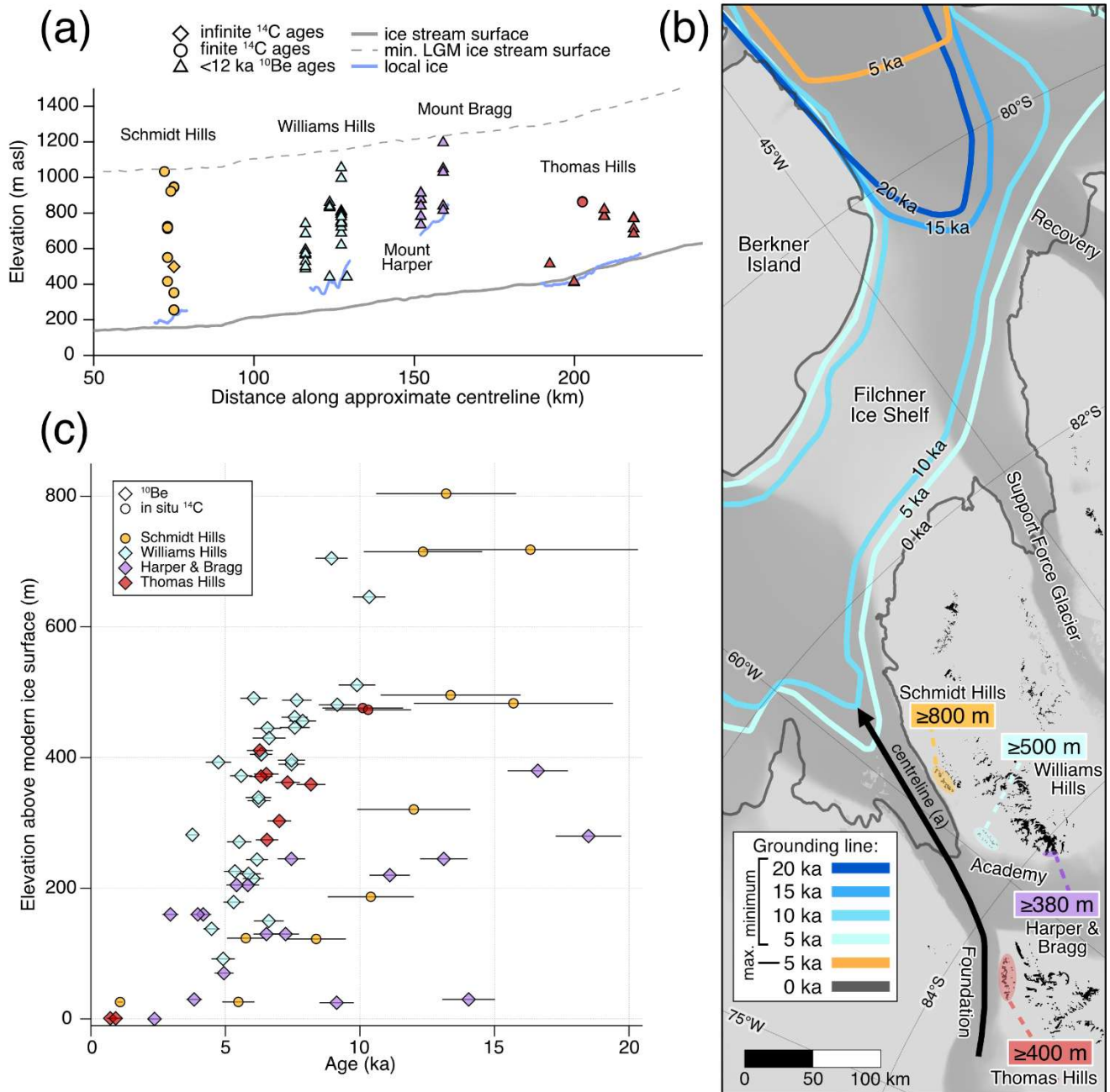
510 Figure 8: Cosmogenic nuclide exposure ages and ice surface elevation from around the FPAS trunk. (a) Exposure ages projected 515 onto an elevation profile along an approximate centreline of the Foundation Ice Stream. (b) Centreline location, minimum LGM ice thickness constraints interpreted from the exposure ages, and former grounding zone positions. (c) Exposure ages from nunataks 520 collected from nunataks adjacent to the Foundation Ice Stream. Elevation data for ice surfaces (a) are sourced from the Reference Elevation Model of Antarctica (REMA; Howat et al., 2019). Note that local ice margins in (a) are highly simplified and the minimum LGM surface is the modern surface profile with the elevation increased above present to the elevation of the highest elevation, post- LGM exposure age. Palaeo grounding zone positions are the inferred minimum (scenario A, blue) and maximum (scenario B, orange) positions of Hillenbrand et al. (2014). The modern (2011) grounding zone position and ice velocities (grey shading) are sourced from the MEASUREs program V2 (Rignot et al., 2016, 2017). Ice velocities are used to highlight ice streams (darker grey is faster ice). Exposure ages in (a) and (c) are collated from the Informal Cosmogenic-nuclide Exposure-age Database (ICE-D; https://version2.ice- d.org/antarctica/ ) and originally sourced from Balco et al. (2016), Bentley et al. (2017), and Nichols et al. (2019). Ages in ICE-D are calculated using the online exposure age calculators formerly known as the CRONUS Earth online calculators ( http://hess.ess.washington.edu ; Balco et al., 2008) with the “primary” production rate calibration data set (Borchers et al., 2016) and the “LSDn” scaling method for neutrons, protons, and muons (Lifton et al., 2014; Balco, 2017). Infinite in situ ^{14}\text{C} ages in (a) indicate continuous exposure for at least \sim 30 kyr. Panels (a) and (b) are modified from Nichols et al. (2019).
