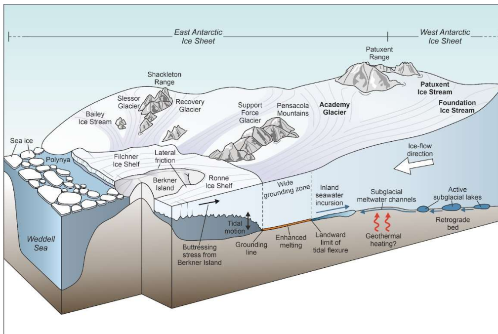
Figure 10: Visualisation of the Foundation Patuxent Academy System (FPAS), showing its pattern of ice flow, landscape setting, and subglacial and grounding zone processes. Also shown is the FPAS’s relationship to surrounding outlet glaciers in the Weddell Sea sector, the Filchner-Ronne Ice Shelf (including the grounded Berkner Island), the Southern Ocean, and major mountain ranges. Note that the visualisation is not true to scale, with some features exaggerated relative to others for display purposes.
