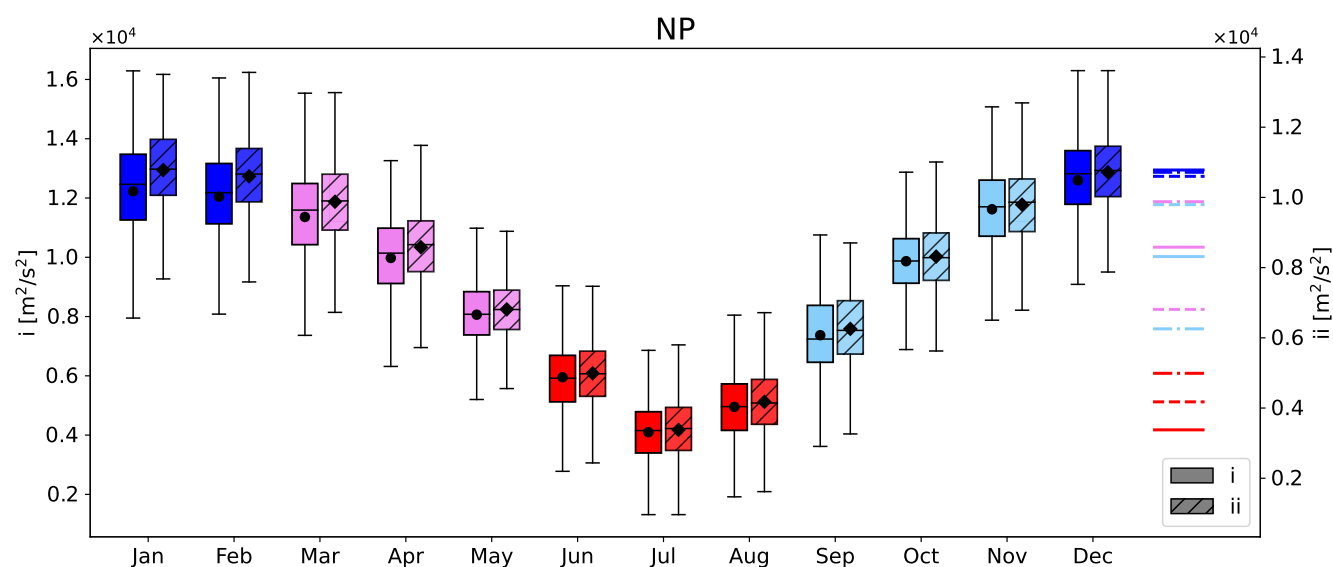
Figure B1. Boxplot showing the distribution of expression (i) in Eq. B2 and expression (ii) in Eq. B4 with y_1 = 20^\circ\text{N} , y_2 = 60^\circ\text{N} and p_0 = 900\text{ hPa} , p_1 = 250\text{ hPa} . The boxes indicate the interquartile range (IQR), with the horizontal line depicting the median and the black marker showing the mean. Whiskers extend to the most extreme data points within 1.5 times the IQR. The horizontal coloured lines on the right show the averages of expression (ii) for the different months in same colours and linestyles as in Fig. 4.
