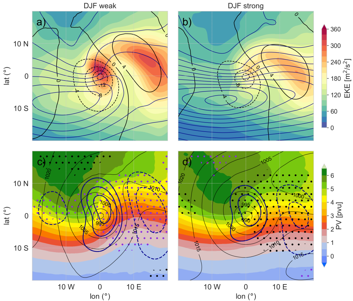
Figure 9. Cyclone-centered composites of cyclones at their time step of maximal 12-h intensification in the NP domain. Shown are cyclones with maximal intensification during time steps belonging to the weak (a,c) and strong U (b,d) terciles. (a,b) show the 300 hPa EKE in shading, the high-pass filtered SLP in black contours (every 4 hPa) and the total kinetic energy at 250 hPa in blue contours (every 200 \text{ m}^2 \text{ s}^{-2} ). The innermost total kinetic energy contour is 1400 \text{ m}^2 \text{ s}^{-2} in (a) and 2200 \text{ m}^2 \text{ s}^{-2} in (b). (c,d) show PV on 320 K in shading, SLP in black contours (every 5 hPa), and the high-pass filtered meridional wind at 300 hPa in blue contours (every 5 \text{ m s}^{-1} ). The significance of a positive (negative) PV anomaly with respect to the PV distribution of all DJF cyclones on a 1% level is shown by black (violet) stippling.
