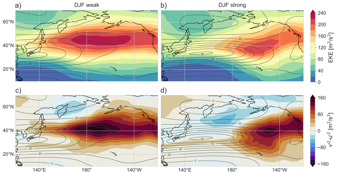
Figure 8. (a,b) EKE at 300 hPa (shading) and 10-d low-pass filtered zonal wind at 250 hPa ( U , gray contours, every 10 \text{ m s}^{-1} ) in the NP. (c,d) Eddy orientation measure, v'^2 - u'^2 (shading) and the 10-d low-pass filtered zonal wind on 250 hPa ( U , gray contours). (a,c) are for the weak jet composite and (b,d) for the strong jet composite.
