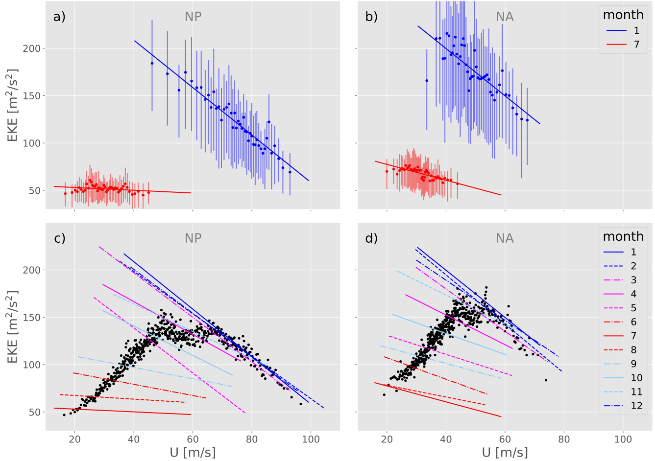
Figure 4. (a,b) Regression lines of instantaneous January (blue) and July (red) 10-d low-pass filtered maximum zonal wind at 250 hPa ( U ) and spatially averaged EKE at 300 hPa in the NP and NA domains, respectively. The data points represent averages and inter-quartile ranges of bins with similar values of U as in Fig. 2c,d but for the two months individually. (c,d) Regression lines as in (a,b) for all months separately superimposed on binned averages from Fig. 2c,d. Shown are results for the NP (a,c) and NA (b,d) for the years 1980-2023. The respective U and EKE domains in the western basins are specified in Sect. 2.2.
