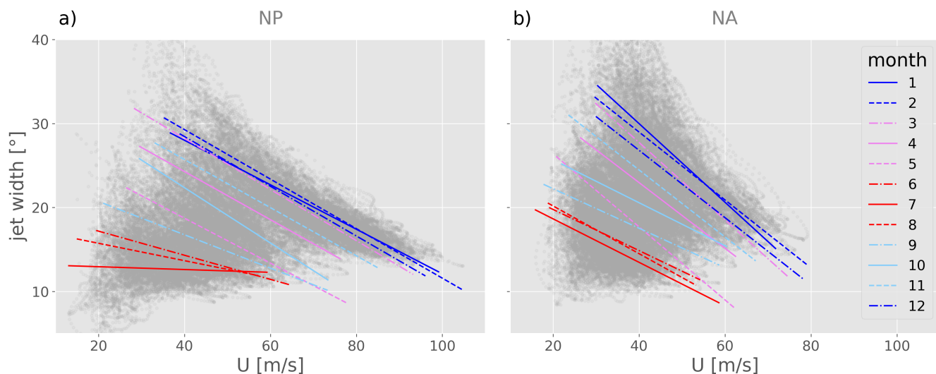
Figure 6. The instantaneous relationship between low-pass filtered zonal wind on 250 hPa, U , and the jet width shown as a scatterplot (gray dots) in (a) the NP and (b) the NA. Regression lines of the data points belonging to the individual months are shown in colour.
