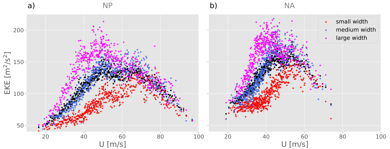
Figure 7. Monthly mean values of EKE versus U in (a) the NP and (b) the NA. Binned averages from Fig. 2 are shown in black. Averages over terciles of different jet width for each U -bin are shown in red (narrow jet), blue (medium jet) and purple (broad jet).
