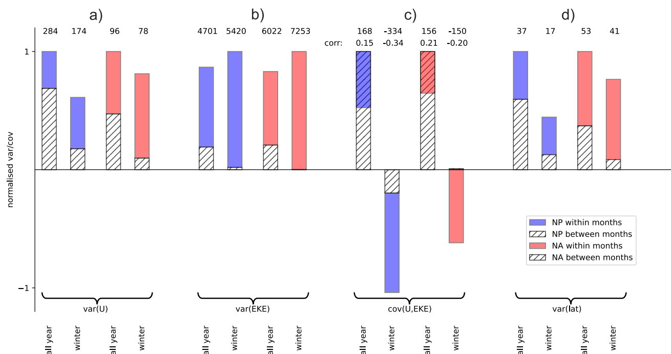
Figure 5. Variance of the maximum zonal 10-d low-pass filtered zonal wind at 250 hPa ( U ) and the averaged EKE at 300 hPa, computed over the NP and NA domains as specified in Sect. 2.2. Also shown are the variance of the latitude of the U maximum and the covariance between U and EKE. Variances and covariances are calculated for the entire year and the extended winter months (NDJFM) in the NP (blue) and NA (red). Bars are normalized by the total annual variance of the respective basin. The hatched portion represents the between-month variance and the coloured portion (blue for NP, red for NA) represents the within-month variance. Absolute total variances and covariances are given in the first row, while the second row specifies the correlation associated with the covariances.
