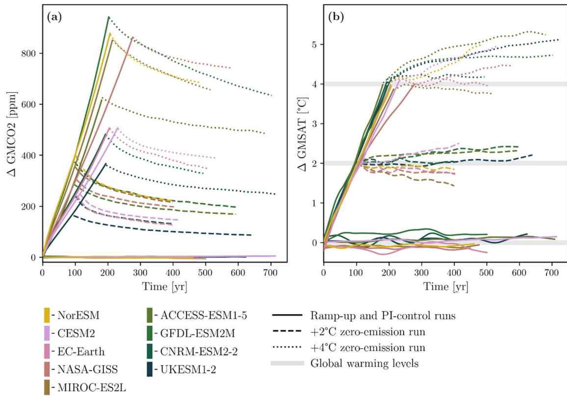
Figure 3: Global mean atmospheric CO 2 (atm.CO 2 in ppm, left panel) and GMSAT (°C, right panel) for the piControl (full line), ramp-up (full line) and zero-emission runs at GWL = 2 °C (dashed lines) and 4 °C (dotted lines), as simulated by nine ESMs (listed in the figure legend).
