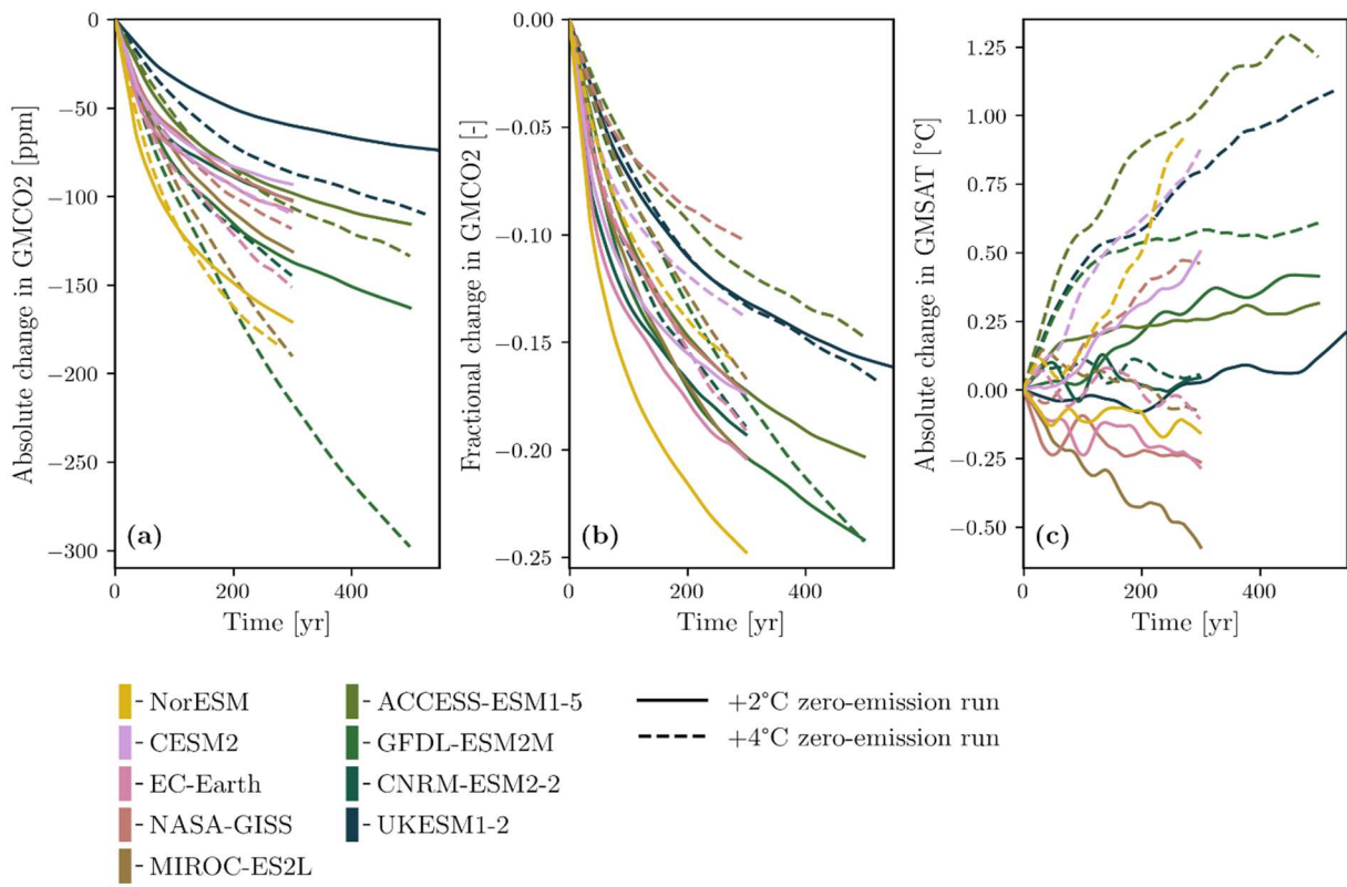
Figure 4: Change in global mean atmospheric CO 2 concentration and GMSAT for the two zero-emission runs expressed as anomalies relative to each value at the start of the respective zero-emission run. Left panel: absolute change in atm.CO 2 in ppm, middle panel: fractional change in atm.CO 2 , and right panel: change in GMSAT in °C.
