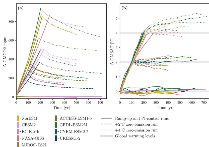
810 Figure 3: Global mean atmospheric CO 2 (atm.CO 2 in ppm, left panel) and GMSAT (°C, right panel) for the piControl (full line), 815 ramp-up (full line) and zero-emission runs at GWL = 2 °C (dashed lines) and 4 °C (dotted lines), as simulated by nine ESMs (listed in the figure legend).
