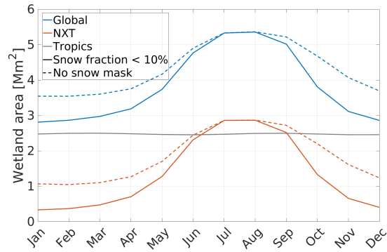
Figure 2. Wetland area yearly-annual cycle for the “Base” experiment. Solid lines only include cells with less than 10% snow whereas dashed lines includes all cells. Blue lines are global values, reddish include only the NXT area (north of 30°N) and the gray line is the “tropics” (everything south of 30°N). For the tropical area, snow masking does not make any difference.
