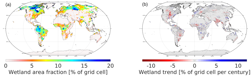
Figure 1. “Base” average distribution of (a) wetland area (% of grid cell area) in northern hemisphere summer (JJA) and (b) 1855-2014 wetland area trend of yearly-annual means (% of grid cell per century). Black dots mark cells with trends significant at the 95% level according to Matlab’s fitlm-fitlm function.
