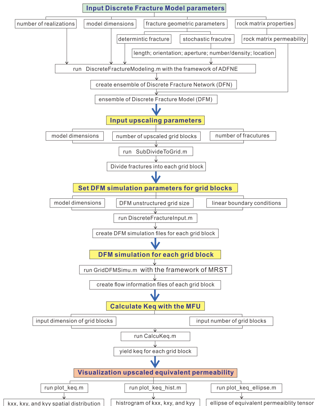
Figure 2: Workflow of the software UpsFrac.
