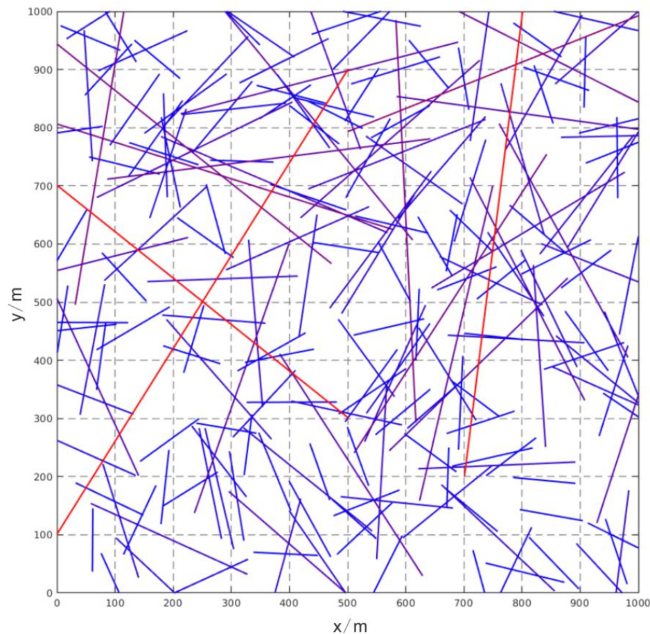
Figure 6: Discrete fracture model generated by UpsFrac. Blue denotes a low aperture, red denotes a high aperture, and the dashed line denotes the grid blocks on a coarse scale.
