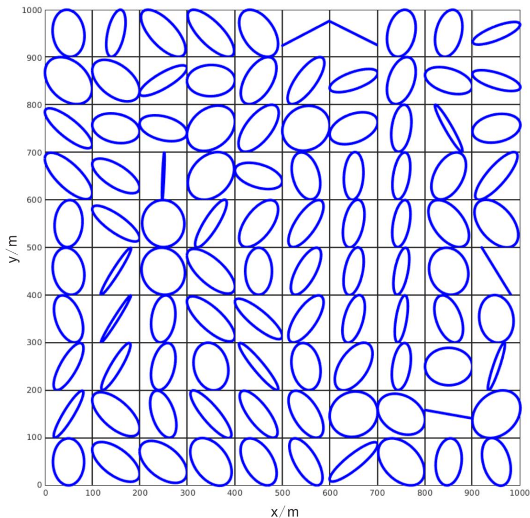
Figure 9: Ellipse of equivalent permeability tensor for the model.
