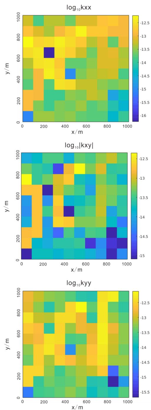
Figure 7: Equivalent permeability distribution of grid blocks on a coarse scale.
