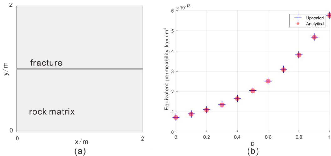
Figure 5: Comparison of upscaled and analytical equivalent permeability for varied aperture models.
