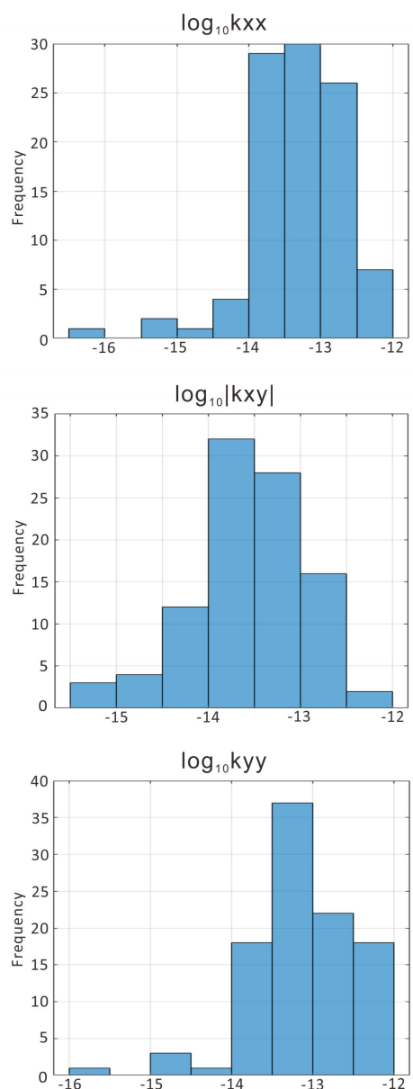
Figure 8: Histograms of upscaled equivalent permeability components.
