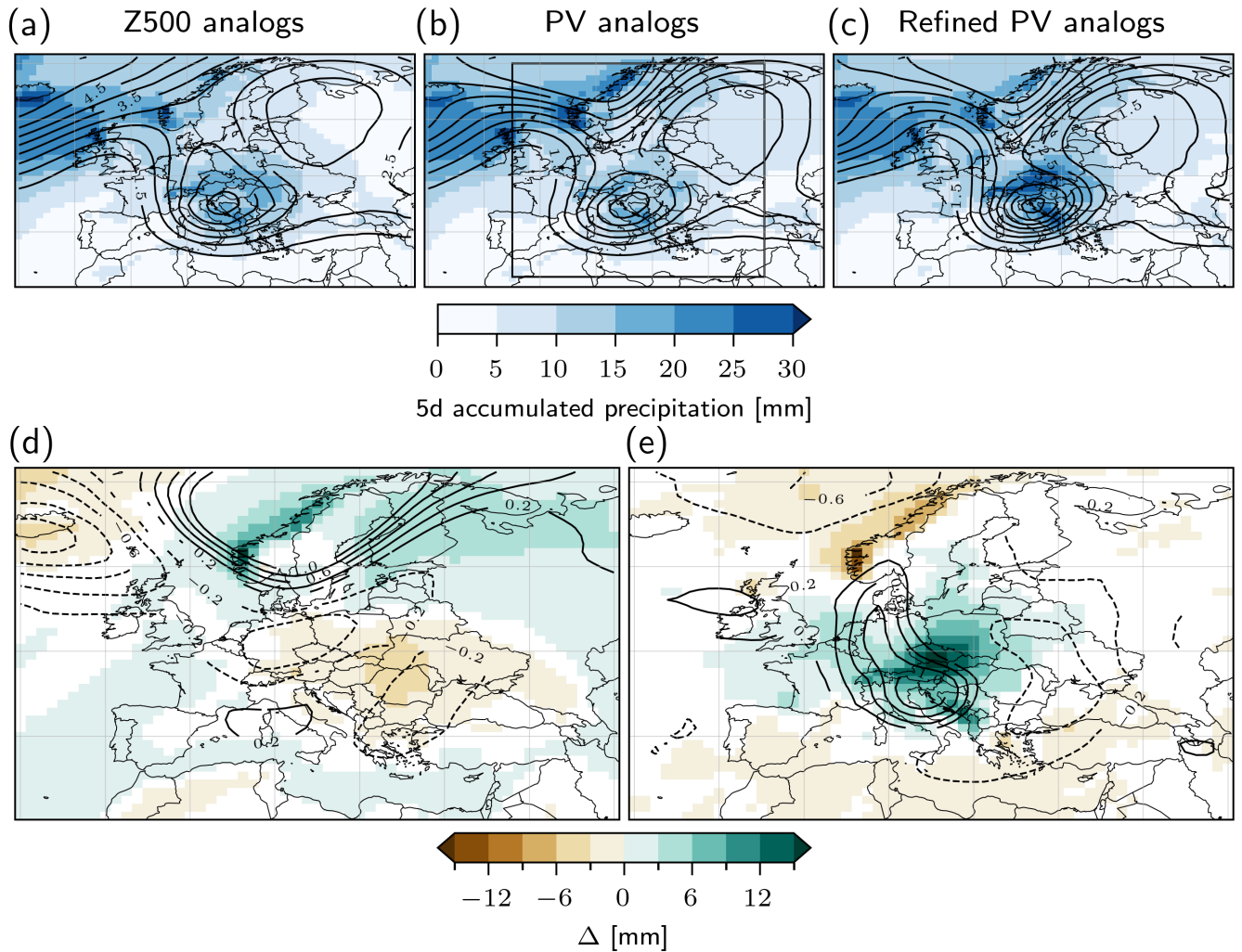
Figure 5. Composite mean of PV and precipitation for analogs selected using the Z500 fields, the 250hPa PV fields and the refined PV analogs. Mean 5-day accumulated precipitation (colors) and 250hPa PV (contours) for (a) the Z500 analogs ( n = 1050 ), (b) all the PV analogs ( n = 1050 ) and (c) the refined PV analogs ( n = 210 ). All analogs are found in the period 1990–1999 restricted to the August, September, October months (seasonal analogs). The PV contours are drawn every 0.5 PVU. Difference between (d) Z500 and all PV analogs (panel b - panel a) and (e) all PV analogs and refined PV analogs (panel c - panel b). Grid points with no significant differences (see text) are marked as white for the precipitation field and not shown for the PV field.
