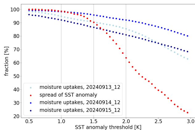
Fig. R2.4: Fraction of moisture uptakes (blue dots) over the Mediterranean and Black Sea occurring over a region with an SST anomaly above a certain threshold for moisture sources calculated for precipitation at 12 UTC on 13, 14 and 15 September 2024. The fraction of the Mediterranean and Black Sea region experiencing a mean SST anomaly from 5 to 11 September above a certain threshold is shown in red dots.
