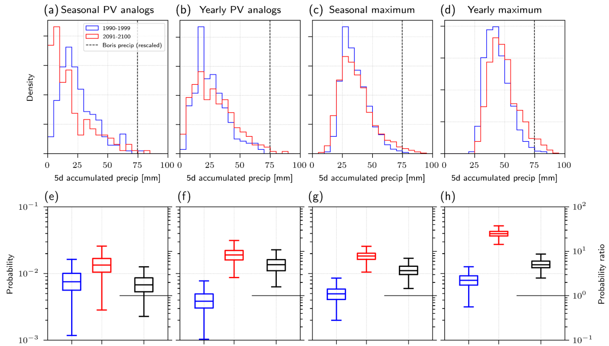
Fig. R2.1 (replacing Fig. 7 in the manuscript): Distribution of mean precipitation in the impacted region ( 47.2^{\circ} - 51^{\circ} N and 12^{\circ} - 19.5^{\circ} E) for Boris-like events defined as analogs events (two left columns) and as maximum precipitation events (two right columns). Distribution of spatial mean 5-day accumulated precipitation over the impacted region for the (a) seasonal and (b) yearly PV analogs and the maximum (c) seasonal and (d) yearly events in the periods 1990--1999 (blue) and 2091--2100 (red). The corresponding precipitation in ERA5 (after rescaling via quantile mapping to the present CESM1 distribution) for the Storm Boris over the same region is shown with a vertical dashed line. Probability to reach the rescaled ERA5 precipitation over the impacted region for the (e) seasonal and (f) yearly PV analogs and the maximum (g) seasonal and (h) yearly events in the periods 1990--1999 (blue) and 2091--2100 (red). Probabilities are estimated using a Gamma distribution for PV analogs and a GEV distribution for maximum events. The boxplots show the distribution of estimated probabilities over bootstrapped samples (see the manuscript for more details). The black boxplots show the corresponding distribution of probability ratios.
