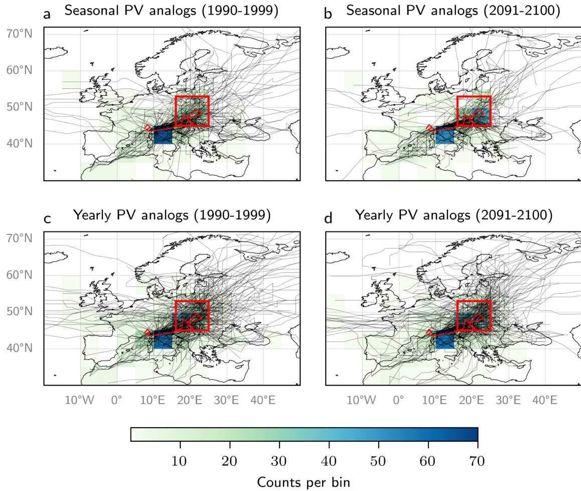
Fig. R1.2: Tracks of selected cyclones for the (a,b) seasonal and (c,d) yearly PV analogs in the CESM1 simulation in the periods (a,c) 1990–1999 and (b,d) 2091–2100. All tracks must be located within the red box at the analog time step. The red track indicates the track of storm Boris. Color shading indicates the number of cyclone track starting points within 5deg x 5deg bins.
