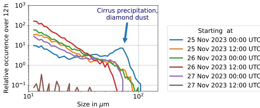
Figure 6. Temporal evolution of the particle size distributions integrated over 12 hours during the ice fog event of 25 November 2023. The particle mode with a modal maximum at particle sizes of 70 \mu\text{m} is observed only during the measurement period starting at 00:00 UTC on 25 November 2023, when streaks of ice particles were falling from high altitudes. For all 12-hour periods during the ice fog event the peak of the measured particle size distribution is at the lower size detection limit of PPD-2K at a spherical equivalent diameter of 11 \mu\text{m} . The last particle size distribution of 27 November 2023 12:00 UTC shows a low concentration at all bins, when no particles were seen on the lidar.
