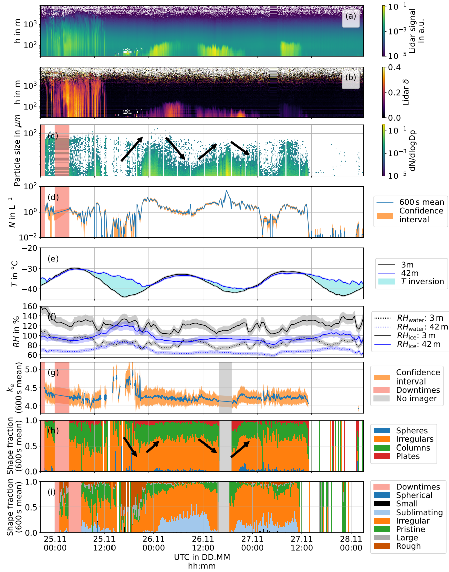
Figure 5. Temporal evolution of the ice fog event of 25 November 2023 with lidar backscattering signal in a.u. for the height h in m (a) ; and lidar backscattering linear depolarisation \delta (b) for the height h in m (b) , particle size distribution (c) and mean particle concentration ( N ) over 600 s (d) . Instrument downtimes are shaded in red. (e) shows the temperature ( T ) measured at heights of 3 m and 42 m above ground is shown in °C. Temperature inversions are highlighted. (f) shows the relative humidity with respect to ice and to liquid water ( RH_{ice} , RH_{water} ) at heights of 3 m and 42 m. (g) shows the 600 s rolling mean ice particle small-scale optical complexity parameter k_e (Vochezer et al., 2016). (h) and (i) show the particle shape fractions derived from the PPD-2K Fourier diffraction pattern analysis and machine learning diffraction pattern analysis, respectively. Arrows highlight the particle growth and sublimation periods with corresponding changes in the fraction of pristine ice crystals.
