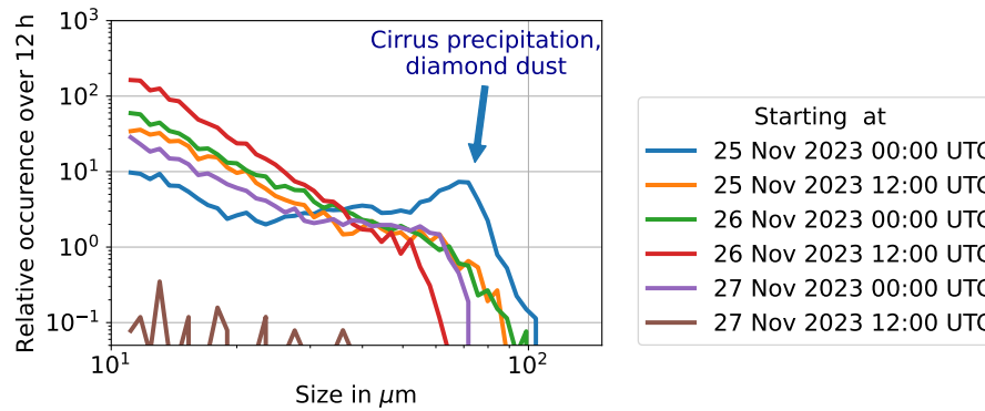
Figure 6. Temporal evolution of the particle size distributions integrated over 12 hours during the ice fog event of 25 November 2023. The particle mode with a modal maximum at particle sizes of 70 \mu\text{m} is observed only during the measurement period starting at 00:00 UTC on 25 November 2023, when streaks of ice particles were falling from high altitudes. For all 12-hour periods during the ice fog event the peak of the measured particle size distribution is at the lower size detection limit of PPD-2K at a spherical equivalent diameter of 11 \mu\text{m} . The last particle size distribution of 27 November 2023 12:00 UTC shows a low concentration at all bins, when no particles were seen on the lidar.
