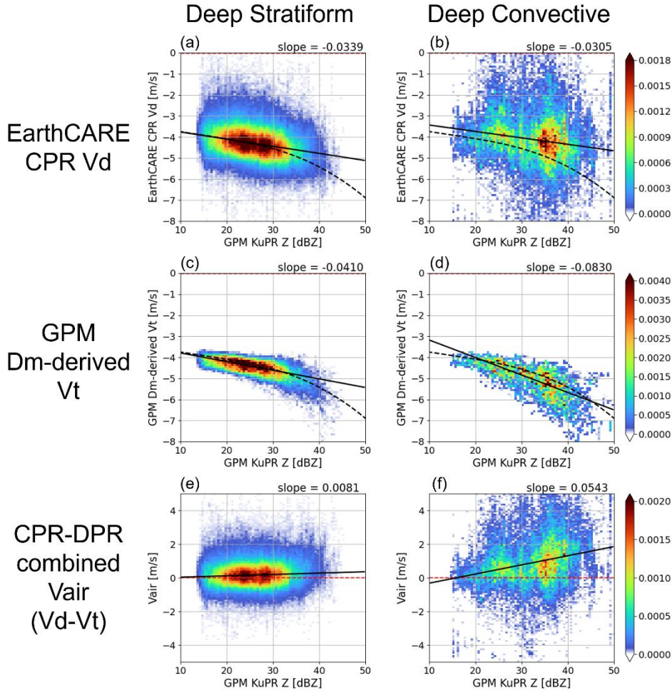
Figure 10: Joint histograms for the temperature above 4°C as a function of Z_{Ku} . The vertical axes represent (a, b) V_d measured by CPR, (c, d) V_t and (e, f) V_{air} calculated using the 2A.DPR product. (a, c, e) deep stratiform and (b, d, f) deep convective types. Each histogram is normalized by the total number of samples of each precipitation type. The solid black lines represent regression lines fitted using the least squares method, with its corresponding slope indicated in the upper right corner outside each panel. The dashed black lines in (a–d) are same as those in Fig. 5.
