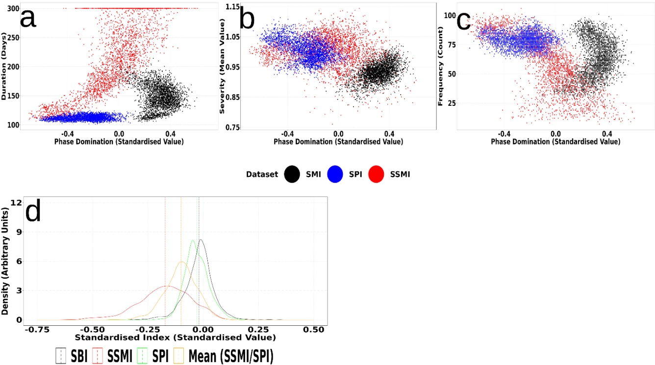
Figure 7: Duration (a), severity (b) and frequency (c) (y axis), mapped against phase domination (common x axis), represented by the mean metric value at each grid cell. Note the difference x and y scales within and between plots. Plots are for the bivariate (SBI) and consecutive (SPI; SSMI) classification techniques. Also included are density plots (d), showing the distribution (SPI, SSMI and mean of both (SPI and SSMI)) during seesaw events defined by the bivariate approach (SBI), with vertical dotted lines representing mean values.
