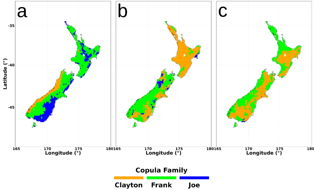
Figure 2: Spatial comparison of the optimal copula family for the pair copulas: Precipitation-Soil Moisture (a); Precipitation-Temperature (b) and Temperature-Soil Moisture, given Precipitation (c). Optimal family was determined using AIC for the period 1 January 1950 to 31 December 2021 and covering the entirety of New Zealand.
