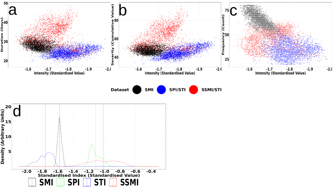
270 Figure 3: Duration (a), severity (b) and frequency (c) (y axis), mapped against intensity (common x axis), represented by the mean metric value at each grid cell. Note the different x and y scales within and between plots. Plots are for the multivariate (SMI) and coincident (SPI and STI; SSMI and STI) classification techniques. Also included are density plots (d), showing the distribution (SPI, SSMI and STI) during hot and dry conditions defined by the multivariate approach (SMI), with vertical dotted lines representing mean values.
