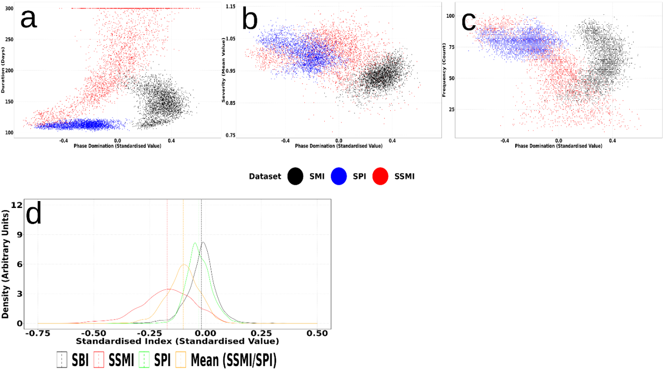
340 Figure 6: Duration (a), severity (b) and frequency (c) (y axis), mapped against phase domination (common x axis), represented by the mean metric value at each grid cell. Note the difference x and y scales within and between plots. Plots are for the bivariate (SBI) and consecutive (SPI; SSMI) classification techniques. Also included are density plots (d), showing the distribution (SPI, SSMI and mean of both (SPI and SSMI)) during seesaw events defined by the bivariate approach (SBI), with vertical dotted lines representing mean values.
