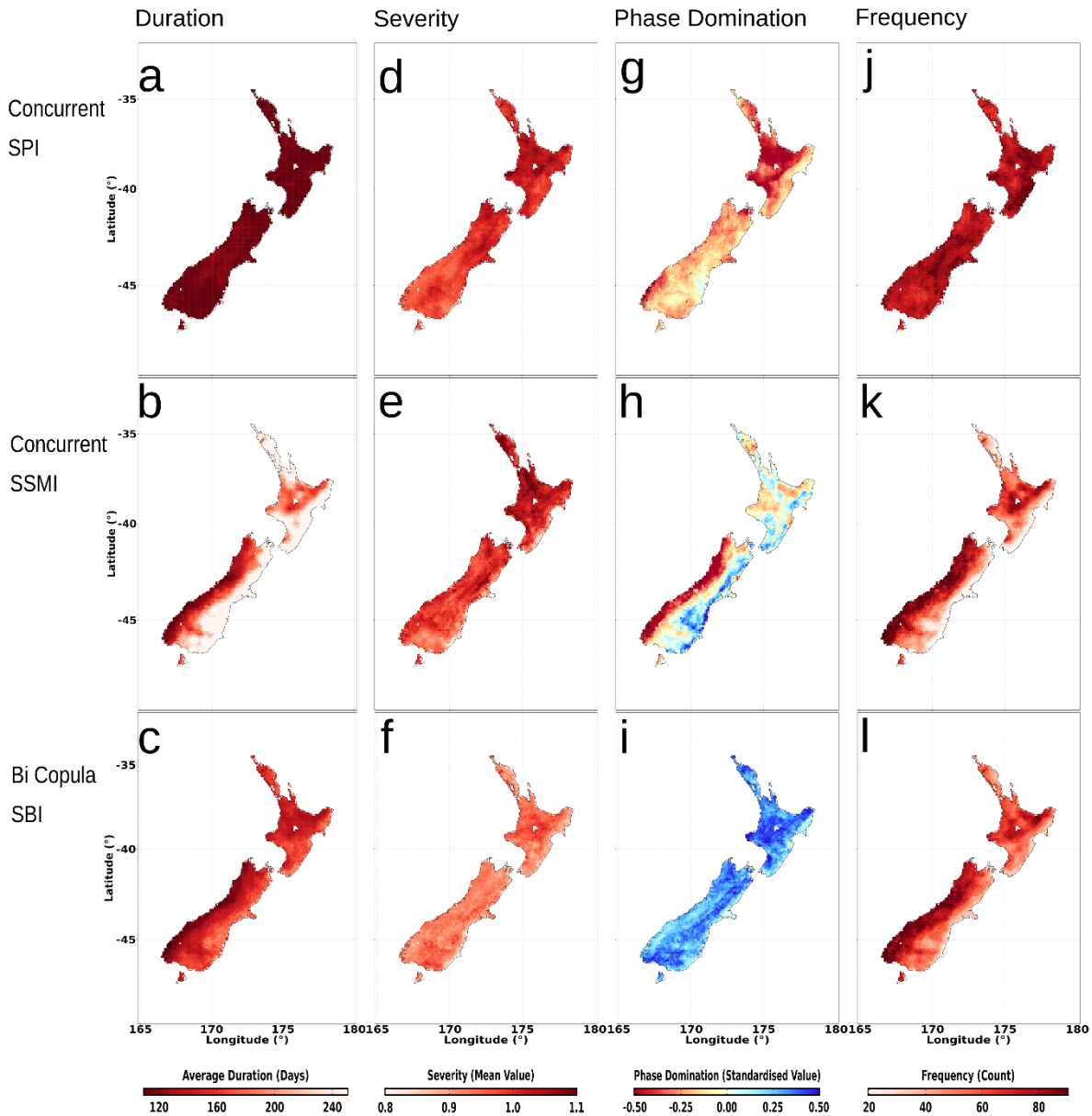
Figure 7: Average duration (a-c), severity (d-f), phase domination (g-i) and frequency (j-l) of seesaw events on a grid cell basis for the period 1950-2021. Showing the concurrent classifications of SPI (a, d, g, j) and SSMI (b, e, h, k), as well as the bivariate SBI (c, f, i, l). Note the differing scales.
