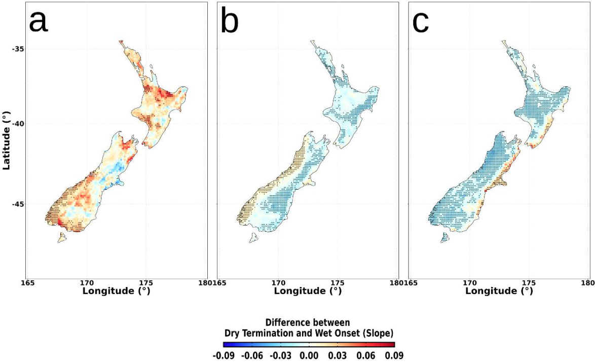
405 Figure 9: Differences in slope rates between dry termination and wet onset rates of seesaw events for the period 1 January 1950 to 31 December 2021 for SPI (a), SSMI (b) and SBI (c) classifications. Stippling indicates significance at the 5% level.
