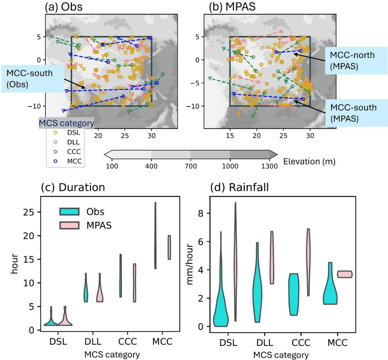
Figure 3. Initial (circles) and final (triangles) locations of each detected MCS during November 21–25, 2023, based on (a) observations and (b) MPAS-A simulations. The four categories of MCS are represented by different colors. Dashed lines indicate the connection between initial and final locations but do not represent the actual MCS tracks. Shading represents elevation (m). The MCC cases analyzed in this study are marked. Violin plots of (c) duration (hours) and (d) mean precipitation (from CMORPH; mm/hour) within the 219 K contours for each MCS category in observations and MPAS-A simulations. The width of the violin plot indicates probability distribution.
