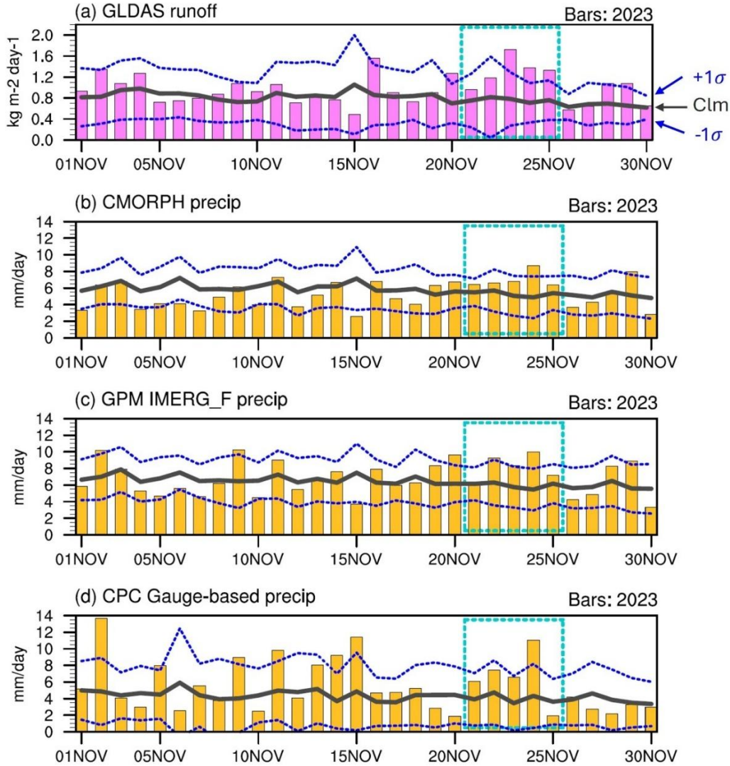
Figure 2. (a) Daily mean basin-averaged runoff (bars; kg/m 2 /day) from GLDAS for 2023 (bars), along with climatological mean (solid gray line) and the climatological mean \pm 1 standard deviation (dashed blue lines) for the period November 1–30. from November 01, 2023, to November 30, 2023, overlaid by climatological runoff (gray line) during November. The period analyzed in this study is within the turquoise box. (b–d) Same as (a), but for precipitation (mm/day) from three observational datasets. The climatological period for each dataset corresponds to its available data range, as detailed in Section 2.1.
