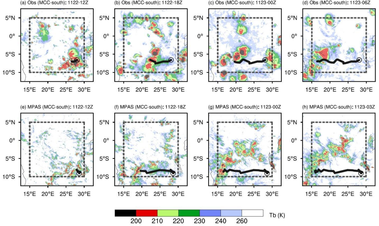
Figure 4. (a–d) MCC-south tracking of Tb (K) every 6 hours (in UTC) from NCEP/CPC data in observations. The black line represents the MCC track, and the open circle denotes its initiation location. (e–h) Same as (a–d), but for MPAS-A simulations. Note that the MCC-south in MPAS-A simulations ends at 03:00 UTC on November 23.
