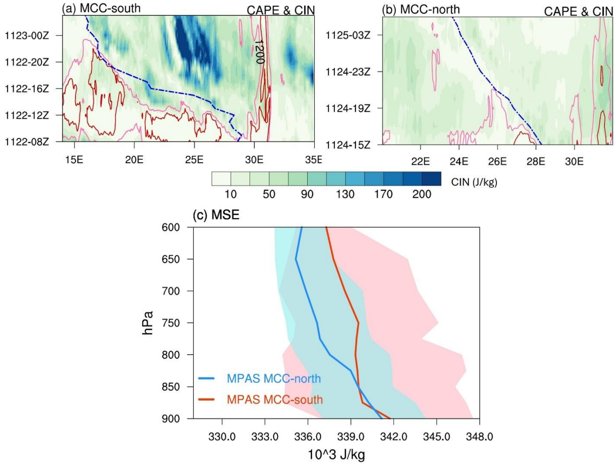
Figure 7. (a) Hovmöller diagram for 8^{\circ}\text{S} – 9^{\circ}\text{S} averaged CAPE (contours; J/kg; the light and dark red contours represent 1200 J/kg and 2000 J/kg, respectively) and CIN (shading; J/kg) for MCC-south from MPAS-A simulations. The blue dashed line represents the MCC track. (b) Same as (a), but for 1.5^{\circ}\text{N} – 2.5^{\circ}\text{N} averaged fields for MCC-north. (c) The mean MSE ( 10^3 J/kg) for all timesteps along the track of MCC-north (blue line) and MCC-south (red line) from MPAS-A simulations. Shading represents the spread of the minimum and maximum values of MSE for all timesteps along the track.
