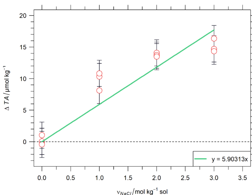
Figure 1: Quantification of background alkalinity coming-originating from the NaCl matrix for the artificial reference material. Where \Delta TA represents the difference of total alkalinity between the measured one and the theoretical value calculated with Eq. 4. Red circles represent single TA potentiometric measurements with error bars representing their standard uncertainty, and green straight line represents the slope obtained from linear regression passing through the origin.
