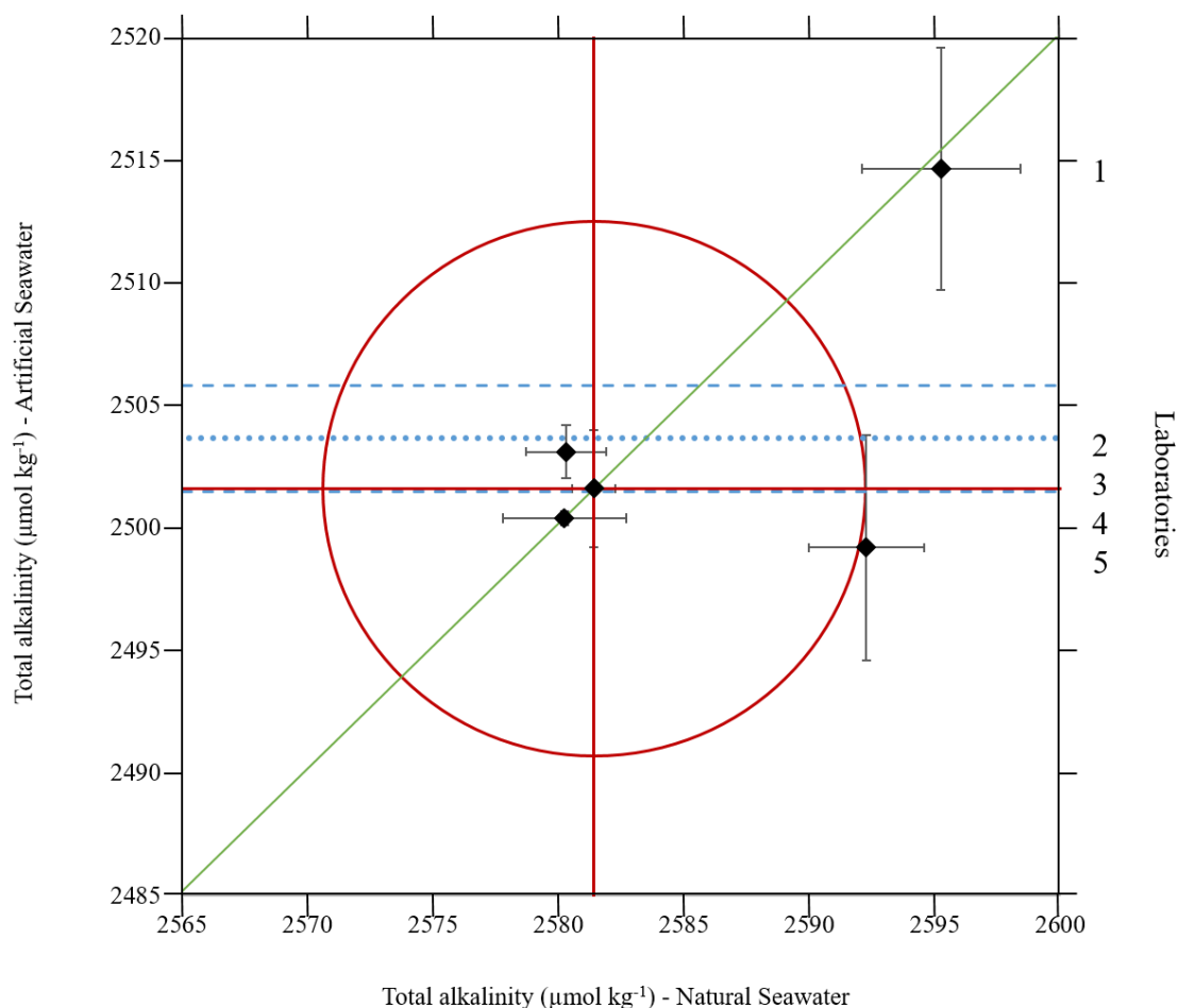
Figure 4: Youden plot of the inter-laboratory comparison conducted on the Stabilized natural seawater (X-axis) and the Artificial seawater, Batch 1 (Y-axis). Where d Diamonds correspond to the data point (X_i, Y_i) of each participant, green straight line corresponds to the 45^\circ line graphical marker, the two straight red horizontal and vertical lines represent the median of total alkalinity results obtained from the five laboratories on the artificial solution and the stabilized natural seawater, respectively, and the red circle represents the 95% confidence level circle. The blue dotted line represents the artificial reference material reference value together with its expanded uncertainty in blue dashed lines.
