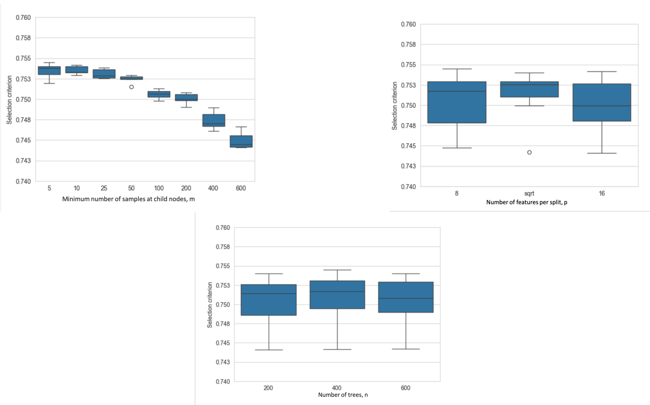
Figure 4. Hyperparameters optimization results for QRF-national. The selection criterion is the median hyperparameter criterion across the catchments of the study.
