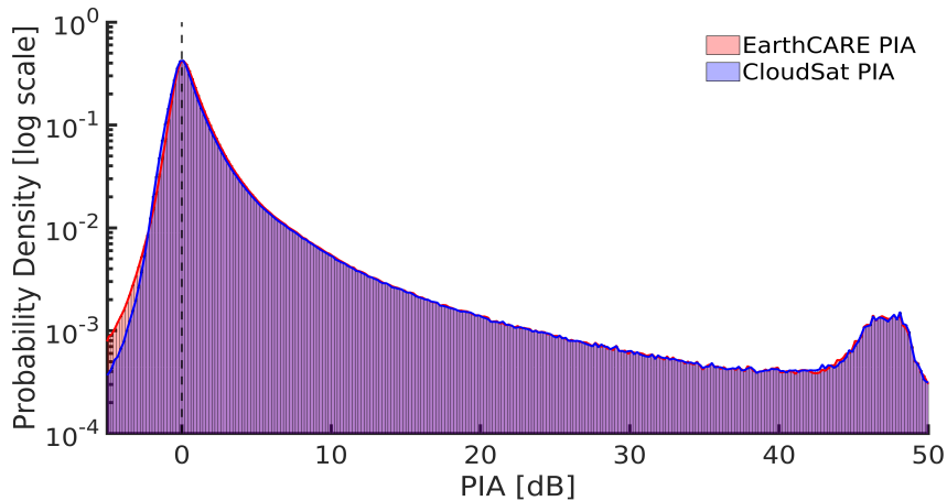
Figure 13. The global probability distributions of PIA estimates obtained from the EarthCARE retrieval methodology applied to CloudSat observations (January–April 2007) and from the PIA from CloudSat retrievals are compared on a logarithmic scale. The overlapping distributions demonstrate strong consistency in the statistical characteristics of the two retrieval approaches, supporting the robustness of the EarthCARE method when applied to CloudSat data.
