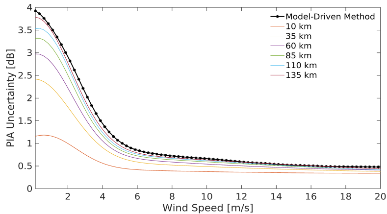
Figure 1. Comparison of PIA uncertainty from the model-driven method (Eq. 5) and the clear-sky interpolation method using 'N' calibration points (Eq. 9), shown as a function of wind speed at cloudy profile and for different calibration-point distances.
