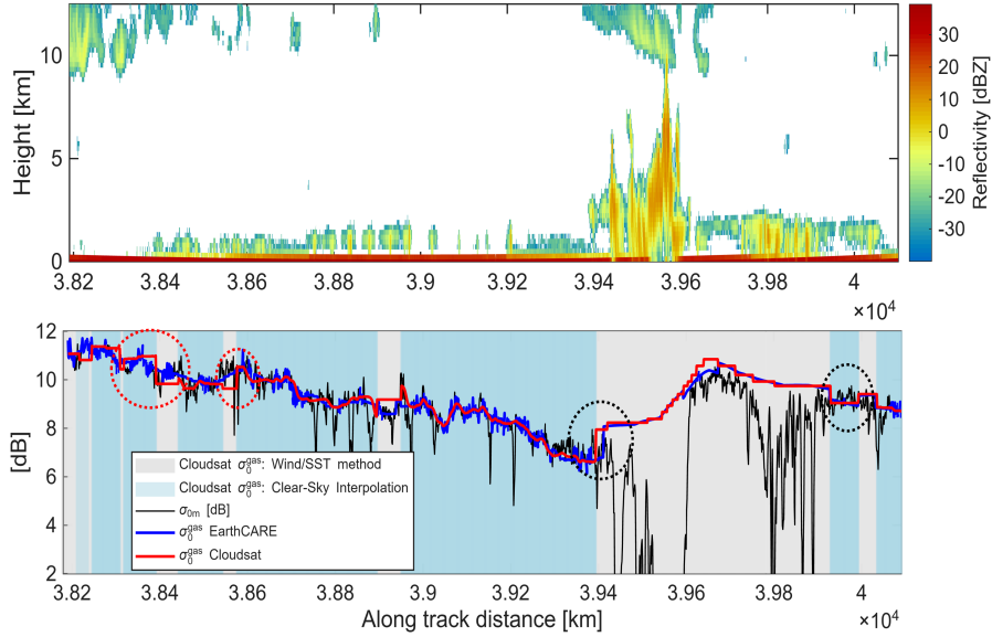
Figure 12. CloudSat Case Study. Top panel: vertical reflectivity profile as a function of along-track distance. Bottom panel: measured normalized radar cross section (NRCS, \sigma_{0m} , black curve), along with the estimated clear-sky NRCS ( \sigma_0^{gas} ) within cloudy regions, derived using the proposed EarthCARE method (blue curve) and the CloudSat-based estimate (red curve). Red circles highlight jumps in the CloudSat \sigma_0^{gas} estimate, while black circles indicate jumps observed in both EarthCARE and CloudSat estimates. Gray and blue shading in the second panel indicate the two estimation methods used in the CloudSat methodology: the Wind/SST method, which utilizes a geophysical model, and the clear-sky interpolation method. Jumps in the CloudSat \sigma_0^{gas} generally occur when the method switches between these two approaches.
