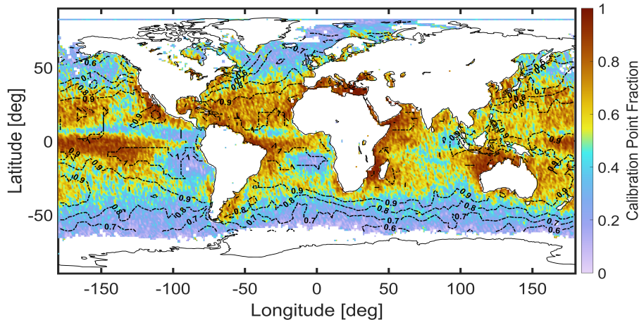
Figure 4. Global distribution of the calibration point fraction, defined as the ratio of calibration points to the total number of radar profiles within each 1^\circ \times 1^\circ grid cell based on 6 months of data (July to December 2024). A profile is considered a calibration point when it is classified as clear sky by the profile_class mask in the Level-2 C-PRO FMR product, or identified as ice-only cloud, and lies within a 10 km along-track segment that includes at least six profiles of the same class and exhibits a measured NRCS standard deviation below 0.3 dB. Black dashed contour lines indicate the fraction of profiles where the clear-sky interpolation method is applied, highlighting regions where this approach is frequently used for PIA estimation.
