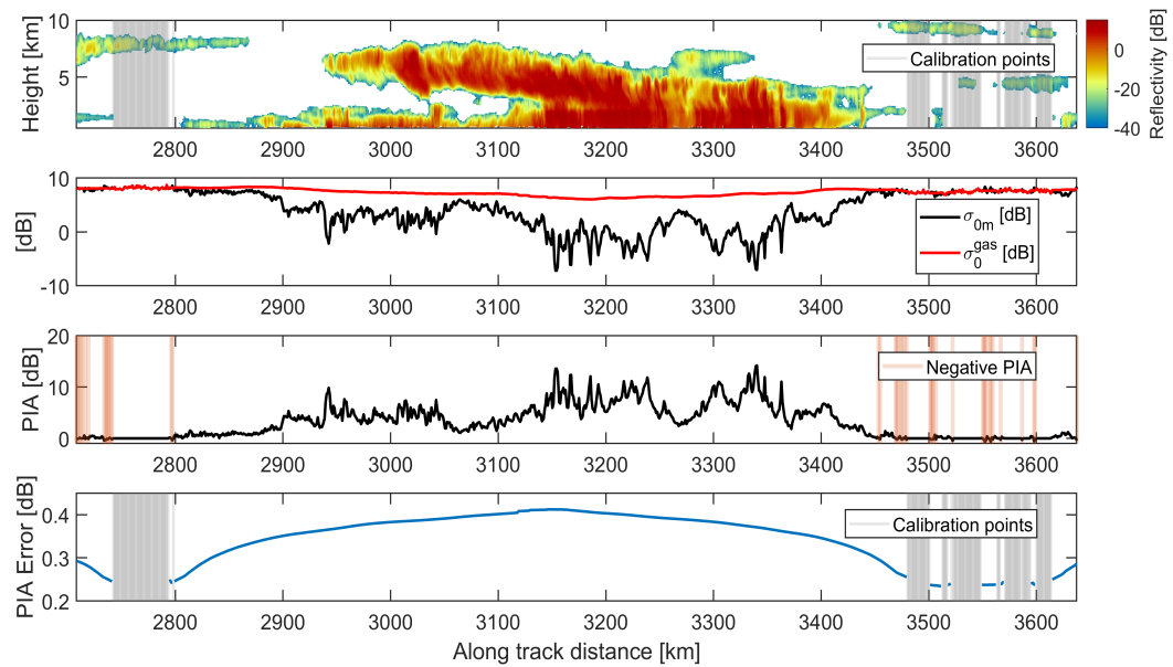
Figure 11. EarthCARE Case 3: same as Fig. 9 for a stratiform cloud observed over the southeastern Atlantic Ocean near the west coast of Africa.
