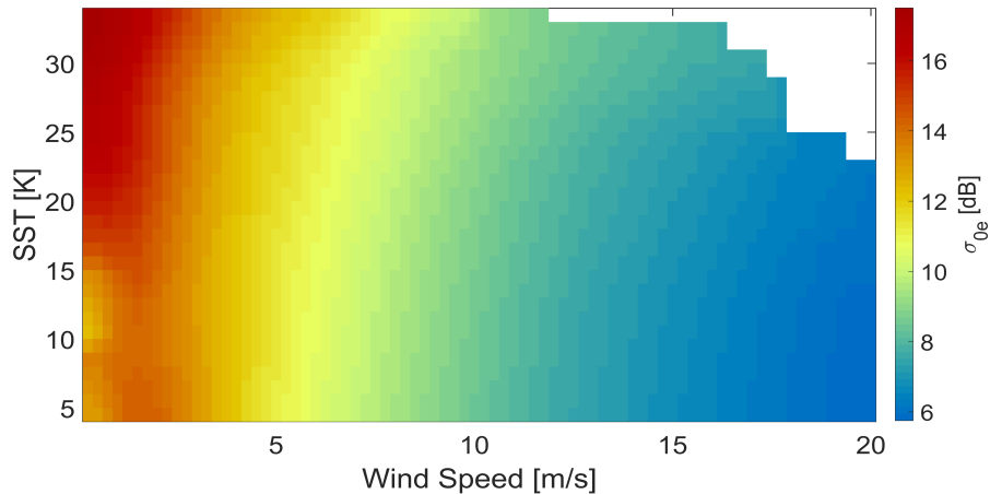
Figure 8. Look-up table of the effective surface backscattering cross section ( \sigma_{0e} ) derived from EarthCARE measurements collected between June 2024 and June 2025, shown as a function of sea surface temperature (SST) and wind speed. The table is constructed by averaging clear-sky NRCS observations corrected for gaseous attenuation within discrete SST and wind speed bins. Results indicate that \sigma_{0e} exhibits significantly greater variability with respect to wind speed than SST.
