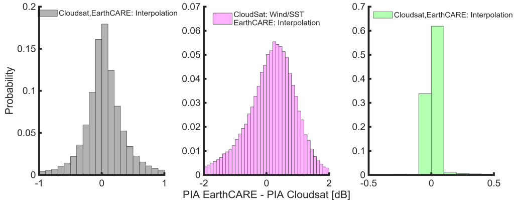
Figure 14. Probability distributions of the differences between PIA estimates from the EarthCARE and CloudSat methodologies based on four months of profiles identified as cloudy by the 2B-GEOPROF CloudSat product. The gray histogram shows cases where both CloudSat and EarthCARE use the clear-sky interpolation method, with a narrow distribution centered near 0 dB. The purple histogram corresponds to profiles where CloudSat uses the wind/SST method and EarthCARE applies clear-sky interpolation, exhibiting a broader distribution with a peak around 0.3–0.5 dB. The green histogram represents cases where both EarthCARE and CloudSat use the wind/SST method, with a distribution centered at 0 dB.
