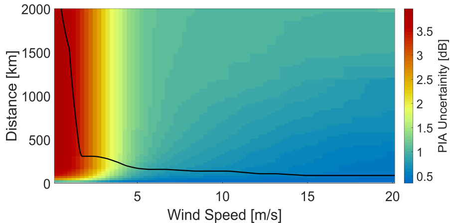
Figure 2. Lookup table of two-way PIA uncertainty associated with the clear-sky interpolation method, shown as a function of wind speed at the cloudy profile and distance to the calibration points. The uncertainty is derived using an ensemble of clear-sky oceanic profiles over the June 2024–June 2025 period. For each profile location x , the NRCS is estimated using all other clear-sky profiles as calibration points. The difference between the estimated and measured NRCS at x defines the residual. These residuals are then binned by wind speed and distance to the calibration points, and the uncertainty in each bin is quantified as the standard deviation of the residuals as in Eq. (9). The solid black contour delineates the transition boundary beyond which the model-driven method, Eq. (5), yields lower PIA uncertainty compared to the clear-sky interpolation approach.
