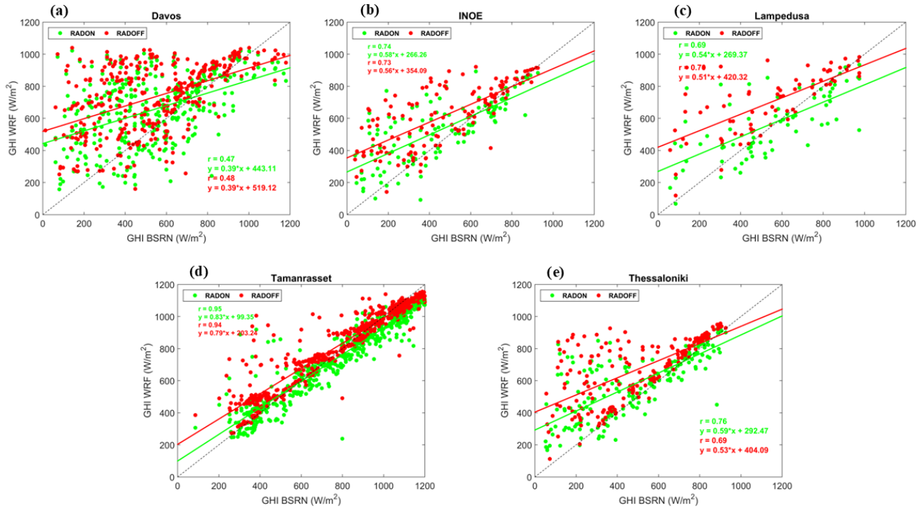
385 Figure 5 Correlation between the GHI from the pyranometer and the model for RADOFF (red) and RADON (green) for the five sites under all sky conditions for DOD>0.05.
