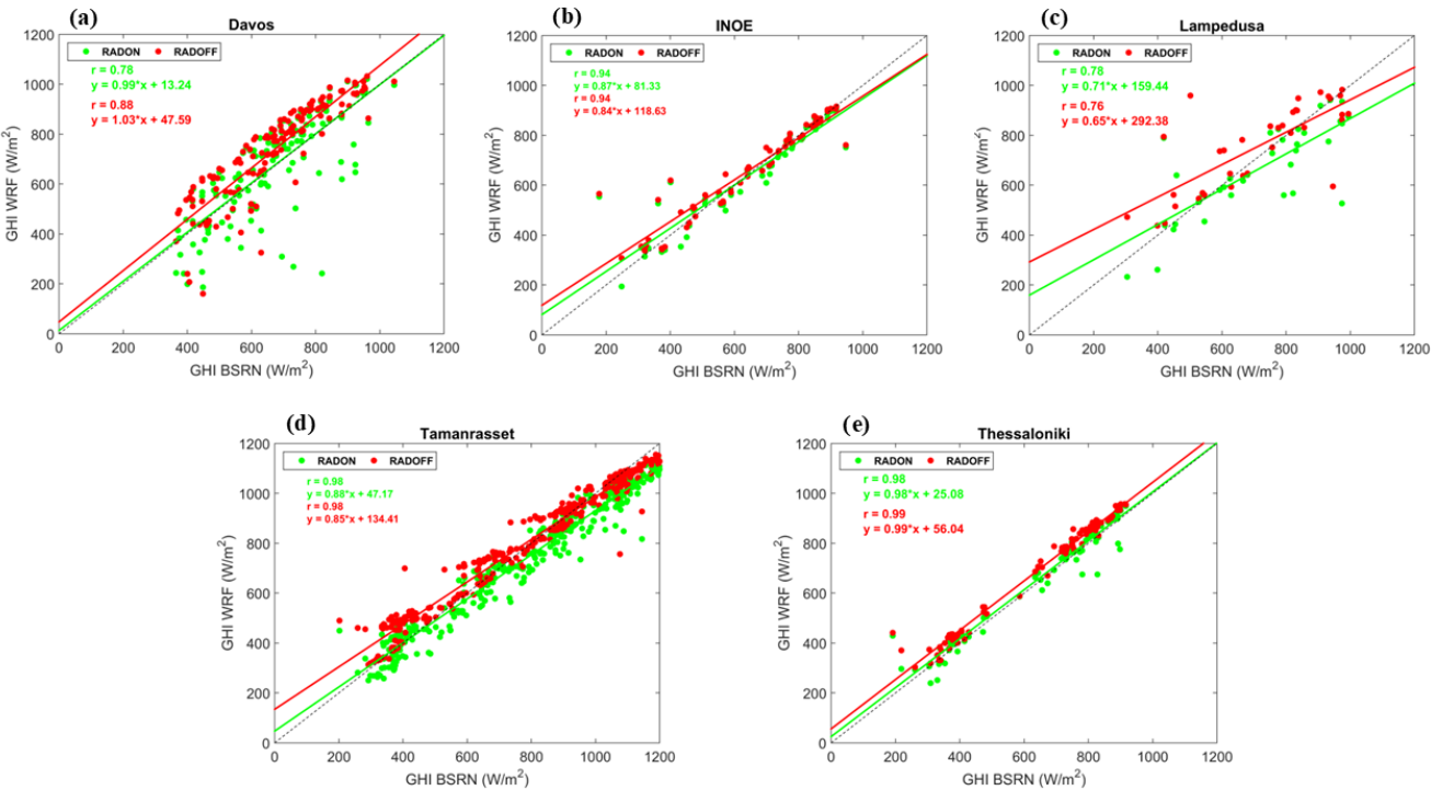
320 Figure 4 Correlation between the GHI from the pyranometer and the model for RADOFF (red) and RADON (green) for the five sites under clear-sky conditions
