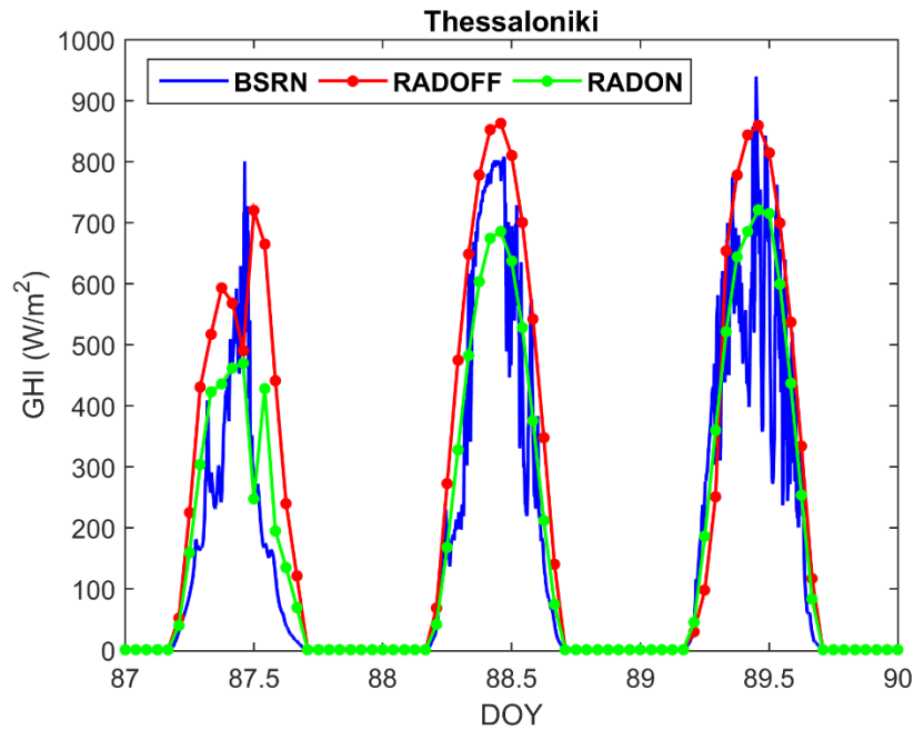
Figure 7 GHI from BSRN and the model for cloudy days in Thessaloniki.
