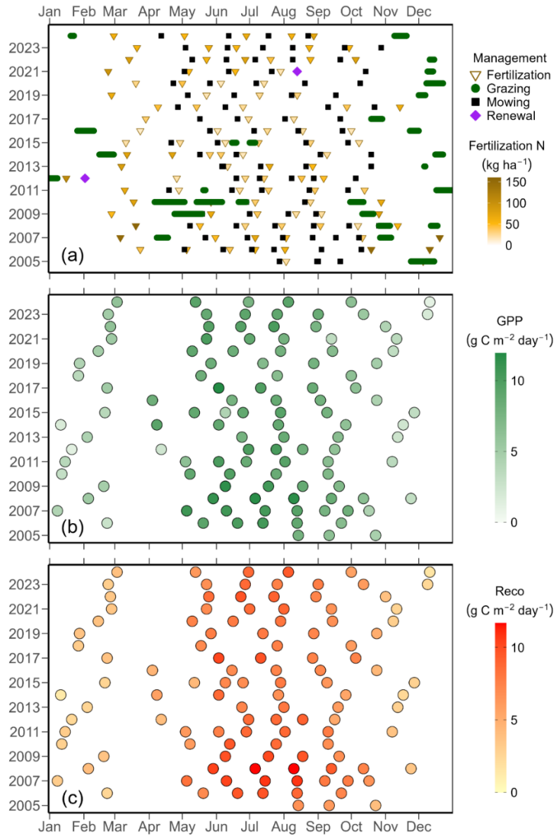
Figure 3. Management events (a) and CO 2 fluxes (b-c) during regrowth periods. (a) Major management events at the Chamau grassland site between July 2005 and December 2024. The x-axis position of each point indicates the date of each event. Symbols
