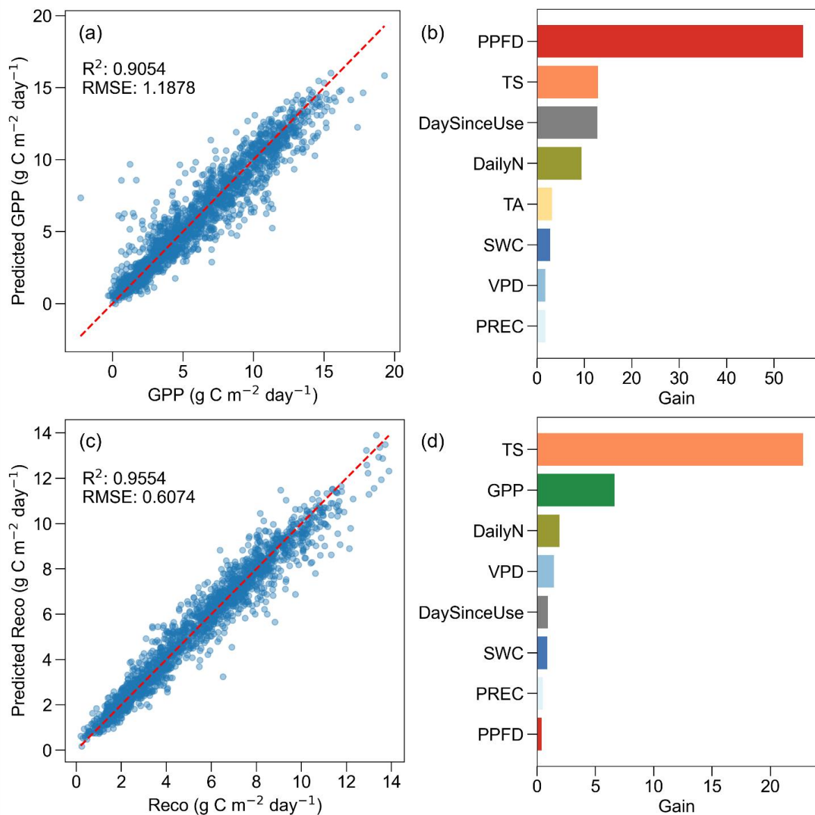
Figure A2. Performance and feature importance of XGBoost models for daily gross primary production (GPP) and ecosystem respiration (Reco). (a) Predicted versus actual GPP with model coefficient of determination (R 2 ) and root mean square error (RMSE) for the testing set, (b) feature importance (gain) for the GPP model, (c) predicted versus actual Reco with model R 2 and RMSE for the testing set, and (d) feature importance (gain) for the Reco model. In panels (a) and (c), red dashed lines represent 1:1 lines. In panels (b) and (d), higher gain values indicate higher importance of the features on model predictions. Features have the same colour code as in Fig. 4: photosynthetic photon flux density (PPFD, red), soil temperature (TS, orange), air temperature (TA, yellow), soil water content (SWC, dark blue), vapour pressure deficit (VPD, blue), precipitation (PREC, light blue), day since last mowing, grazing or renewal (DaySinceUse, grey), daily fertilizer nitrogen input (DailyN, moss green), and gross primary production (GPP, green).
