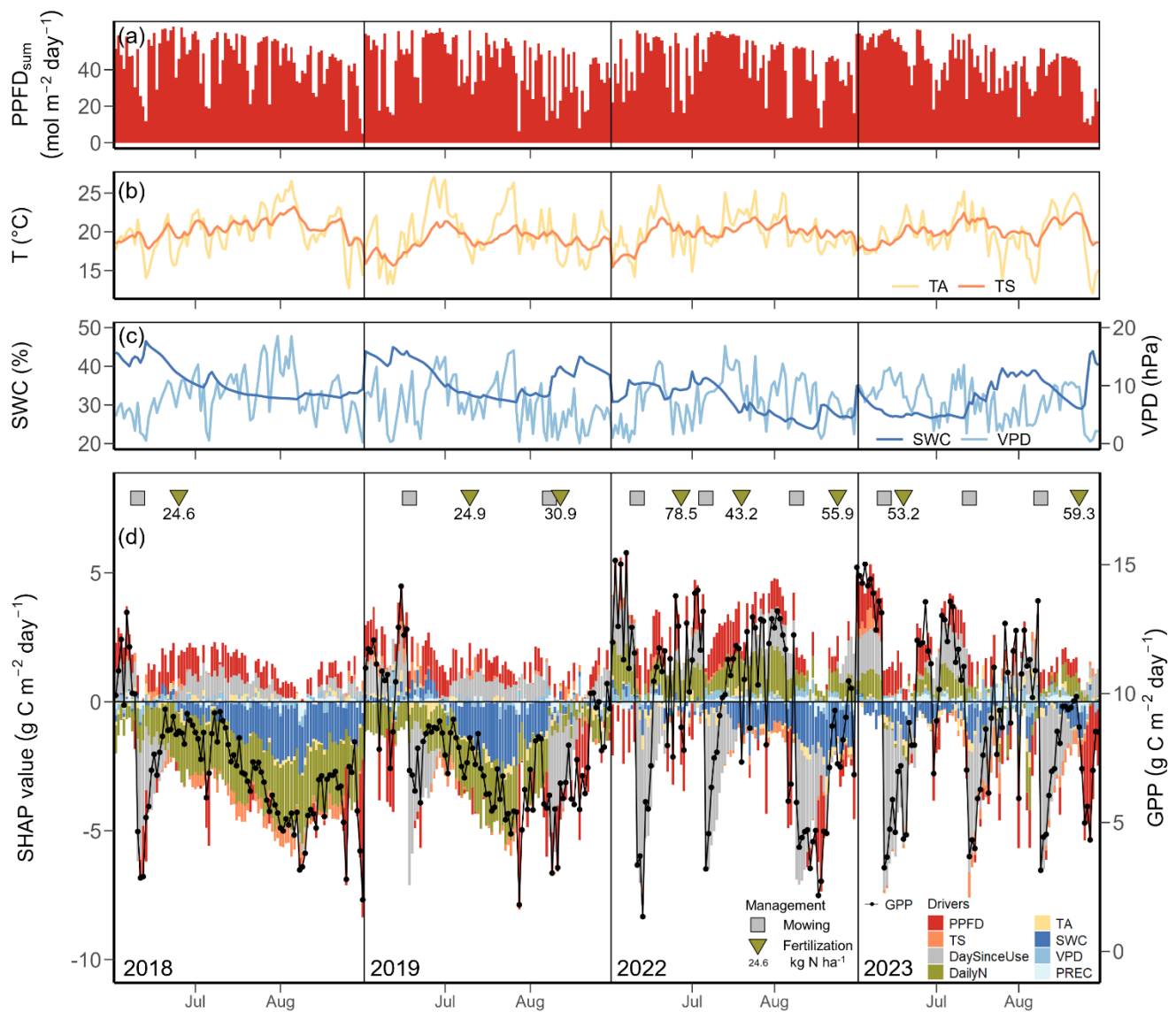
Figure 6. Meteorological conditions and drivers of gross primary production (GPP) for days in the peak growing seasons (June, July, August) during the extreme years 2018, 2019, 2022 and 2023 from SHAP analysis 2. (a) Daily total photosynthetic photon flux density (PPFD sum ), (b) daily mean air temperature (TA, yellow line) and soil temperature (TS, orange line), (c) daily mean volumetric soil water content (SWC, dark blue line) and vapour pressure deficit (VPD, light blue line), (d) daily GPP (black dot-line) and SHAP values of each driver (stacked bar) are given. Colours of the bars represent different drivers: photosynthetic photon flux density (PPFD, red), soil temperature (TS, orange), air temperature (TA, yellow), soil water content (SWC, dark blue), vapour pressure deficit (VPD, blue), precipitation (PREC, light blue), day since last mowing, grazing or renewal (DaySinceUse, grey), and daily fertilizer nitrogen input (DailyN, moss green). The mean prediction of GPP during non-extreme months in peak growing seasons (June, July, August) at SHAP value zero corresponds to a GPP of 9.7 \text{ g C m}^{-2} \text{day}^{-1} . The years 2018 and 2019 were before the grassland renewal in 2021, the years 2022 and 2023 after the grassland renewal. Positive SHAP values represent positive effects of drivers on GPP relative to the mean prediction, while negative values indicate negative effects from the mean prediction. Symbols in the top of panel (d) represent management events during these months: mowing (squares) and fertilization (triangles). Numbers under the triangles give the amount of total fertilizer nitrogen (N) input. The x-axis position of each symbol indicates the date of each event.
