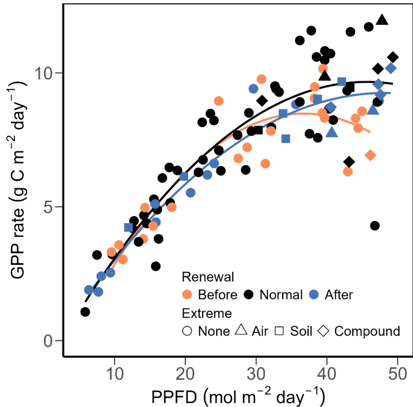
Figure 5. Relationships between mean photosynthetic photon flux density (PPFD) and gross primary production (GPP) during regrowth periods between 2005 and 2024, excluding the renewal years (2012 and 2021). Two years before the renewal years (i.e., 2010 and 2011; 2019 and 2020) are presented in orange; two years after the renewal years (2013 and 2014; 2022 and 2023) are shown in blue, while the remaining years are shown in black. Regrowth periods that spanned across extreme months (as shown in Fig. 2) are shown in different shapes: high air dryness (triangles), high soil dryness (squares), and compound air and soil dryness (diamonds). Second-degree polynomial fits are shown in solid lines, with the same colour code as for the years.
