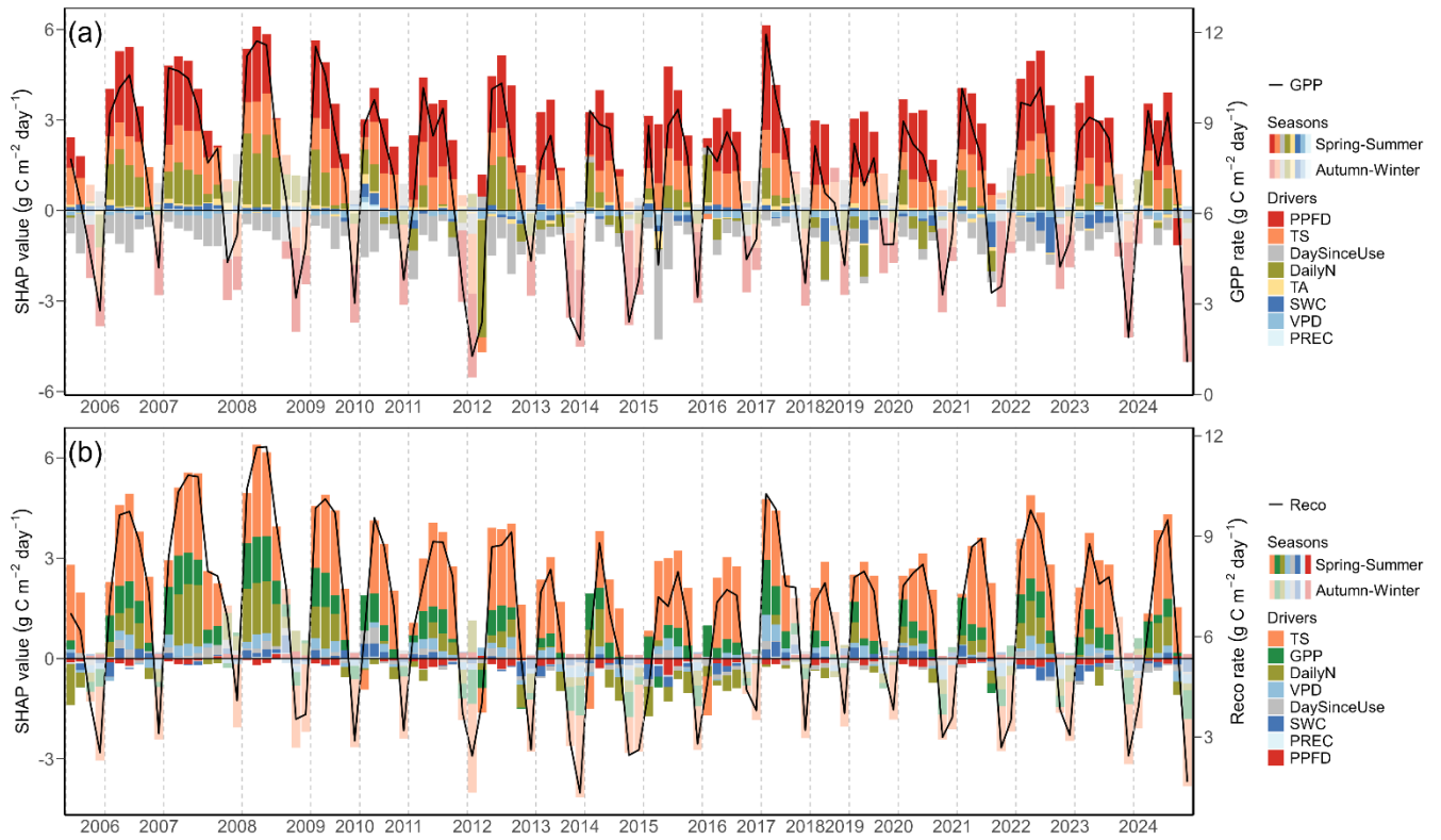
Figure 4. Drivers of (a) gross primary production (GPP) and (b) ecosystem respiration (Reco) for all regrowth periods during the years 2005 to 2024 from SHAP analysis 1. Each stacked bar represents mean SHAP values of drivers from the overall XGBoost model, presented for each regrowth period: total photosynthetic photon flux density (PPFD, red), soil temperature (TS, orange), air temperature (TA, yellow), volumetric soil water content (SWC, dark blue), vapour pressure deficit (VPD, blue), precipitation (PREC, light blue), daily fertilizer nitrogen input (DailyN, moss green), day since last mowing, grazing or renewal (DaySinceUse, grey), and gross primary production (GPP, green). The overall mean prediction for all years at SHAP value zero corresponds to a GPP of 6.1 \text{ g C m}^{-2} \text{ day}^{-1} and Reco of 5.3 \text{ g C m}^{-2} \text{ day}^{-1} . Positive SHAP values represent positive effects of drivers on GPP and Reco relative to the mean prediction, while negative values indicate negative effects from the mean prediction. GPP and Reco during each regrowth period are shown as black lines. Bars with full opaque colours indicate regrowth periods in the spring-summer season (April-September). Bars with more transparent colours indicate regrowth periods in the autumn-winter season (October-March).
