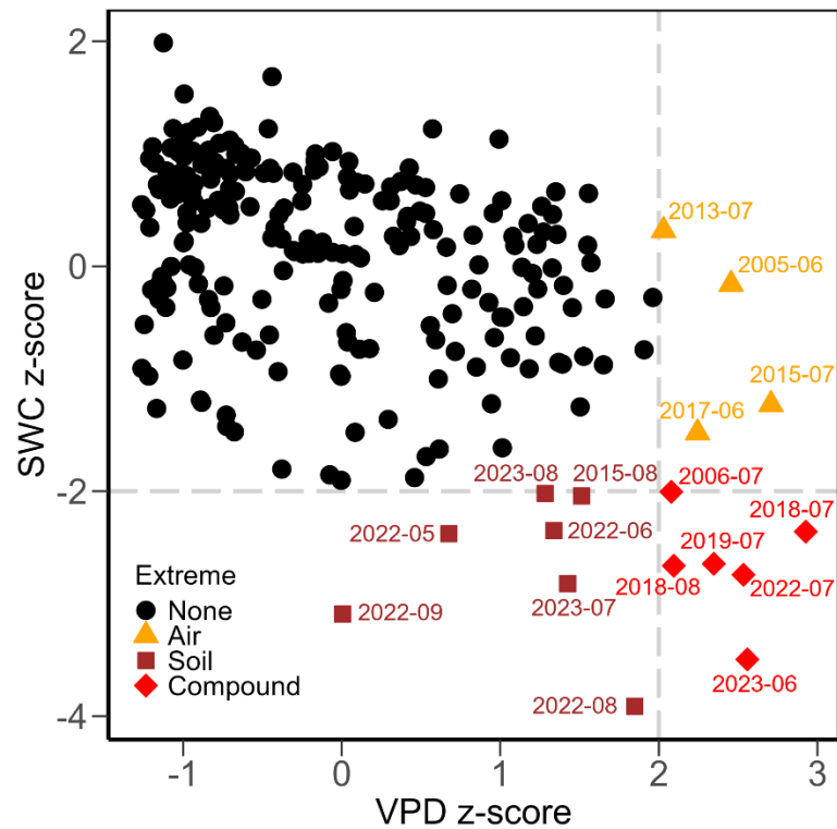
Figure 2. Z-scores for monthly mean vapour pressure deficit (VPD) and volumetric soil water content (SWC) from 2005 to 2024. Grey dashed lines indicate thresholds for extreme months (z-score of 2 for VPD and of -2 for SWC). Symbols and colours indicate types of extreme: none (black dots), high air dryness (orange triangles), high soil dryness (dark red squares), and compound air and soil dryness (red diamonds).
