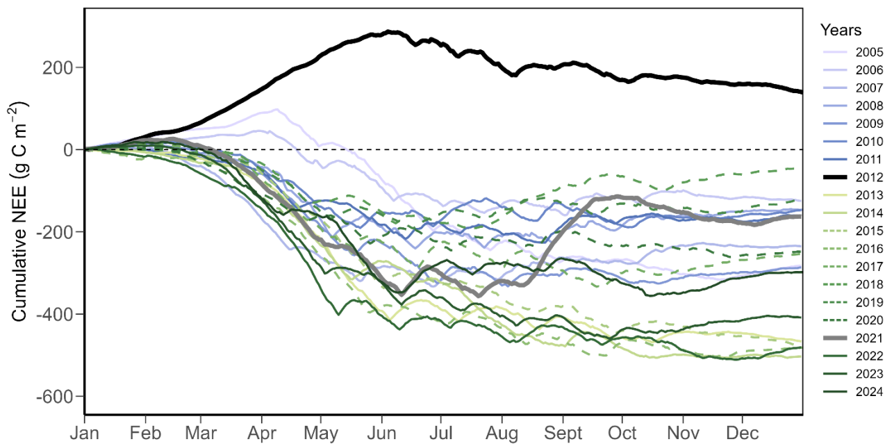
565 Figure A1. Annual cumulative sum of daily net ecosystem CO 2 exchange (NEE) for the years 2005 to 2024. Years during the N 2 O mitigation experiment (2015 to 2020; see Methods and Feigenwinter et al., 2023b) are shown with dashed lines, years with sward renewals (2012 and 2021) are shown in thicker black and grey lines, respectively.
