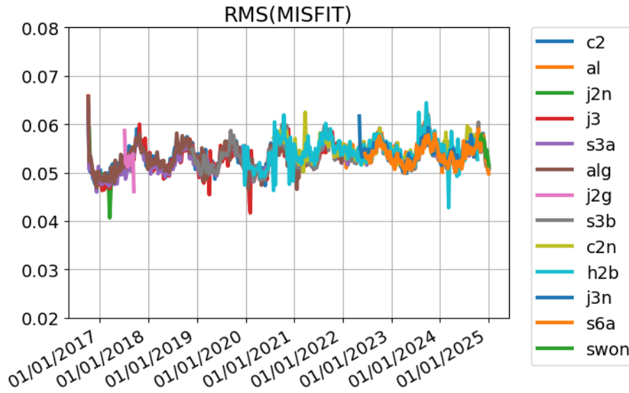
Figure 6: Temporal evolution of the global mean SLA innovation (observation – background model first trajectory) (top panel) and RMS of this misfit (below panel) for the different altimetry data sets assimilated in GLO12v4: c2 (Cryosat-2), al (Alti-Ka), j2n (Jason-2 tandem phase), j3 (Jason-3), s3a (Sentinel 3a), alg (Alti-Ka geodetic phase), j2g (Jason-2 geodetic phase), s3b (Sentinel 3b), c2n (Cryosat-2), h2b (Hy 2b), j3n (Jason-3 tandem phase), s6a (sentinel 6a), swon (Swot nadir). Units are meters.
