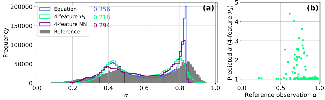
Figure 7. Comparison of the sea ice albedo distributions during the validation period (2019–2020) between the VIIRS product (Key et al., 2001, 2016) as reference observation and the predictions from the best-performing models in each model class in terms of MSE. Panel (a) illustrates the distribution of the reference observation alongside predictions from the best-performing equation (Eq. 4), the 4-feature polynomial of degree three P_3 , and the 4-feature neural network (NN), all within the physical range between 0 and 1. The Hellinger distance for each model is shown next to the legend in their respective colors. Panel (b) shows predicted albedo values falling outside the physical range for the polynomial of degree three with four features, plotted against the observed sea ice albedo.
