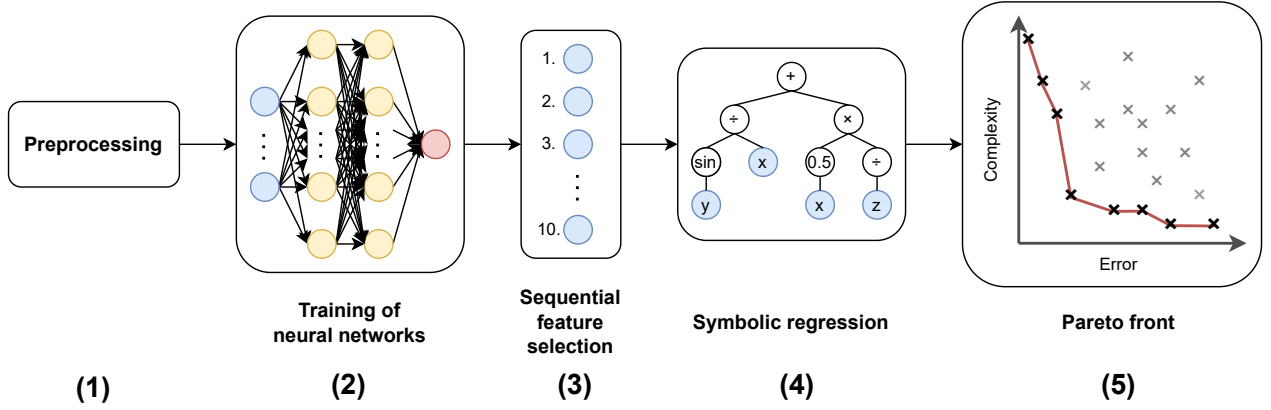
Figure 1. Pareto optimality-based workflow based on Beucler et al. (2025) and Grundner et al. (2024), exemplarily for discovering equations with symbolic regression. The process involves: (1) preprocessing of observational and reanalyses data to ensure consistency for the machine learning workflow, (2) training of multilayer perceptron neural networks (NNs), (3) sequential feature selection (SFS) for dimensionality reduction and identification of key features out of ten features governing sea ice albedo, (4) symbolic regression as data-driven equation discovery approach, and (5) comparison between the best-performing equations and baseline models (polynomials and NNs with reduced feature sets chosen by the SFS algorithm) on an error-complexity plane to evaluate how increasing model complexity reduces error.
