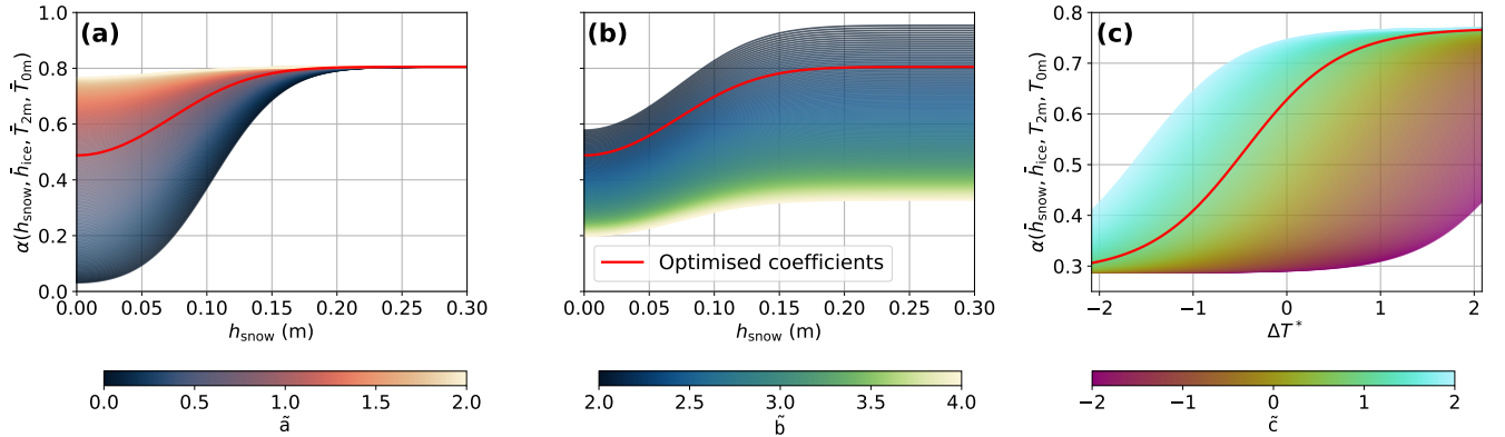
Figure 5. The impact of the coefficients \tilde{a} , \tilde{b} and \tilde{c} on the functional behaviour of Eq. 4. Panels (a) and (b) illustrate the dependency of sea ice albedo ( \alpha ) on snow depth ( h_{\text{snow}} ) with varying \tilde{a} and \tilde{b} , respectively. Panel (c) demonstrates the response on the difference between 2m temperature ( T_{2m} ) and surface temperature ( T_{0m} ) with varying \tilde{c} . The other coefficients are kept fixed at their optimal values and the other features at their mean values during the validation period (2019–2020) denoted with bar overhead (Table B1 in Appendix B). The red line indicates Eq. 4 with the optimised coefficient values (see Sec. 3.2).
