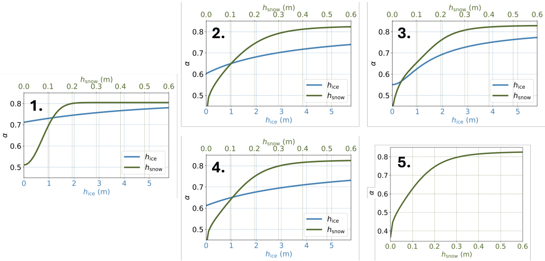
Figure C1. Comparison of the responses of the candidate equations to varying snow depth ( h_{\text{snow}} ) and sea ice thickness ( h_{\text{ice}} ), complementary to Fig. 3. Equation 1 equals Eq. 4 in the main text.
