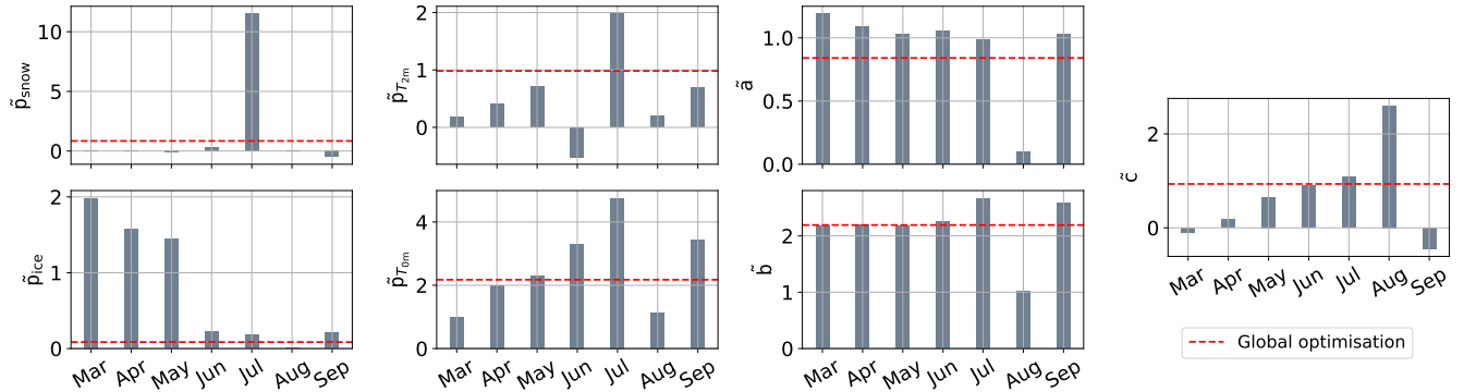
Figure H1. Monthly optimised coefficients of Eq. 4. The coefficients are unitless, meaning that they are rescaled by dividing by their standard deviations of the training set (2013–2018).
