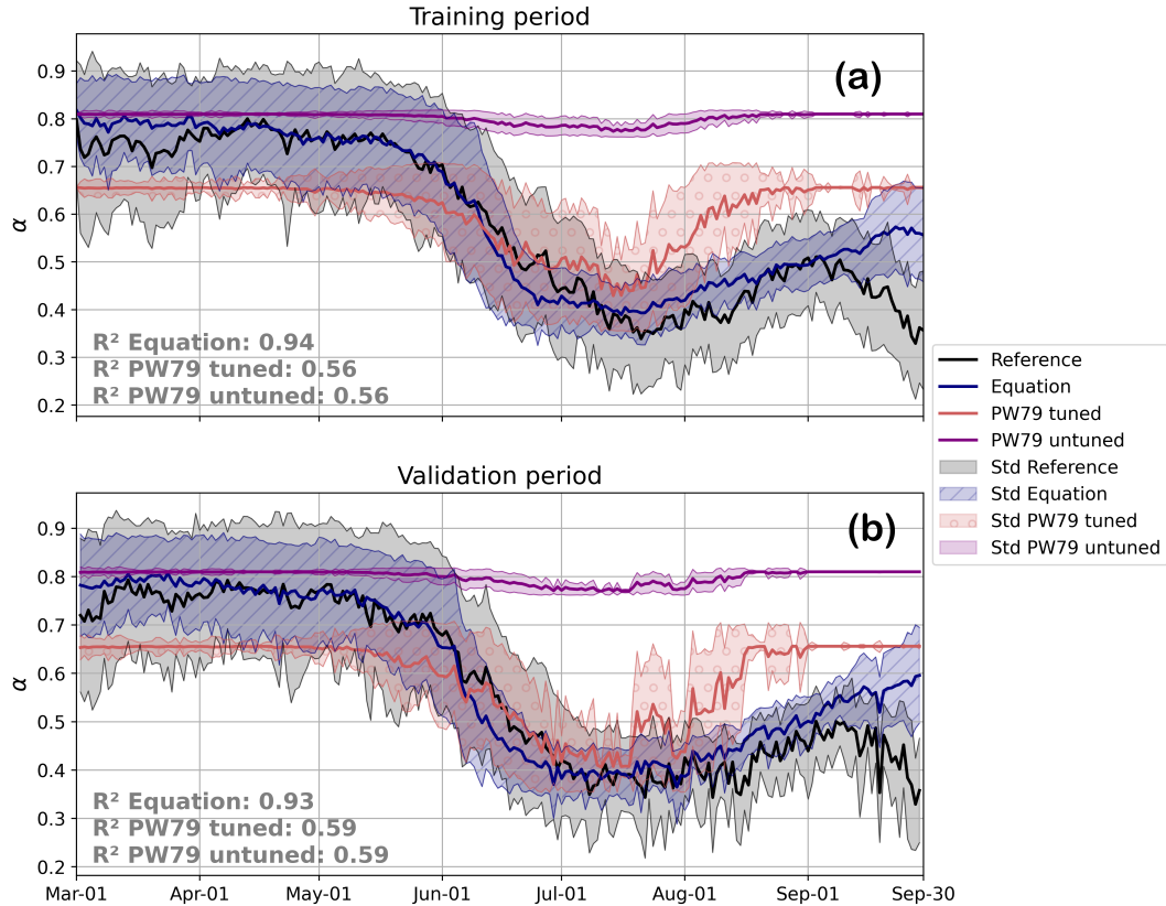
Figure F1. Seasonal cycle of albedo \alpha from March 1 to September 30 averaged (a) from 2013 until 2018 (training period) and (b) from 2019 until 2020 (validation period), complementary to Fig. 9.
