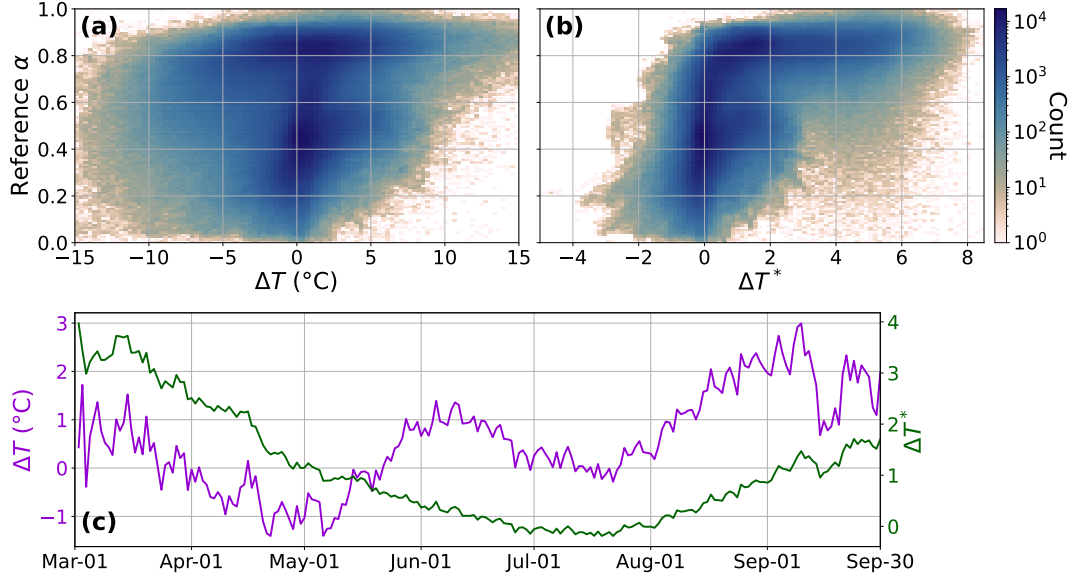
Figure 4. Comparison between the temperature difference \Delta T = T_{2m} - T_{0m} and the weighted temperature difference \Delta T^* = p_{T_{2m}} T_{2m} - p_{T_{0m}} T_{0m} . Panel (a) and (b) show the density heat map for the observed sea ice albedo \alpha and \Delta T and \Delta T^* , respectively, on a logarithmic scale. Panel (c) illustrates the seasonal cycle of observed \Delta T and \Delta T^* from March 1 to September 30 averaged from 2013 until 2020.
