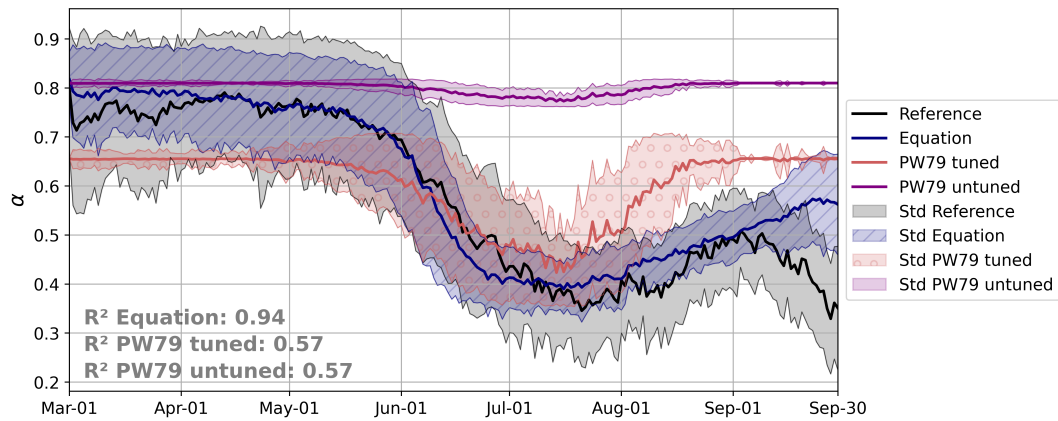
Figure 9. Seasonal sea ice albedo cycle from March 1 to September 30 averaged from 2013 until 2020 observed via the VIIRS satellite instrument (Key et al., 2001, 2016) as reference observation, and computed with the best-performing equation (Eq. 4), and the sea ice albedo parametrization by Parkinson and Washington (1979), here referred to as PW79. The untuned PW79 corresponds to the standard configuration of the Finite-Element Sea Ice Model (FESIM; Danilov et al., 2015), while for a fair data-driven comparison, PW79 is tuned to the training set, including data from 2013 to 2018, using the Nelder-Mead method (Nelder and Mead, 1965).
