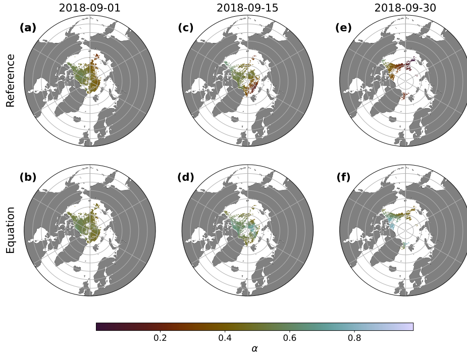
Figure E1. Comparison of sea ice albedo maps between the VIIRS product (reference observation) and Eq. 4 on September 1, 15 and 30, 2018.
