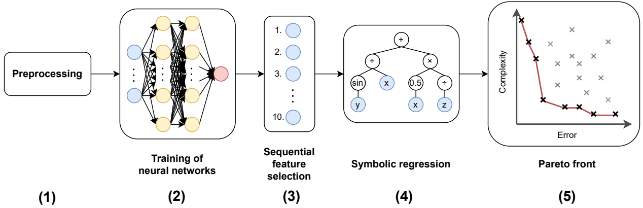
Figure 1. Pareto optimality-based workflow based on Beucler et al. (2024) Beucler et al. (2025) and Grundner et al. (2024), exemplarily for discovering equations with symbolic regression. The process involves: (1) preprocessing of observational and reanalyses data to ensure consistency for the machine learning workflow, (2) training of multilayer perceptron neural networks (NNs), (3) sequential feature selection (SFS) for dimensionality reduction and identification of key features out of ten features governing sea ice albedo, (4) symbolic regression as data-driven equation discovery approach, and (5) comparison between the best-performing equations and baseline models (polynomials and NNs with reduced feature sets chosen by the SFS algorithm) on an error-complexity plane to evaluate how increasing model complexity reduces error.
