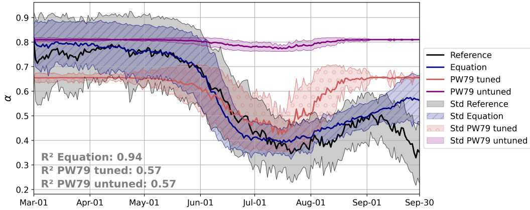
Figure 9. Seasonal sea ice albedo cycle from March 1 to September 30 averaged from 2013 until 2020 observed via the VIIRS satellite instrument (Key et al., 2001, 2016) as ground-truth reference observation , and computed with the best-performing equation (Eq. 4), and the sea ice albedo parametrisation by Parkinson and Washington (1979), here referred to as PW79. The untuned PW79 corresponds to the standard configuration of the Finite-Element Sea Ice Model (FESIM; Danilov et al., 2015), while for a fair data-driven comparison, PW79 is tuned to the training set, including data from 2013 to 2018, using the Nelder-Mead method (Nelder and Mead, 1965).
