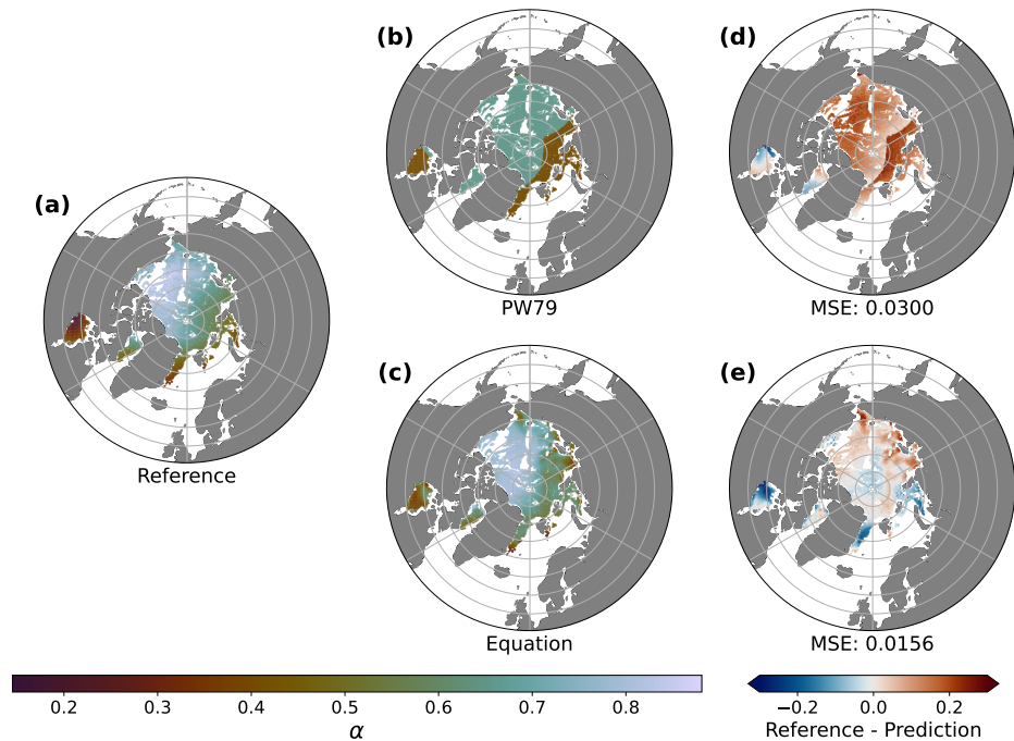
Figure 8. Comparison between (a) the sea ice albedo observed via the VIIRS satellite instrument (Key et al., 2001, 2016) as ground-truth reference observation , (b) the tuned FESIM-parametrisation PW79 , and (c) the best-performing equation (Eq. 4) for May 23rd, 2020. The deviations to the ground-truth reference observation are illustrated in panel (d) for PW79 and panel (e) for Eq. 4.
