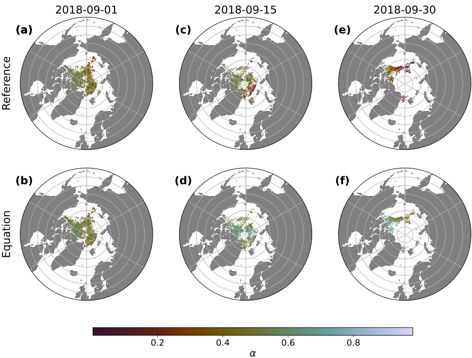
Figure E1. Comparison of sea ice albedo maps between the VIIRS product ( ground-truth reference observation ) and Eq. 4 on September 1, 15 and 30, 2018.
