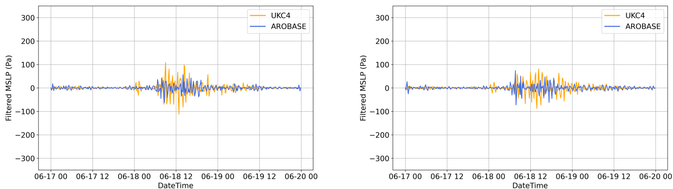
Figure 9. Filtered MSLP time series for the UKC4 (orange) and AROBASE (blue) for the two locations in the Celtic Sea shown as red stars in Fig 8: 50.81°N, 7.04°W (left panel), 51.31°N, 5.77°W (right panel).
