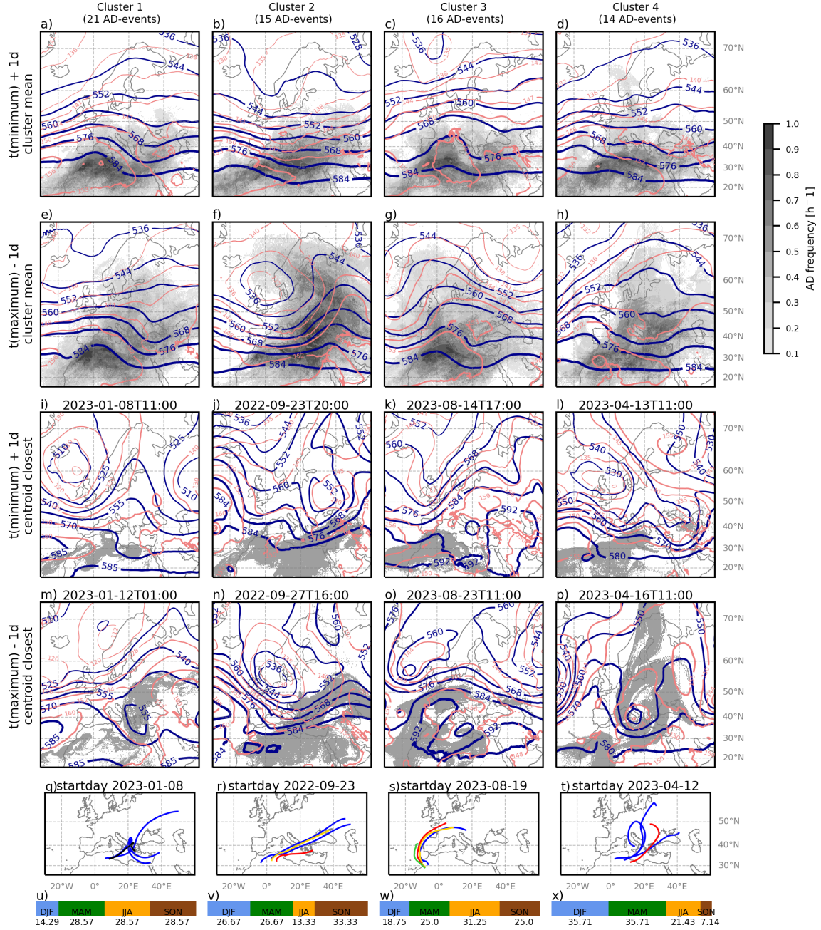
Figure 3. For each of the four clusters (columns): Cluster mean Z_{500} in gpdam (blue contours), mean Z_{850} in gpdam (orange contours) and AD-frequency (grey shading) for the situation at 24h after the onset (a-d), 24h before the AD maximum (e-h). The same is shown for the observation closest to the cluster centroid (i-p, AD-columns shown in grey). Clusters are based on standardised Z_{500} anomalies at 24h before the maximum. Panels q-t show the four trajectory clusters based on the trajectories started on day 5 prior to the AD maximum, colouring of the trajectory clusters is according to the classification algorithm explained in Section 2.4. The bottom row (u-x) shows the seasonal breakdown of each cluster in percent (allocated season for the time of the AD maximum). The number of members in each cluster is given in the column title.
