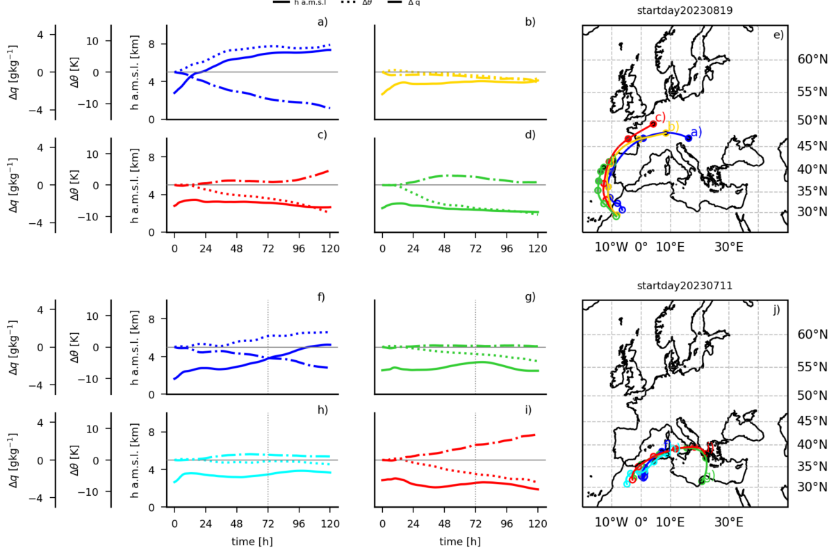
Figure 9. Exemplary display of the trajectory clusters for the trajectories initialised on 19 August 2023 (top) and 11 July 2023 (bottom). The AD maximum is at 24 August 2023, 11 UTC (5 days after initialisation), and 14 July 2023, 06 UTC (3 days after initialisation), respectively. Note that 120 h and 72 h (marked with vertical line in panels f-i) indicate the approximate time around which the AD maximum occurs, respectively. Since the trajectories averaged in the cluster means have varying initialisation times, this time point does not correspond to the exact time for all individual trajectories. Panels a-d and f-i depict the temporal evolution of the individual cluster means. Lines depict h.a.m.s.l (solid), \Delta\theta (dotted), and \Delta q (dash-dotted) with respect to initialisation. Panels e and j show the paths of the cluster means.
