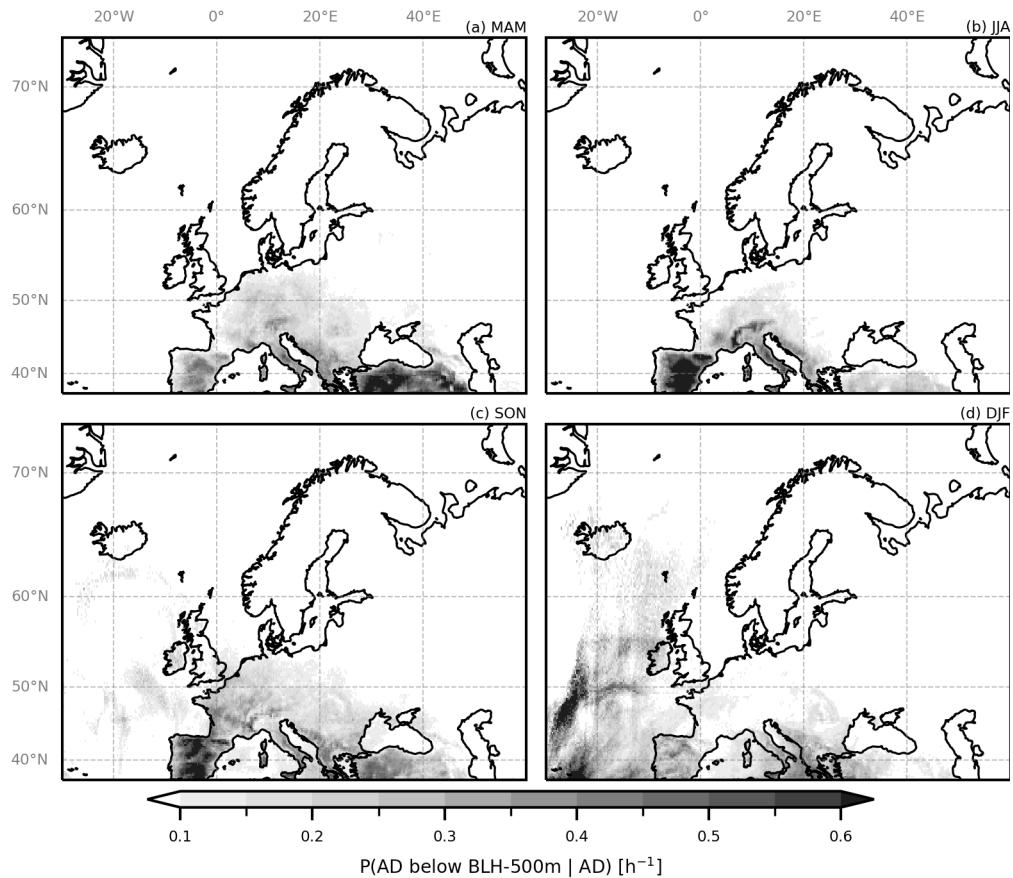
Figure A3. Probability of the lowest AD-cell being within the BL, P(\text{AD below BLH} \mid \text{AD}) , per season.
