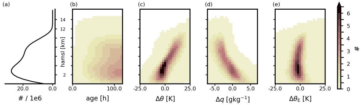
Figure 8. 2D-histograms of cell-averaged changes in trajectories. For each AD-cell ( 0.25^\circ \times 0.25^\circ \times 500 m) all trajectories within are averaged. The histograms depict the distribution of cells in total (a), the average age (b), average differences to the starting location of potential temperature ( \Delta\theta , c), specific humidity ( \Delta q , d), and equivalent potential temperature ( \Delta\theta_E , e), respectively, across all cells north of 37^\circ N and all time steps.
