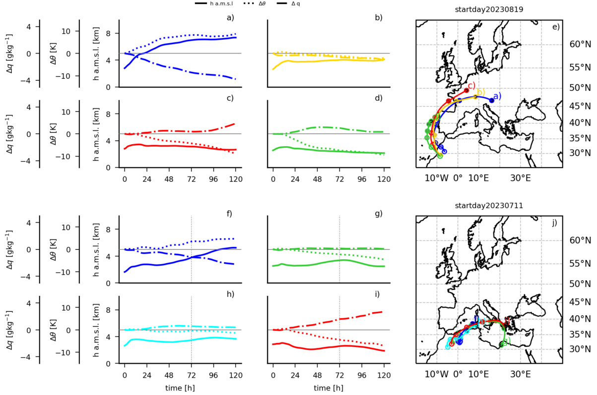
Figure 9. Schematic display of subjectively-identified ‘typical’ trajectory clusters a-f for the trajectories initialised on 19 August 2023 (top) and 11 July 2023 (bottom). x-axis shows The AD maximum is at 24 August 2023, 11 UTC (5 days after initialisation), and 14 July 2023, 06 UTC (3 days after initialisation), respectively. Note that 120 h and 72 h (marked with vertical line in panels f-i) indicate the approximate time around which the AD maximum occurs, respectively. No scales are given. Since the trajectories averaged in the cluster means have varying initialisation times, as this figure is meant to be schematic and should account the exact time for different features to occur at different times or magnitudes all individual trajectories. Solid, dotted, Panels a-d and dash-dotted lines f-i depict the temporal evolution of the individual cluster means. Lines depict differences in h.a.m.s.l (solid), \theta (dotted), and q since \Delta q (dash-dotted) with respect to initialisation, respectively. Panels e and j show the paths of the cluster means.
