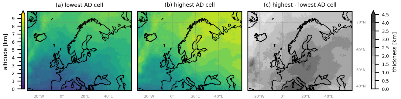
Figure 5. Average altitudes of lowest (a) and highest (b) AD-cells, and their distance (c). This distance describes the maximal thickness of the AD, but it does not depict the actual number of layers present.
