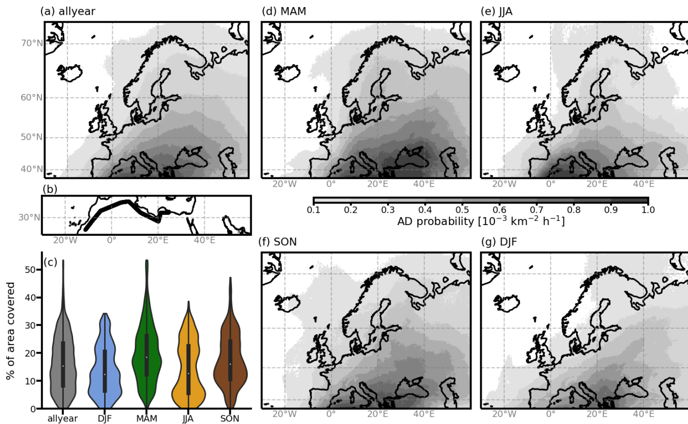
Figure 1. (a) Probability of an AD being present in the respective cell, weighted by the cell's area, for the entire 2-year period (allyear) in the shown domain . (b) Locations of the starting points of the trajectories along the 'curtain'. (c) Violin plot of the percentage of the area in the domain covered by an AD, per season. The violins are normed to have the same area. (d)-(g) Same as (a), but for MAM, JJA, DJF, and SON, respectively.
