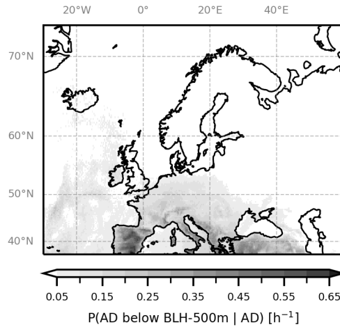
Figure 7. Probability of the the lowest AD-cell being within the BL, P(\text{AD below BLH} \mid \text{AD}) .
