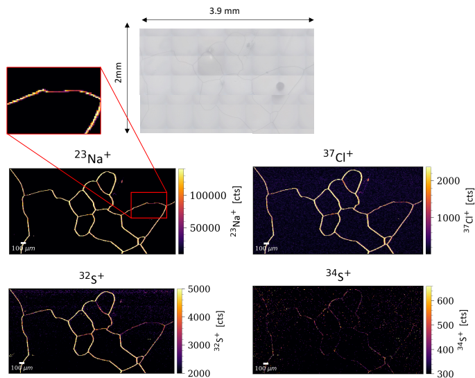
Figure 4: Example map for EDC1819-3, 10µm spot size . The channels for the isotopes ^{33}\text{S} and ^{35}\text{Cl} contain noise only and are therefore not plotted . Shown on the top is the optical mosaic. Note the potential discontinuity in the grain boundary intensity marked by a red square in the ^{23}\text{Na} map and the respective zoom-in on the top left .
