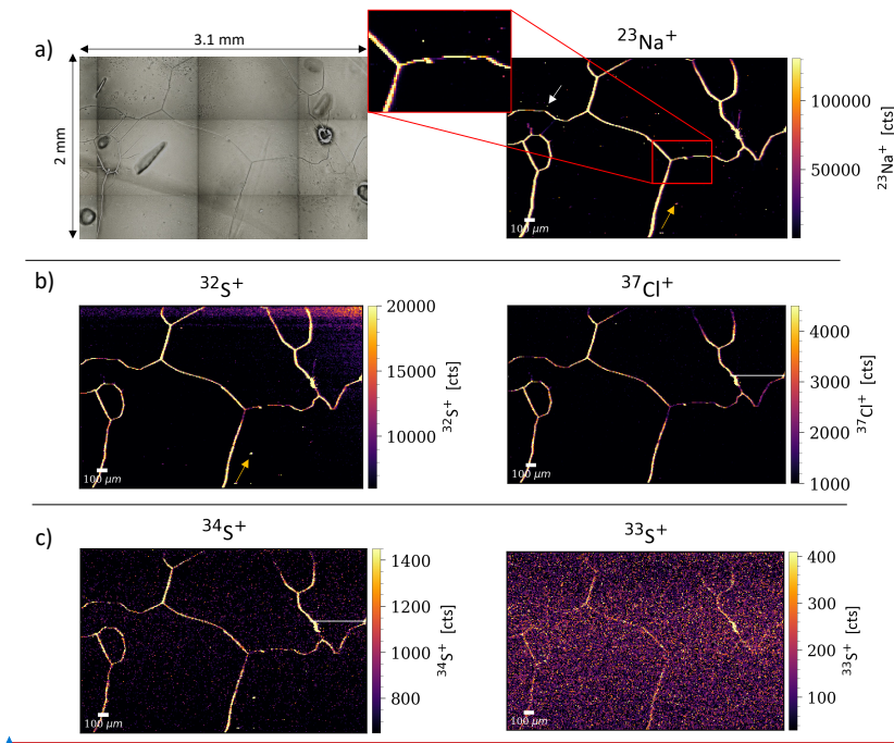
Figure 3: Example map for EDC1819-2, 10 \mu\text{m} spot size. Row a) shows the optical mosaic with dark lines denoting grain boundaries and the map for ^{23}\text{Na} . Note the potential discontinuity in the grain boundary intensity marked by a red square; the same area is shown as a zoom-in section. White and yellow arrows indicate examples of an intra-grain intensity spot for Na only and Na with S, respectively. Row b) contains the maps for the two main channels with signals for S and Cl, ^{32}\text{S} and ^{37}\text{Cl} respectively. Under best case mapping performance, other isotopes of sulfur may also show signals, illustrated in row c). The white horizontal line on the right-hand side in the ^{37}\text{Cl} and ^{34}\text{S} maps is an absence of signal as a result of an autoblanking procedure protecting the detector in the ICP-TOFMS.
