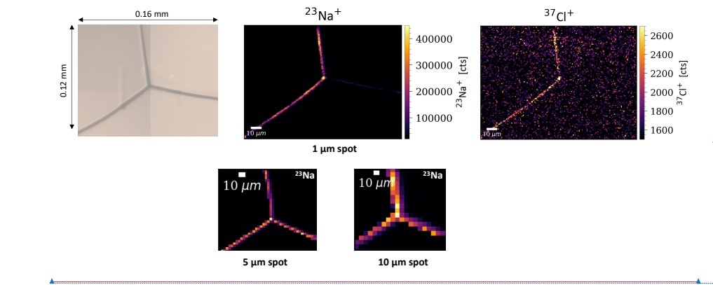
Figure 6: Exemplary investigation into the influence of spot size on detecting enhanced localization at triple junctions versus grain boundaries. The top row shows ultra-high resolution maps of a triple junction recorded at 1 μm spot size, alongside an optical mosaic of the same area. Note that the lower intensity on the right-hand side grain boundary is likely impacted by the scanning-direction, an effect only noticed at this high resolution (see text). The bottom row shows Na maps recorded over the same triple junction with 5 and 10 μm spot size.
