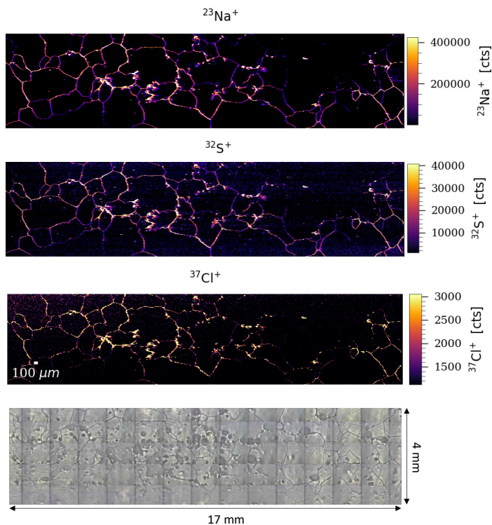
385 Figure 2: Map of EGRIP bag 2286 (20 \mu\text{m} spot, 4 x 17 mm). Shown are intensities in counts (cts) for ^{23}\text{Na} (top row), ^{32}\text{S} 390 and ^{37}\text{Cl} (middle rows) and the optical mosaic (bottom)
