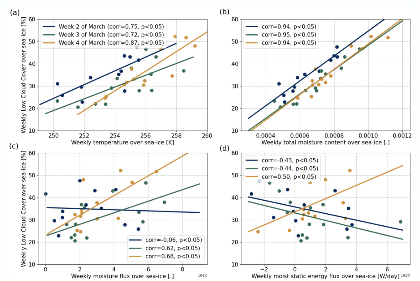
Figure 11. Relationship between weekly average low cloud cover over sea-ice and (a) lower troposphere air temperature, (b) moisture content, (c) poleward moisture flux and (d) poleward moist static energy flux.
