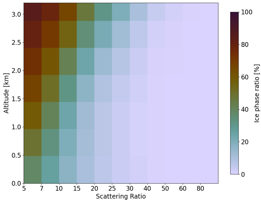
Figure D1. Ice phase ratio over the Arctic sea-ice between March and May computed for each bins of SR and altitude. The ice phase ratio is computed as the ratio between the SR-altitude histograms considering layers classified as ice clouds only and SR-altitude histograms considering layers classified as ice and liquid-containing. CALIPSO-GOCCP monthly gridded SR-altitude histograms by cloud phase were published in Cesana et al., 2013. It highlights the predominance of liquid-containing clouds for SR > 30
