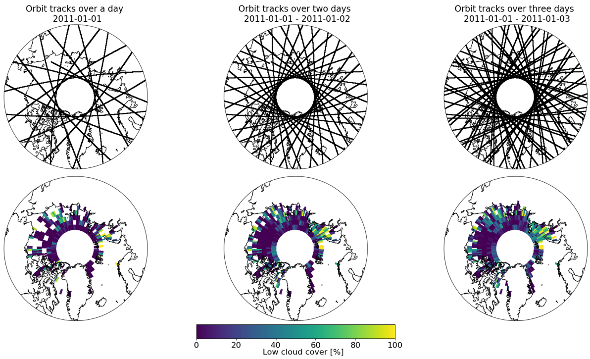
Figure H1. (top) Every CALIPSO orbit tracks over one, two and three days. (bottom) Maps of Low cloud cover averaged over one, two and three days from CALIPSO-GOCCP 2^\circ \times 2^\circ daily gridded data.
