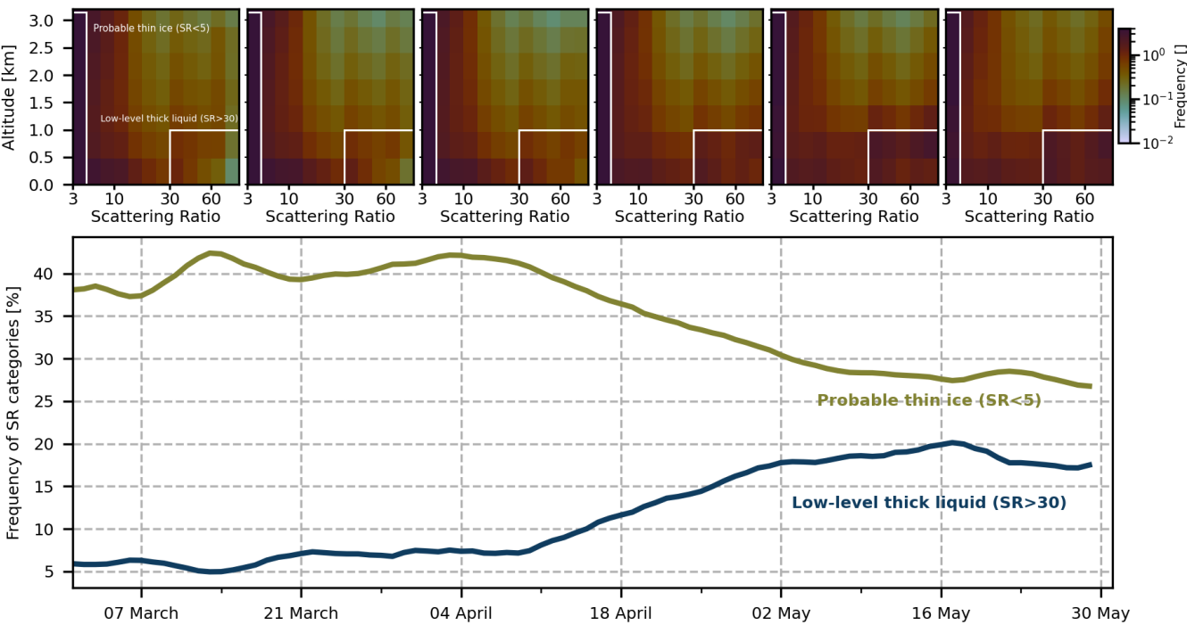
Figure 3. (top panels) Sum of all daily SR histograms over 2-weeks period between March and May from 2008 to 2020 normalized by the total number of occurrences over the period from 0km to 3.2km altitude and SR 3 to 10000. Whites boxes correspond to the categories called on bottom panel. (bottom panel) Evolution of the occurrence frequency of two categories: (green) probable thin ice category and (dark blue) low-level thick liquid-containing category over the Arctic sea-ice covered region between March and May. Data from CALIPSO-GOCCP daily gridded dataset between 2008 and 2020.
