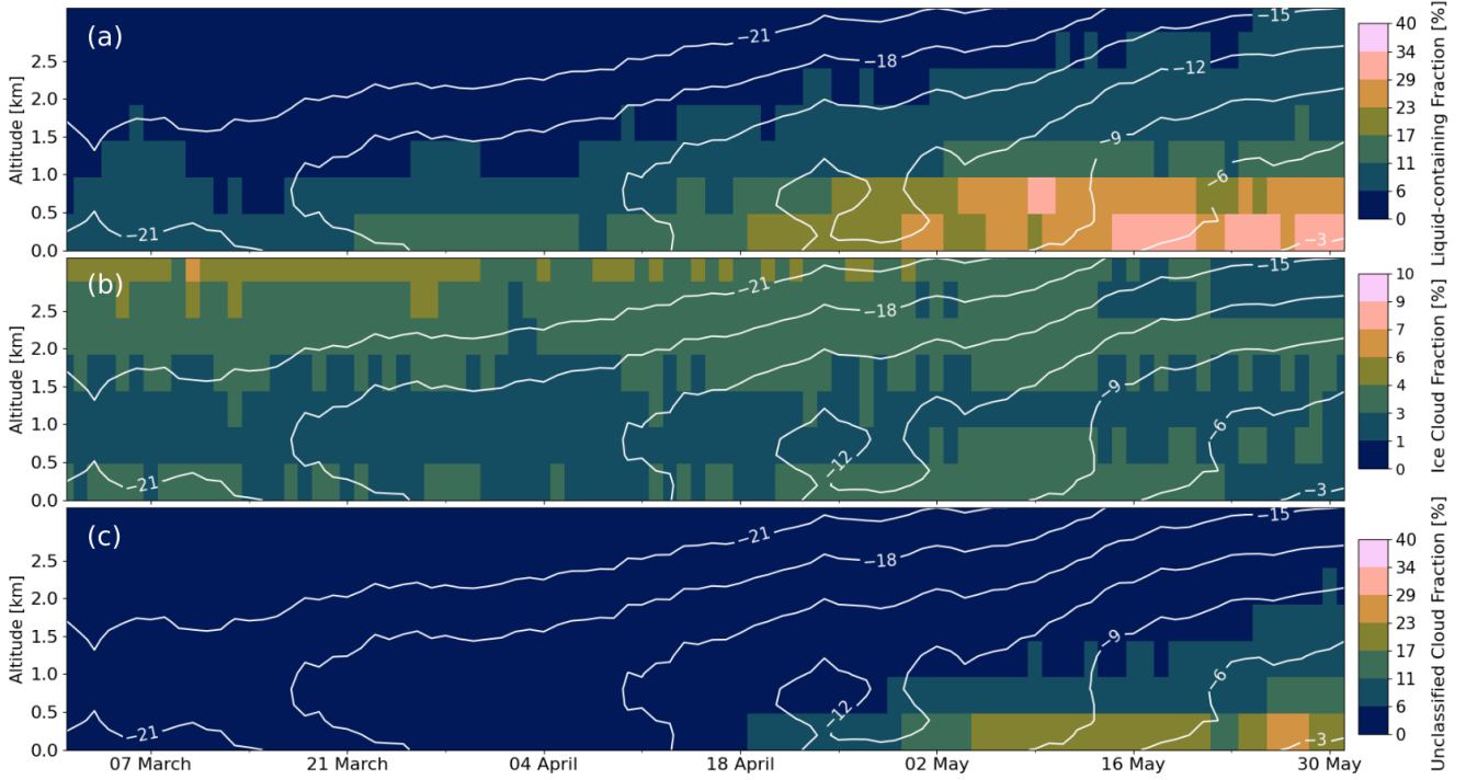
Figure 2. Daily profiles of (a) liquid-containing cloud fraction, (b) ice cloud fraction and (c) unclassified cloud fraction all over the Arctic ice-covered region for 13 years (2008-2020). White contours are air temperature seasonality built from the ERA5 hourly gridded dataset over the Arctic sea-ice covered region. Colorbars are from 0% to 40% for the liquid-containing and unclassified cloud fraction profiles, 0% to 10% for the ice cloud fraction profiles. Data are from CALIPSO-GOCCP daily gridded dataset.
