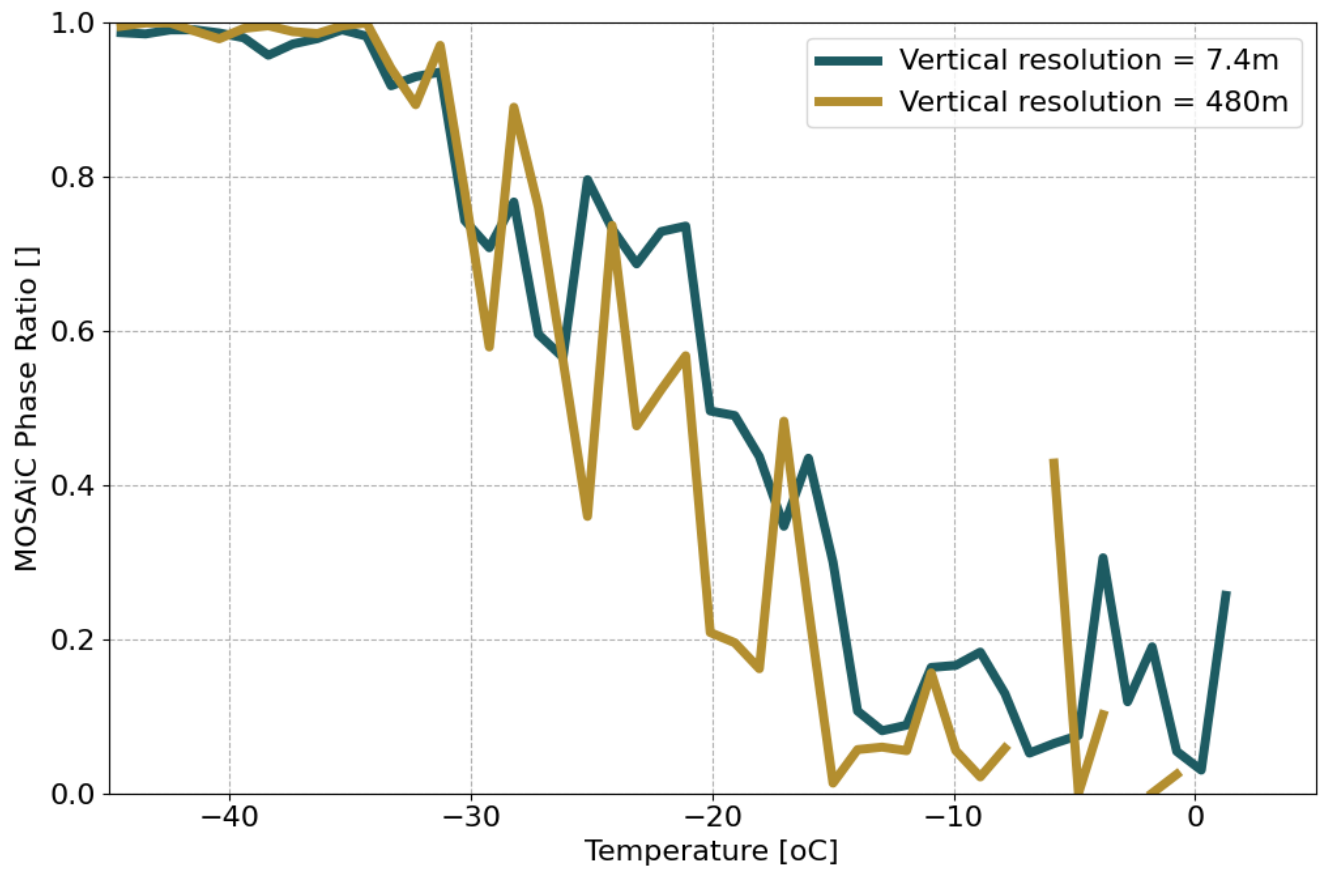
Figure B1. Lidar Ice Phase Ratio from the MOSAiC ground-based lidar at (green line) 7.4 nominal vertical resolution and (yellow line) 480m CALIPSO-GOCCP-like vertical resolution.
