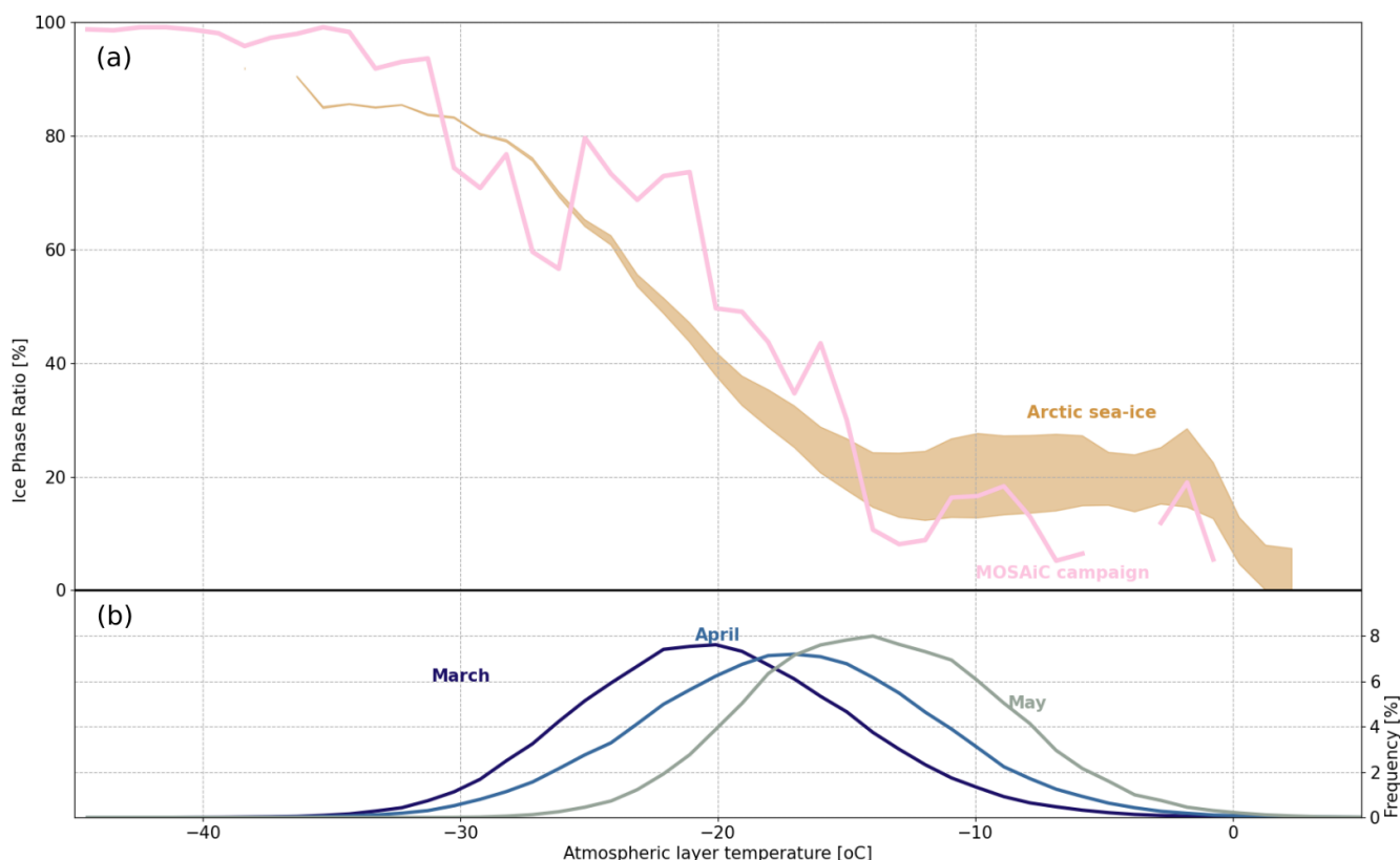
Figure 7. a) Ice phase ratio within clouds as a function of atmospheric layer temperature above the Arctic sea-ice covered region (below 3.2km of altitude) for the 13 years of CALIPSO-GOCCP (orange) and from the MOSAiC observations (pink). The shaded envelope accounts for uncertainty by considering unclassified phase clouds either as ice clouds (upper bound) or excluding them from the ice clouds category (lower bound). The same phase detection methodology is applied to both ground-based and space-based lidar observations. (b) Probability density functions of atmospheric layer temperatures below 3.2km altitude for the months of March, April and May over the Arctic sea-ice covered region for the 13 years studied.
