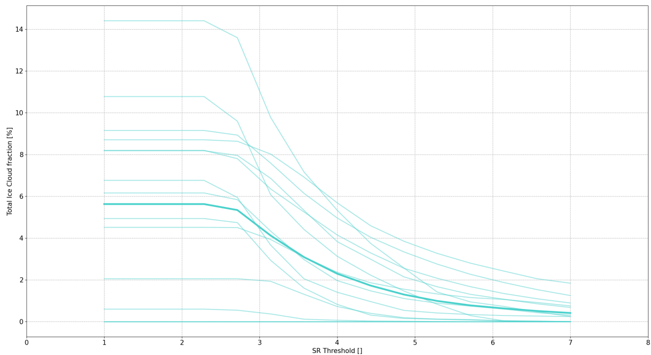
Figure C1. (thin lines) Sensitivity of daily ice cloud fraction (number of ice layer detection divided by total number of layers over a day) to SR cloud detection threshold for each day of March 2020 from the MOSAiC lidar cloud observations. The bold line represents the average sensitivity of the daily ice cloud fraction to the SR threshold over March 2020.
