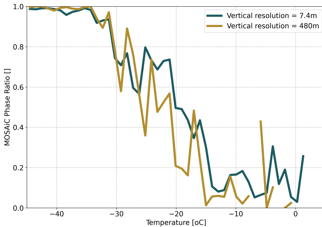
Figure B1. Ice Phase Ratio from the MOSAiC ground-based lidar at (green line) 7.4 nominal vertical resolution and (yellow line) 480m CALIPSO-GOCCP-like vertical resolution.
