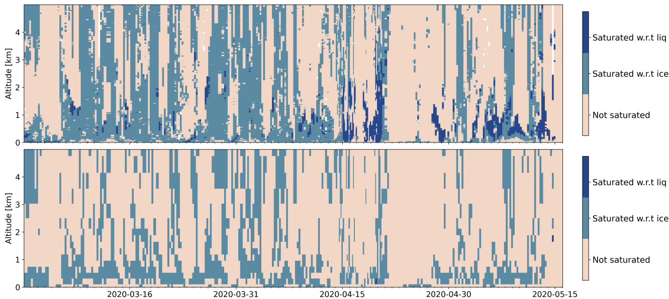
Figure E1. Water vapor saturation state for (top line) MOSAiC radiosoundings and (bottom line) ERA5 collocated to radiosoundings between 1 March 2020 and 15 May 2020.
