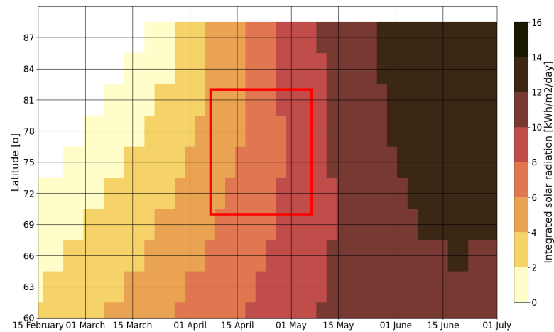
Figure A1. Modeled Integrated solar radiation on a daily scale between February and June, based on the hourly solar angle only.
