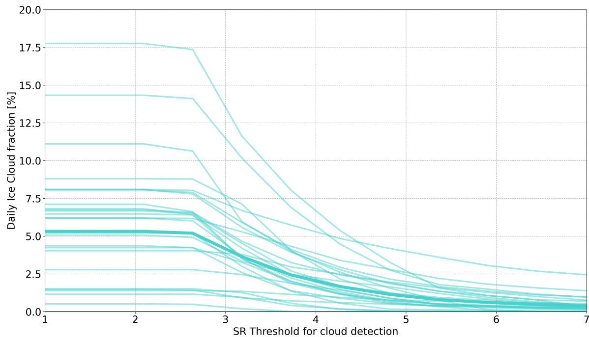
Figure C1. (thin lines) Sensitivity of daily ice cloud fraction (number of ice layer detection divided by total number of layers over a day) to SR cloud detection threshold for each day of March 2020 from the MOSAiC lidar cloud observations. The bold line represents the average sensitivity of the daily ice cloud fraction to the SR threshold over March 2020.
