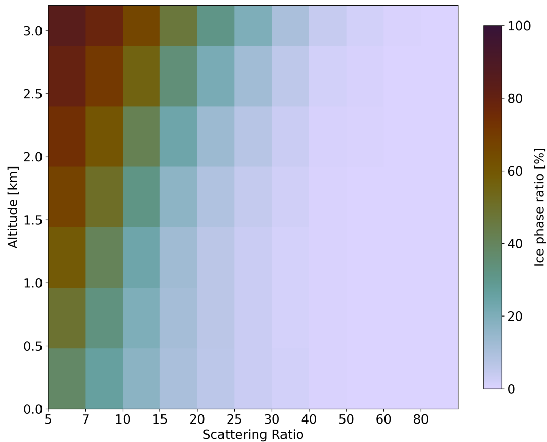
Figure D1. Ice phase ratio over the Arctic sea-ice between March and May computed for each bins of SR and altitude. The ice phase ratio is computed as the ratio between the SR-altitude histograms considering layers classified as ice clouds only and SR-altitude histograms considering layers classified as ice and liquid-containing. CALIPSO-GOCCP monthly gridded SR-altitude histograms by cloud phase were published in Cesana et al., 2013. It highlights the predominance of liquid-containing clouds for SR > 30
