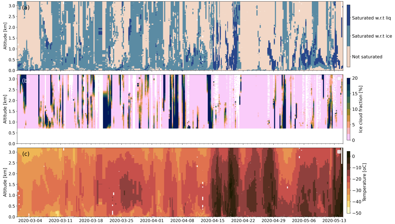
Figure 5. MOSAiC campaign time series of (a) water vapor saturation state (beige=non saturated, light blue=saturated w.r.t ice, and dark blue=saturated w.r.t liquid), RH w.r.t to ice is retrieved from MOSAiC temperature and RH w.r.t liquid measurements based on radiosonde profiles, (b) ice cloud fraction profiles from the MOSAiC ground-based lidar observations where the ice cloud fraction at each altitude bin is computed as the number of ice detections (using SR > 3 ) divided by the total number of valid measurements at the same altitude bin over 6 hours. (c) Temperature measurements from MOSAiC radiosoundings.
