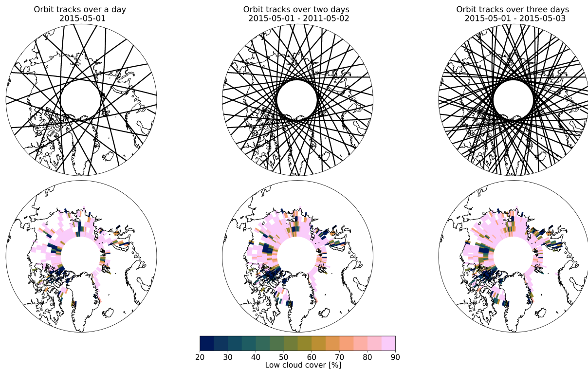
Figure H1. (top) Every CALIPSO orbit tracks over one, two and three days. (bottom) Maps of Low cloud cover averaged over one, two and three days from CALIPSO-GOCCP 2^\circ \times 2^\circ daily gridded data.
