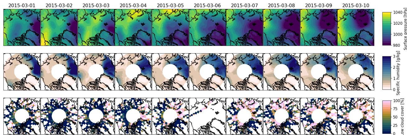
Figure F1. Daily maps of (top panels) surface pressure, (middle panels) mean specific humidity below 800hPa and (bottom panels) low cloud cover during an intrusion event in March 2015. Data of surface pressure and specific humidity are from the ERA5 hourly gridded dataset and low cloud cover from CALIPSO-GOCCP.
