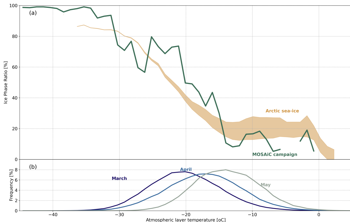
Figure 7. a) Ice phase ratio within clouds as a function of atmospheric layer temperature above the Arctic sea-ice covered region (below 3.2km of altitude) for the 13 years of CALIPSO-GOCCP (orange) and from the MOSAiC observations (green). The shaded envelope accounts for uncertainty by considering unclassified phase clouds either as ice clouds (upper bound) or excluding them from the ice clouds category (lower bound). The same phase detection methodology is applied to both ground-based and space-based lidar observations. (b) Probability density functions of atmospheric layer temperatures below 3.2km altitude for the months of March, April and May over the Arctic sea-ice covered region for the 13 years studied.
