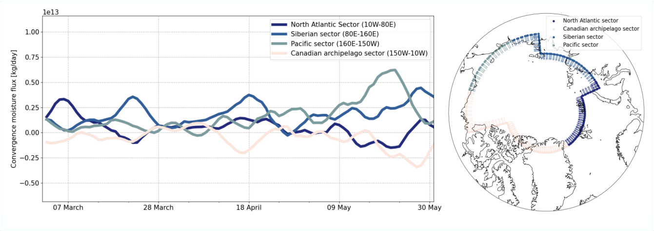
Figure J1. (left) Sensitivity of the poleward moisture flux (shown in Fig.4) to the choice of contour segment (North Atlantic sector, Siberian sector, Pacific sector and the Canadian Archipelago sector). (right) Map of the corresponding contour segments used to compute the poleward moisture flux.
