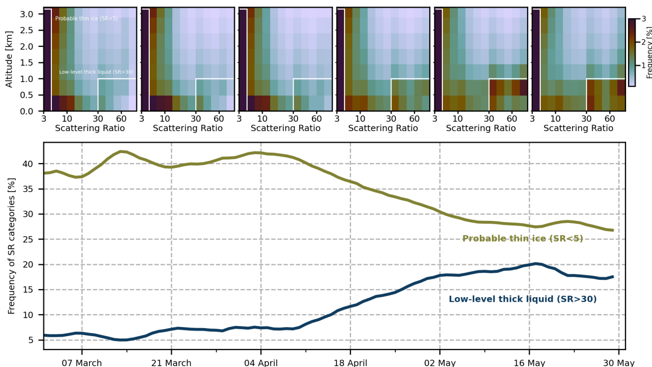
Figure 3. (top panels) Sum of all daily SR histograms over 2-weeks period between March and May from 2008 to 2020 normalized by the total number of occurrences over the period from 0km to 3.2km altitude and SR 3 to 10000. Whites boxes correspond to the categories called on bottom panel. (bottom panel) Evolution of the occurrence frequency of two categories: (green) probable thin ice category and (dark blue) low-level thick liquid-containing category over the Arctic sea-ice covered region between March and May. Data from CALIPSO-GOCCP daily gridded dataset between 2008 and 2020.
