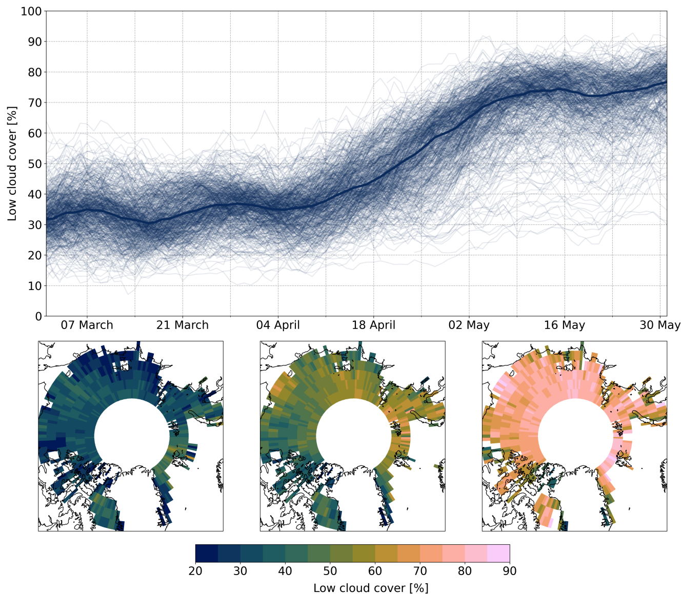
Figure 1. (top panel) Low cloud cover over the Arctic sea-ice covered region between March and May. Each thin blue line is the low cloud cover evolution at each single latitude-longitude pixel averaged over 13 years. The thicker blue line represents the median low cloud cover evolution. (bottom panel) Low cloud cover maps averaged over the first two weeks of March (bottom left), the last two weeks of April (bottom center) and the last two weeks of May (bottom right). Data are from CALIPSO-GOCCP 2^\circ \times 2^\circ daily gridded dataset between 2008 and 2020. See Supplementary.H for additional information on CALIPSO spatial sampling.
