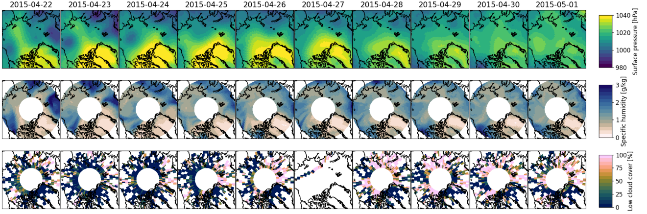
Figure F2. Daily maps of (top panels) surface pressure, (middle panels) mean specific humidity below 800hPa and (bottom panels) low cloud cover during a blocking event in April 2015. Data of surface pressure and specific humidity are from the ERA5 hourly gridded dataset and low cloud cover from CALIPSO-GOCCP.
