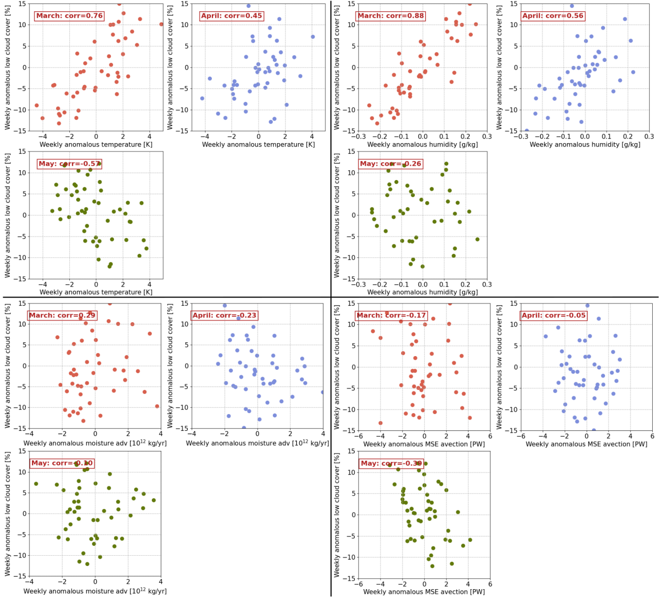
Figure I1. Relationship between weekly average low cloud cover over sea-ice and (upper left quadrant) 950hPa air temperature, (upper right quadrant) 950hPa moisture content, (lower left quadrant) poleward moisture flux and (lower right) poleward moist static energy flux for the weeks of March (orange dots), April (blue dots) and May (green dots). For each weeks, anomalies are defined as the difference between the weekly mean and the corresponding 2008-2020 mean for that same week.
