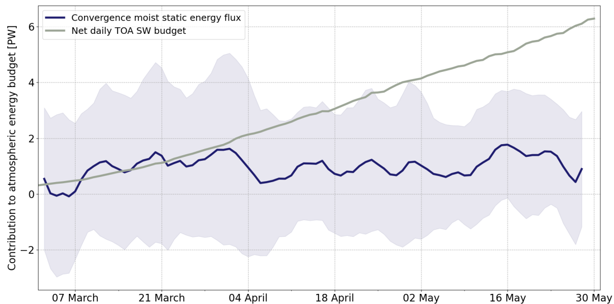
Figure G1. Contribution of horizontal transport of moist static energy and solar radiation to the total atmospheric energy stored over the sea-ice. The net top-of-the-atmosphere shortwave radiation budget (grey line) is integrated over the surface defined in Fig.4 of the present article. The convergence of moist static energy is integrated along the same spatial contour as defined in Fig.4.
