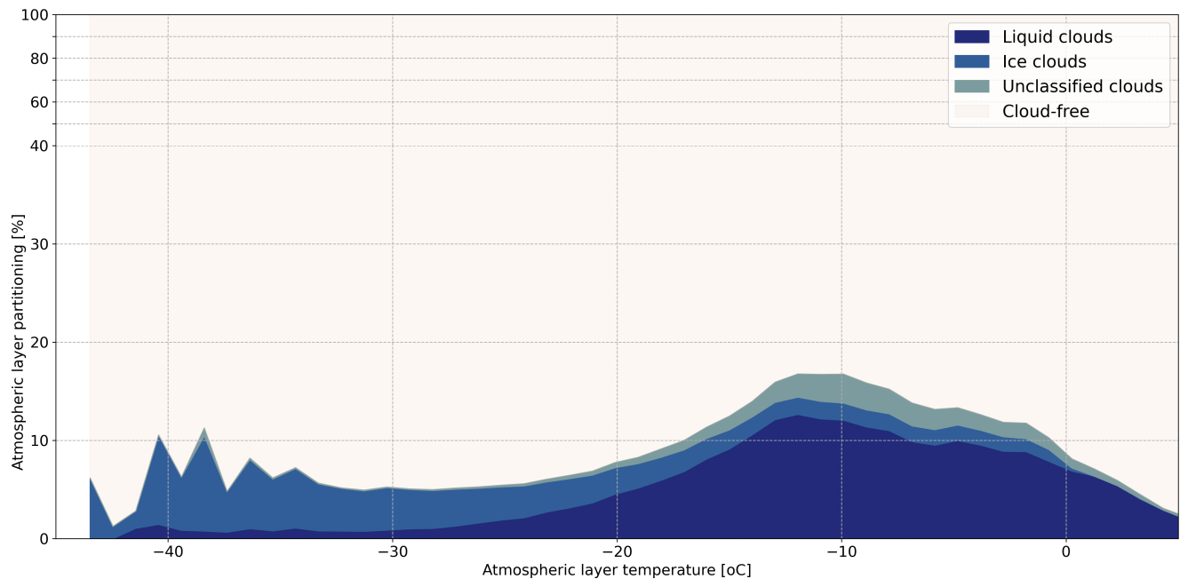
Figure 6. Atmospheric layer partitioning (liquid clouds, ice clouds, unclassified phase clouds and cloud-free) as a function of atmospheric layer temperature, over the Arctic sea-ice covered region below 3.2km altitude.
