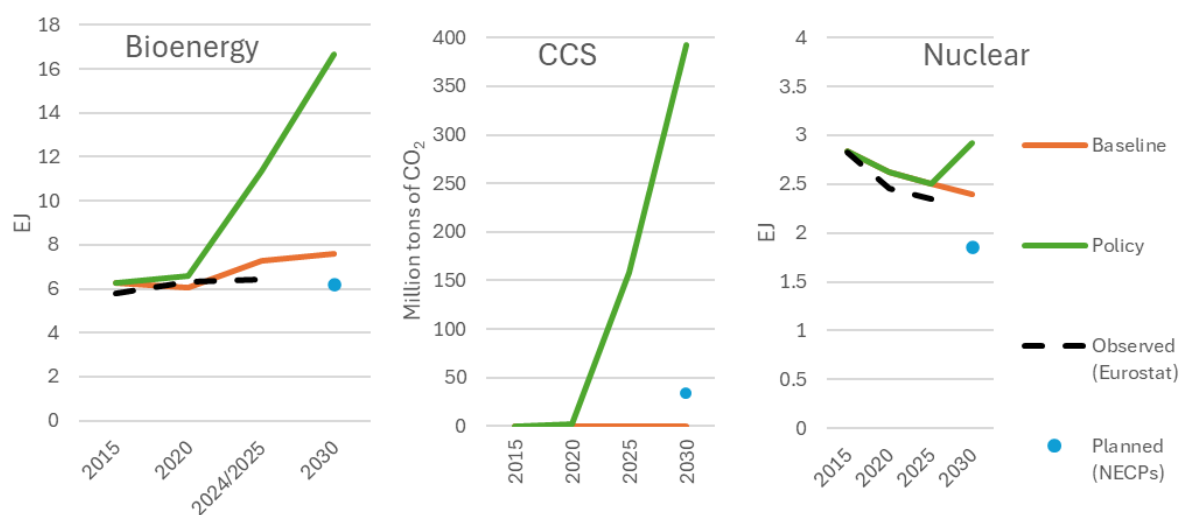
Figure S13: Comparison of model simulations with real-world and projected values for Bioenergy, CCS and Nuclear energy in the EU-27. For Bioenergy, the observed value refers to 2024 due to lack of data for 2025.
