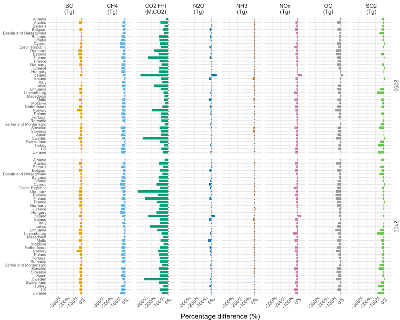
565 Figure 16: Percentage differences in GHG and air pollutant emissions between the policy and the baseline scenarios 570 by period, country, and specie (%).
