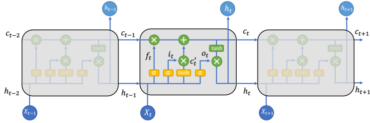
Figure 3: The architecture of the LSTM model.
