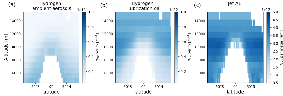
Figure 3. Comparison of average number of ice particles after the vortex downwash per meter formed by hydrogen aircraft ((a) and (b)) and fossil jet fuel aircraft (c). For hydrogen aircraft, the ice particles formed are separated into those formed on ambient aerosol (a) and lubrication oil (b), respectively. Note the difference in scale between all three plots. Hydrogen simulations are run with base setting EUR = 1 , \kappa_o = 6 \cdot 10^{-4} , EI_o = 2 \text{ mg (kg fuel)}^{-1} and lognormal size distribution with geometric mean radius \mu_o = 7.5 \text{ nm} and geometric width \sigma_o \approx 1.45 for lubrication oil droplets. For ambient aerosols we have hygroscopicity parameter \kappa_a = 0.5 and lognormal size distribution with geometric mean radius \mu_a = 15 \text{ nm} and geometric width \sigma_a = 2.2 . All simulations are run for 20 randomly chosen dates (see Supplement S5) as a representative sample for 2019.
