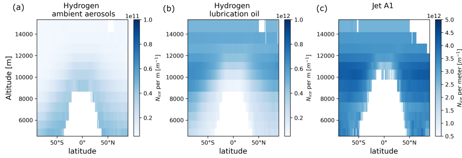
Figure 3. Comparison of average number of ice particles after the vortex downwash per meter formed by hydrogen aircraft ((a) and (b)) and fossil jet fuel aircraft (c). For hydrogen aircraft, the ice particles formed are separated into those formed on ambient aerosol (a) and lubrication oil (b), respectively. Note the difference in scale between all three plots. Hydrogen simulations are run with base setting EUR = 1 , \kappa = 6 \cdot 10^{-6} , EI_o = 2 \text{ mg (kg fuel)}^{-1} and lognormal size distribution with geometric mean radius \mu_o = 7.5 \text{ nm} and geometric width \sigma_o \approx 1.45 for lubrication oil droplets. For ambient aerosols we have hygroscopicity parameter \kappa = 0.5 and lognormal size distribution with geometric mean radius \mu_a = 15 \text{ nm} and geometric mean width \sigma_a = 2.2 . All simulations are run for 20 randomly chosen dates (see Supplement S5) as a representative sample for 2019.
