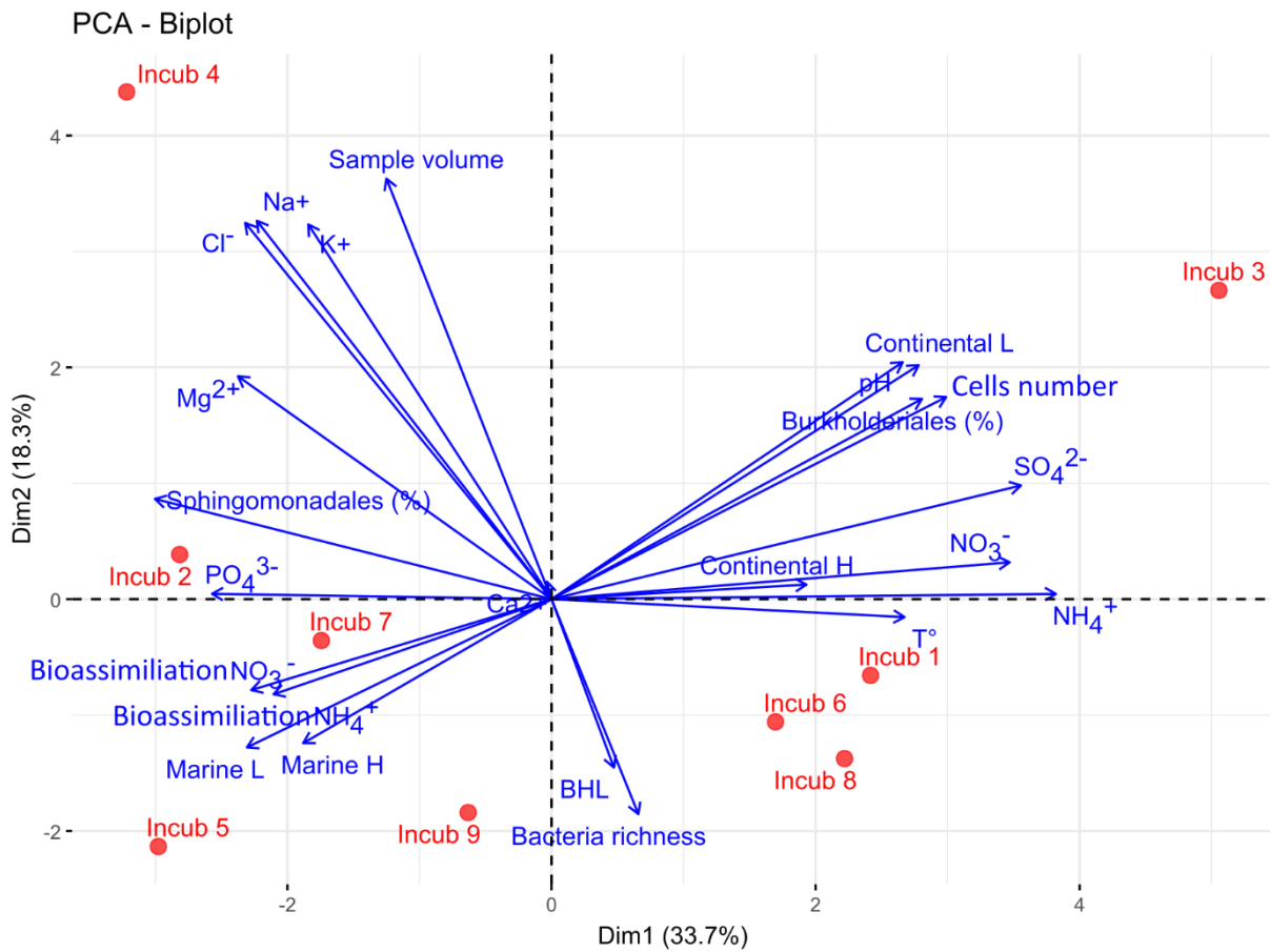
330 Figure 5. Principal component analysis (PCA) between the initial chemical, biological and meteorological variables of rainwater samples and inorganic nitrogen bioassimilation rates during incubations (blue arrows). The red dots represent the different incubations numbered in chronological order. BLH: Boundary Layer Height; L and H for “Marine” and “Continental” air mass origins stand for Low and High altitude, respectively.
