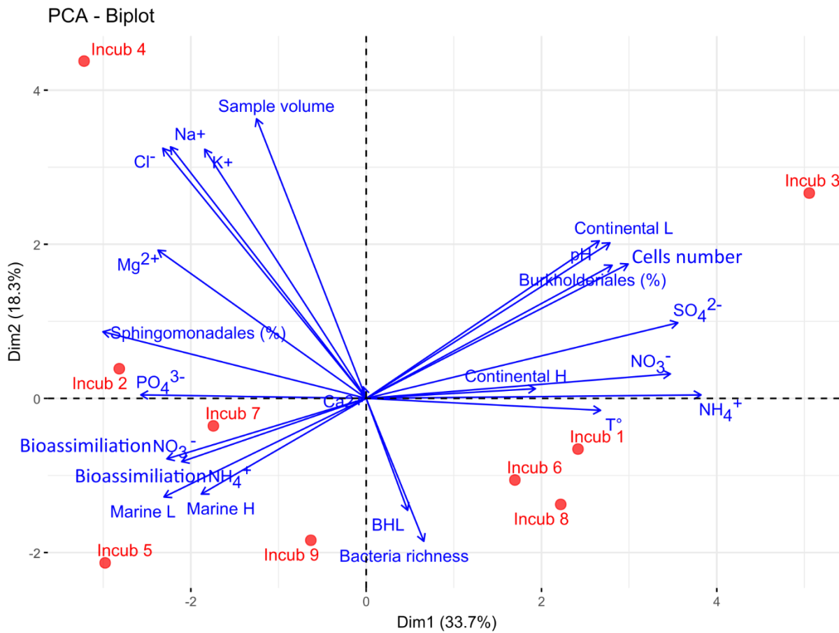
Figure 5. Principal component analysis (PCA) between the meteorological and initial chemical and biological and meteorological variables of rainwater samples and inorganic nitrogen bioassimilation rates during incubations (blue arrows). The red dots represent the different incubations, numbered in chronological order. BLH: Boundary Layer Height; L and H for “Marine” and “Continental” air mass origins stand for indicate Low and High altitude, respectively.
