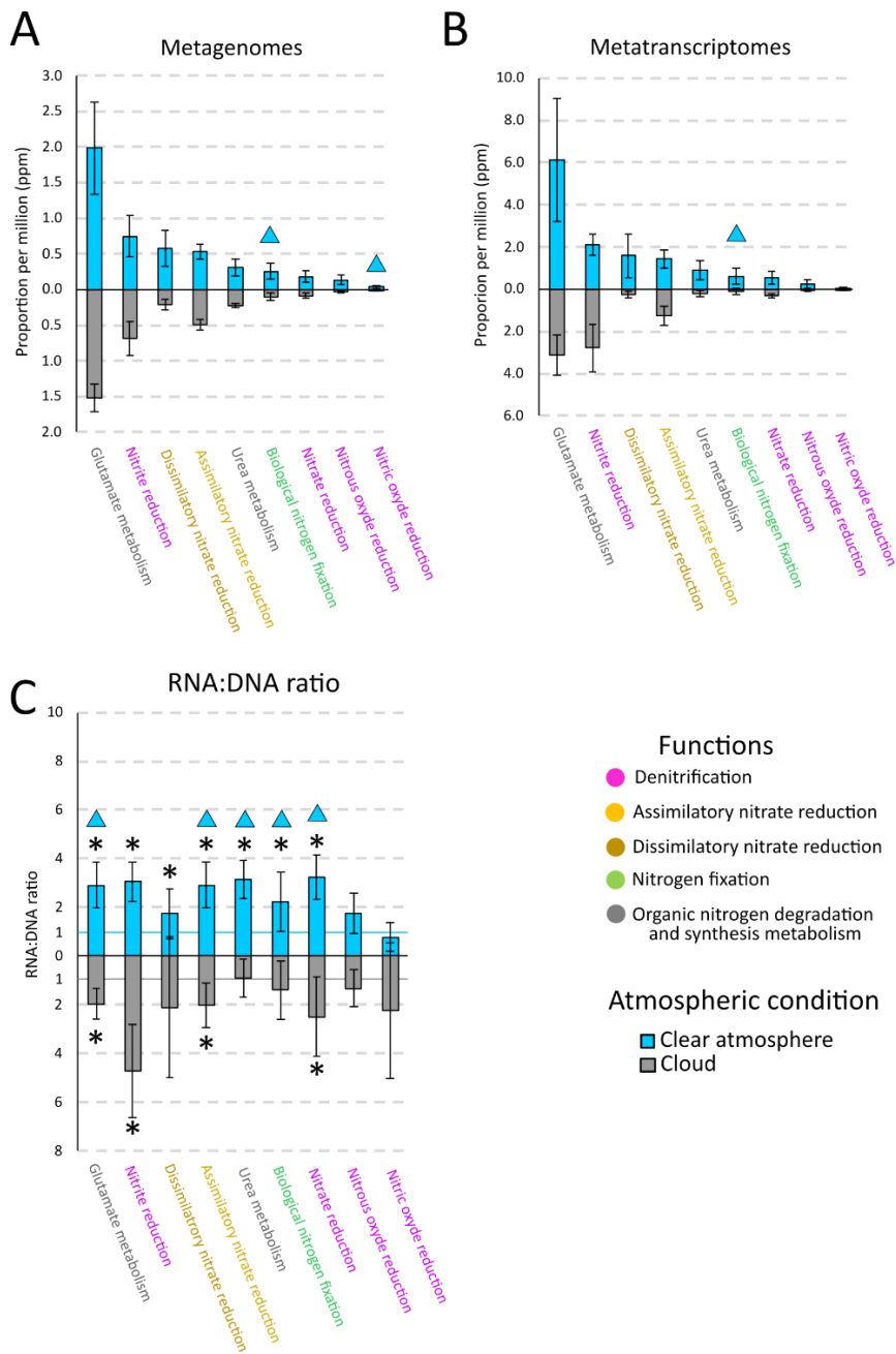
280 Figure 1. Proportions (per million base pairs) of nitrogen processing genes ( with a threshold value greater than 0.1 ppmbp ) in (A) atmospheric metagenomes, (B) metatranscriptomes, and (C) corresponding RNA:DNA ratios, in clouds (grey) or clear atmosphere (blue) at the puy de Dôme mountain station. For (C), the blue line corresponding to the value 1 for clear atmosphere condition and the grey line corresponding to the value 1 for cloud condition. Triangles represent significant differences between clear atmosphere and cloud condition ( Student or Mann-Whitney test ). Asterisks (*) indicate that the RNA:DNA ratio is different from 1 ( Student or Wilcoxon test ).
