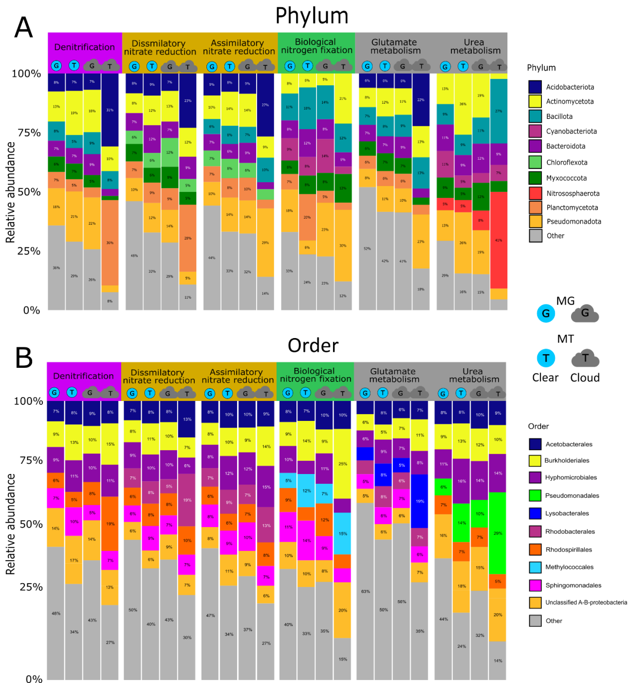
Figure 2. Proportion of bacterial phyla (A) and orders (B) in clear-clear atmosphere and cloud metagenomes (MG) and metatranscriptomes (MT). For each active biological function linked to the nitrogen cycle, (with a threshold value greater than 0.1 ppmbp in MG and MT) , the 8-eight major phyla and orders are represented by different colors. Proportions greater than or equal to 5% are displayed directly on the figure.
