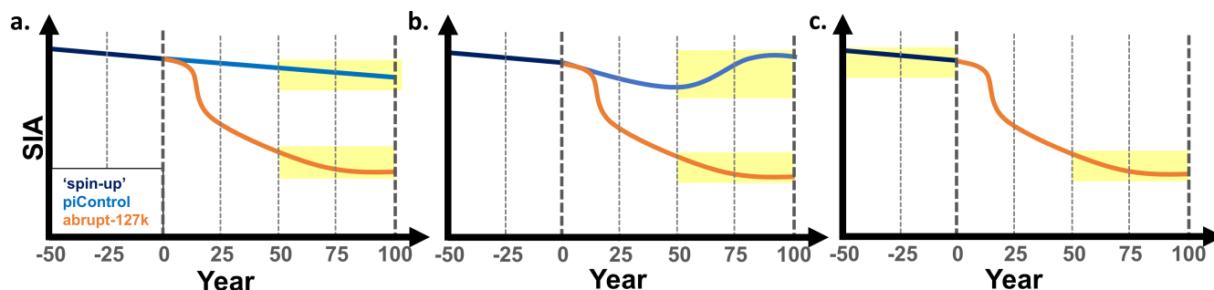
Figure 4. Recommendations for choice of years of piControl which should be used for comparison to abrupt-127k . Recommended procedure is to run both experiments on from the same branch point (same initial condition at year 0). This means that any (a) residual simulation drift and/or (b) low frequency variations can occur in both experiments. If piControl is not run on from the branch point, (c) illustrates that in this case, we recommend differencing from closest pre-branch portion of the piControl (here denoted the ‘spin-up’ simulation and shown in navy).
