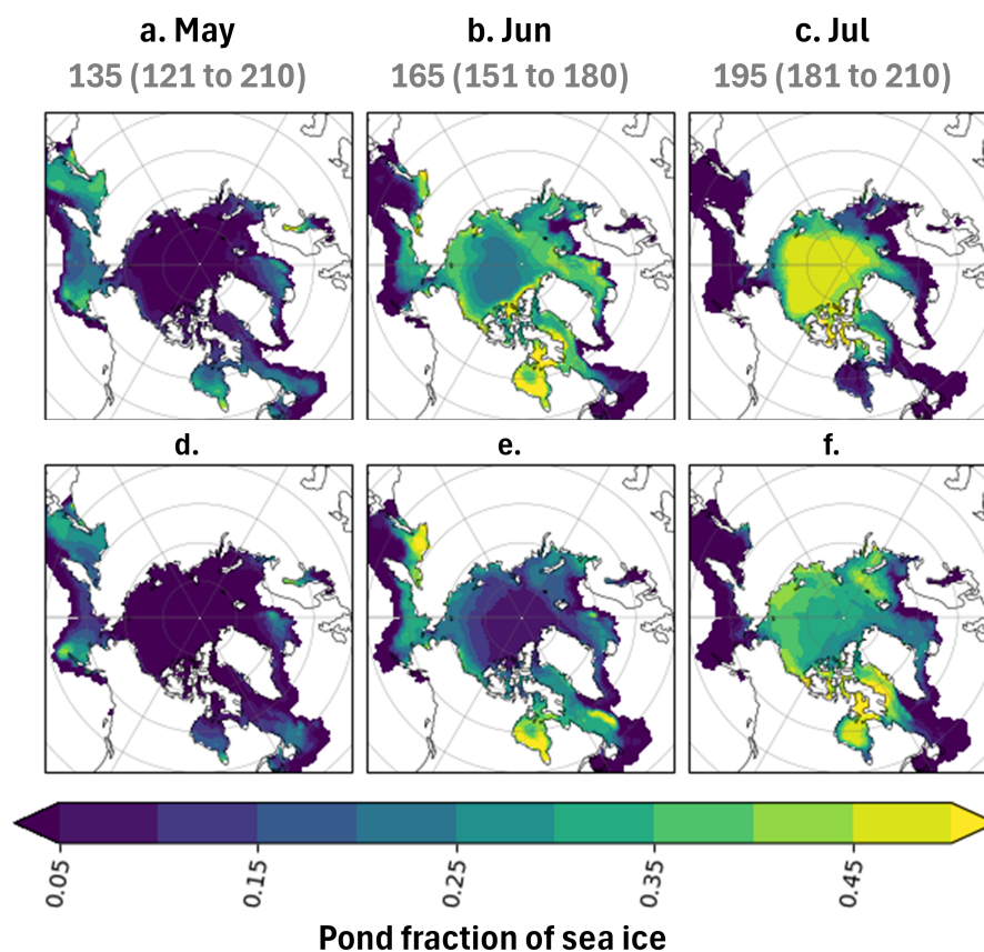
Figure A4. Mean monthly pond-covered fraction of sea ice, over years 50-100 of (a-c) abrupt-127k and (d-f) piControl simulations. HadGEM3 uses a 360-day calendar, so along the x-axis we show both the month and the central 'day of the year' (day range in brackets) for this month in the 360-day calendar.
