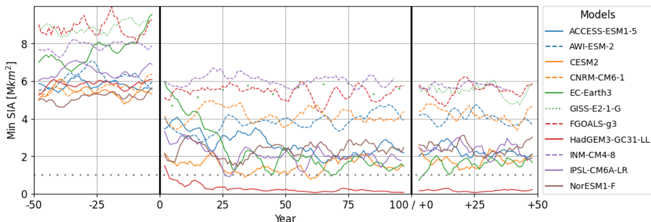
Figure 2. Multi-model evolution of Arctic sea ice area (SIA) minima. 5-year running average of minimum monthly SIA per model for the piControl (left panel), first 100 yrs of lig127k spin-up (centre panel), and fully spun up lig127k (right panel). Solid lines are used for model simulations with at least one practically ice-free summer during the spin up. Dotted lines indicate the model simulation does not drop below the practically ice-free threshold, of 1 \times 10^6 \text{ km}^2 in SIA (shown with horizontal gray dotted line).
