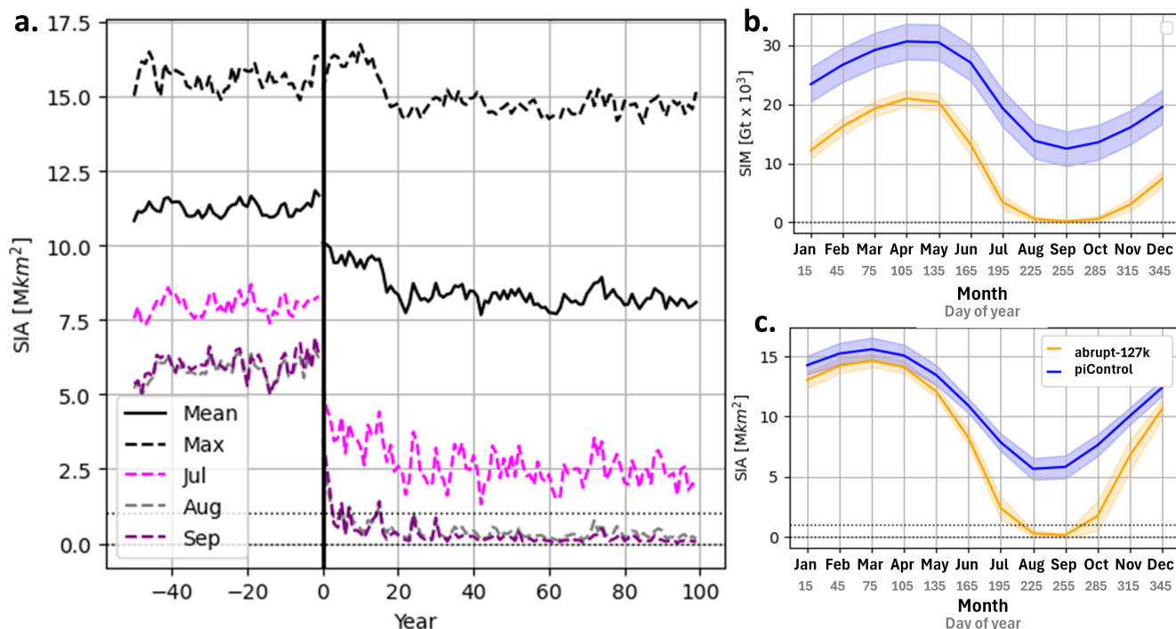
Figure 5. Timeseries and seasonal cycle of Arctic sea ice area (SIA) and sea ice mass (SIM) for example HadGEM3 abrupt-127k simulation. (a) Timeseries of sea ice area (SIA) from years 0 to 100 of abrupt-127k . piControl (shown as years ‘-50-0’) and abrupt-127k (years 0-100). SIA for (pink) July, (grey) August, (purple) September each year, with annual mean SIA as a solid black line, and monthly maximum SIA each year as a dashed black line. After Diamond et al. (2021). Mean monthly value (solid line and shaded area showing twice the standard deviation), for (b) SIA, and (c) sea ice mass. We use years 50-100 of abrupt-127k (orange) and the equivalent years of piControl (blue); HadGEM3 uses a 360-day calendar, so along the x-axis we show both the month and the central ‘day of the year’ for this month in the 360-day calendar. See Appendix C for SIA and SIM definitions.
