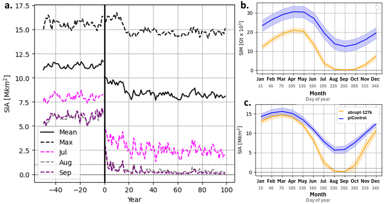
Figure 5. Timeseries and seasonal cycle of Arctic sea ice area (SIA) and sea ice mass (SIM) for example HadGEM3 abrupt-127k simulation. Timeseries and seasonal cycle of Arctic sea ice area (SIA) and sea ice mass (SIM) for the example HadGEM3 abrupt-127k simulation. (a) Timeseries of sea ice area (SIA) from years 0 to 100 of abrupt-127k . piControl (shown as years ‘-50-0’) and abrupt-127k (years 0-100). SIA for (pink) July, (grey) August, (purple) September each year, with annual mean SIA as a solid black line, and monthly maximum SIA each year as a dashed black line. After Diamond et al. (2021). Mean monthly value (solid line and shaded area showing twice the standard deviation), for (b) SIA, and (c) sea ice mass. We use years 50-100 of abrupt-127k (orange) and the equivalent years of piControl (blue); HadGEM3 uses a 360-day calendar, so along the x-axis we show both the month and the central ‘day of the year’ for this month in the 360-day calendar. See Appendix C for SIA and SIM definitions.
