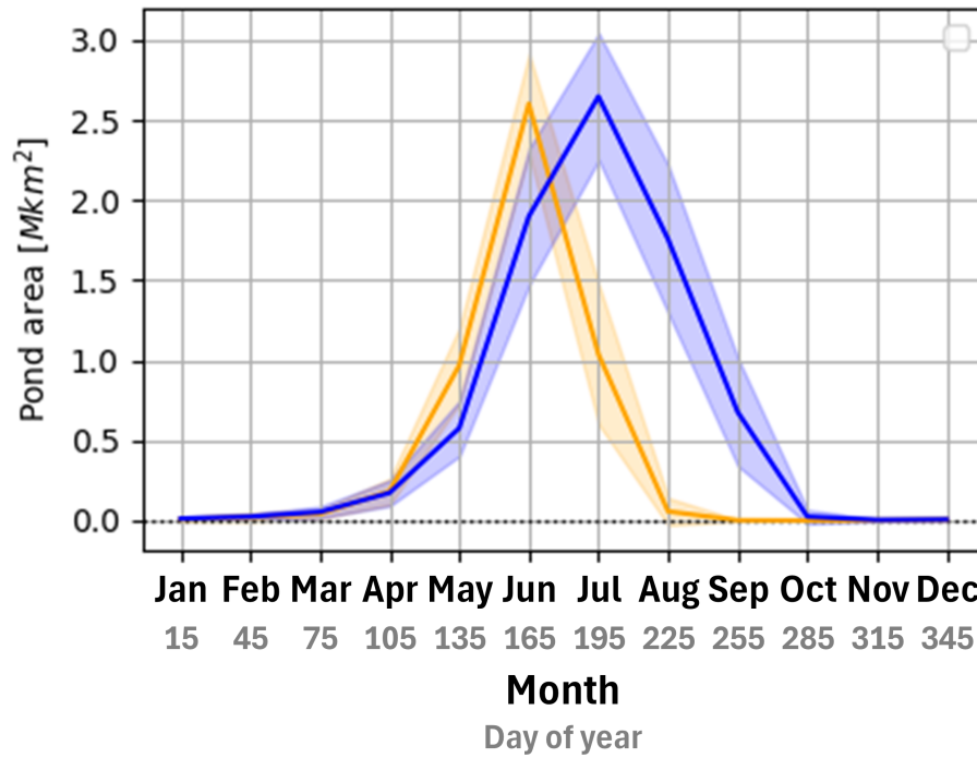
Figure A3. Monthly melt-pond climatology. Total melt-pond area, calculated using years 51-100 of both runs. Result from abrupt-127k (orange) and piControl (blue). HadGEM3 uses a 360-day calendar, so along the x-axis we show both the month and the central ‘day of the year’ for this month in the 360-day calendar.
