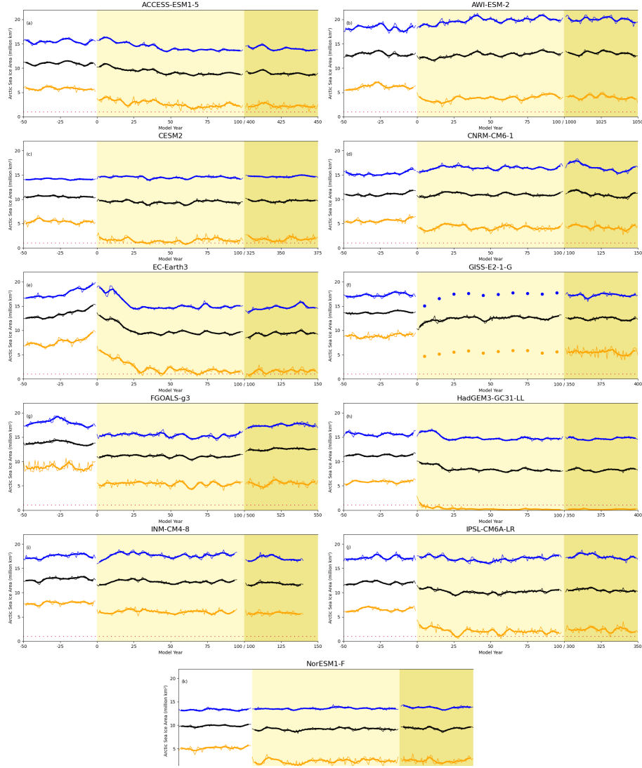
Figure A6. Multi-model evolution of sea ice area. (a-k) Per model breakdown of the data shown in Fig. 2, showing evolution of the annual monthly maximum (blue), average (black) and minimum sea ice area (orange) (after Diamond et al., 2021). Thicker lines show a five-year running mean. Orange dotted lines represent a SIA of 1 \times 10^6 \text{ km}^2 , below which the Arctic is considered sea ice free. For (f), dots show a decadal average due to data limitations.
