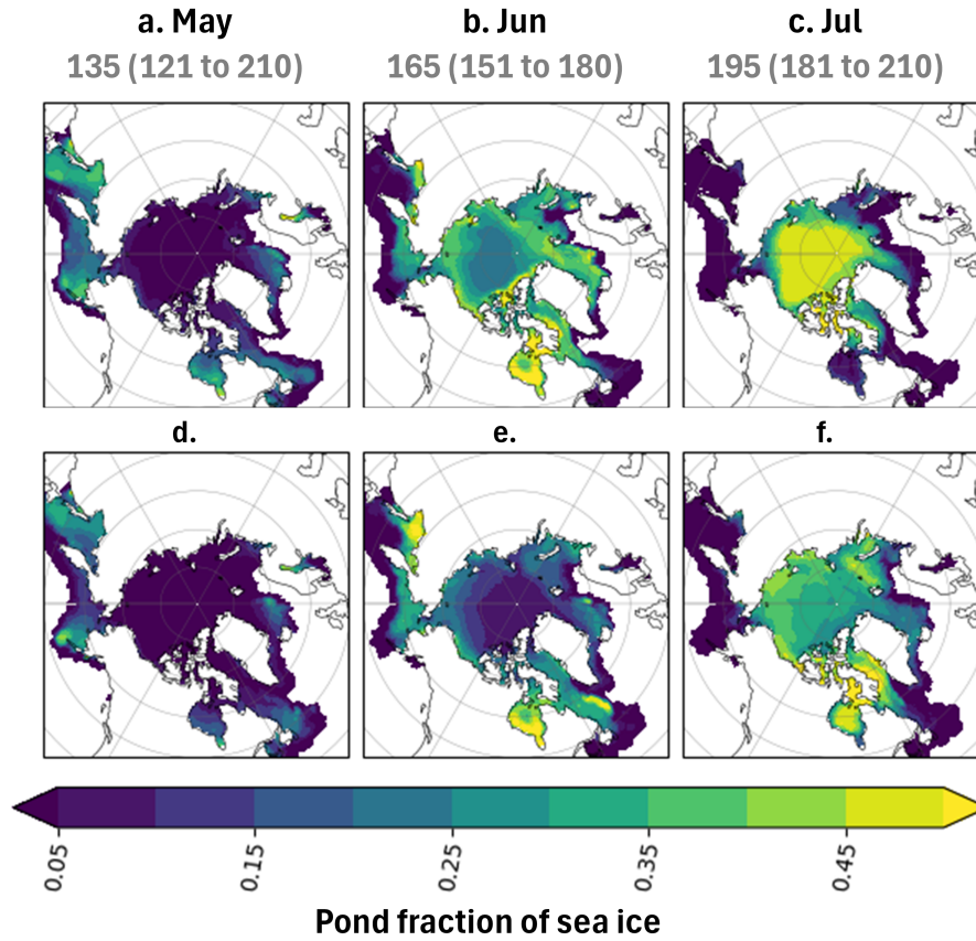
Figure A4. Mean monthly pond-covered fraction of sea ice, over years 50-100 51-100 of (a-c) abrupt-127k and (d-f) piControl simulations. HadGEM3 uses a 360-day calendar, so along the x-axis we show both the month and the central ‘day of the year’ (day range in brackets) for this month in the 360-day calendar.
