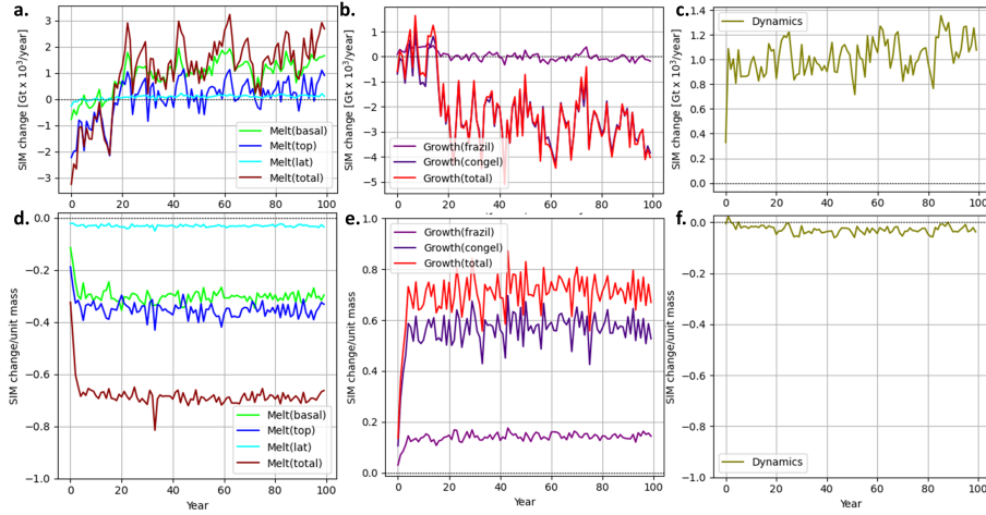
Figure A1. Timeseries as in Figure 8 with additional diagnostics. Additional diagnostics are: (a,d) ‘melt’ variables: basal melt, top melt and lateral melt; (b, e) ‘growth variables’: frazil and congelation growth; (c, f) mass change due to dynamics. Variables in (a-c) are calculated identically to Fig. 8a, and (d-f) are calculated identically to Fig 8b.
