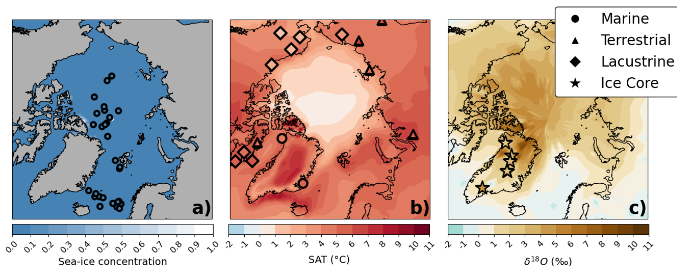
Figure 1. Three lines of evidence for a sea ice free Arctic at 127 ky. (a) Marine core evidence for the minimum sea ice concentration at 127 ky: occurrences of T. quinqueloba (Vermassen et al., 2023), with the climatological minimum-month (September) sea ice concentration from a lig127k simulation run with HadGEM3 (Guarino et al., 2020). (b) Simulated summer (an average of June to August) surface air temperature anomalies from the lig127k HadGEM3 simulation, overlaid with reconstructed summer temperature anomalies (Sime et al., 2023). (c) Ice core \delta^{18}O anomalies from seven Greenland ice core sites (stars) (Domingo et al., 2020), superimposed on simulated annual mean precipitation-weighted \delta^{18}O anomalies from a lig127k HadCM3 simulation with an ice-free summer Arctic Ocean ( c.f. Malmierca-Vallet et al., 2018).
