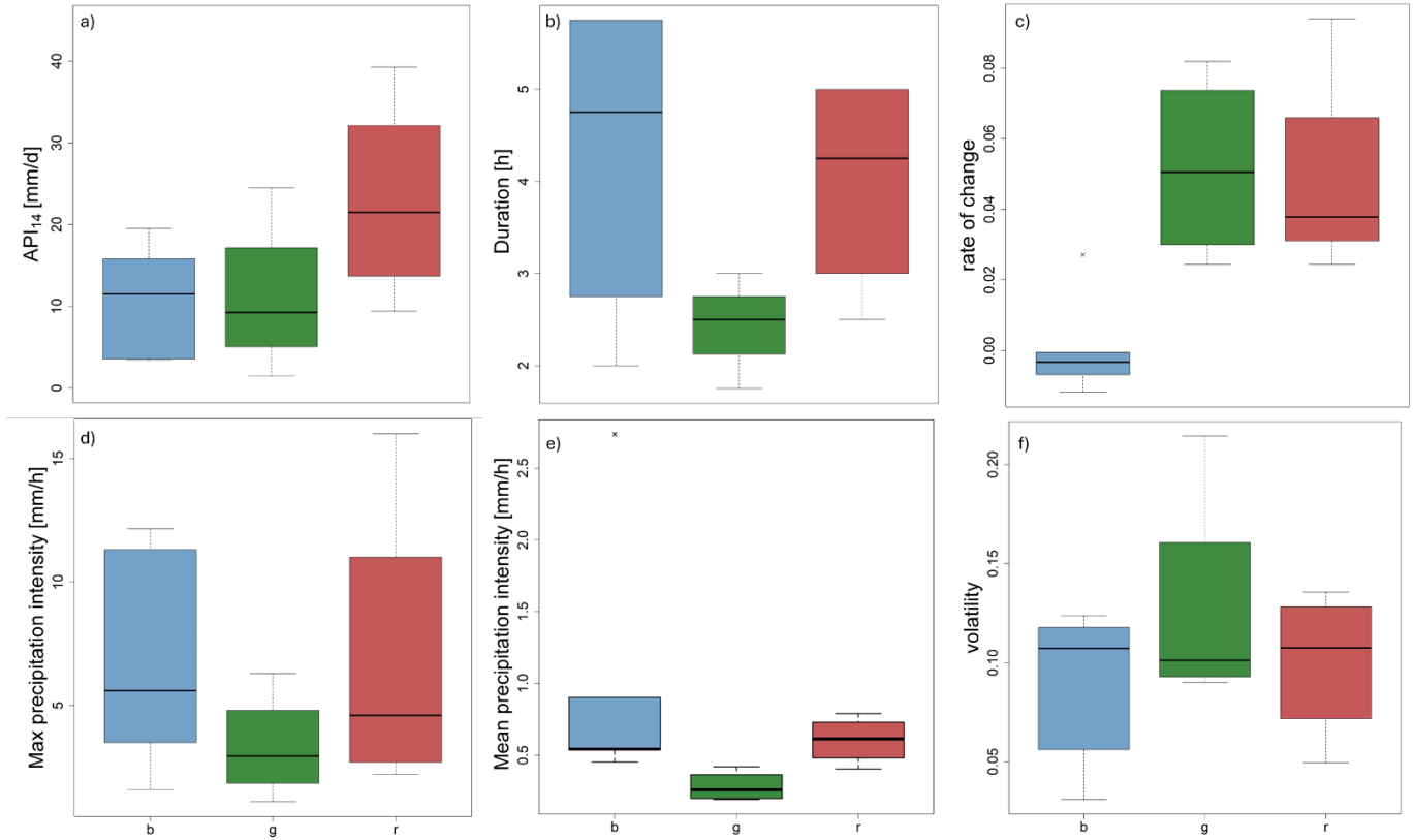
270 Figure 5: Boxplots of hydrological parameters for each cluster of Fig. 4 (a), x-axis values correspond to the cluster color (blue, green, red); a) API_{14} [mm/d]; b) event duration [h]; c) mean rate of change [ L/s^2 ]; d) maximum precipitation intensity in one hour [mm/h]; e) mean precipitation intensity [mm/h]; f) volatility [ L/s^2 ].
