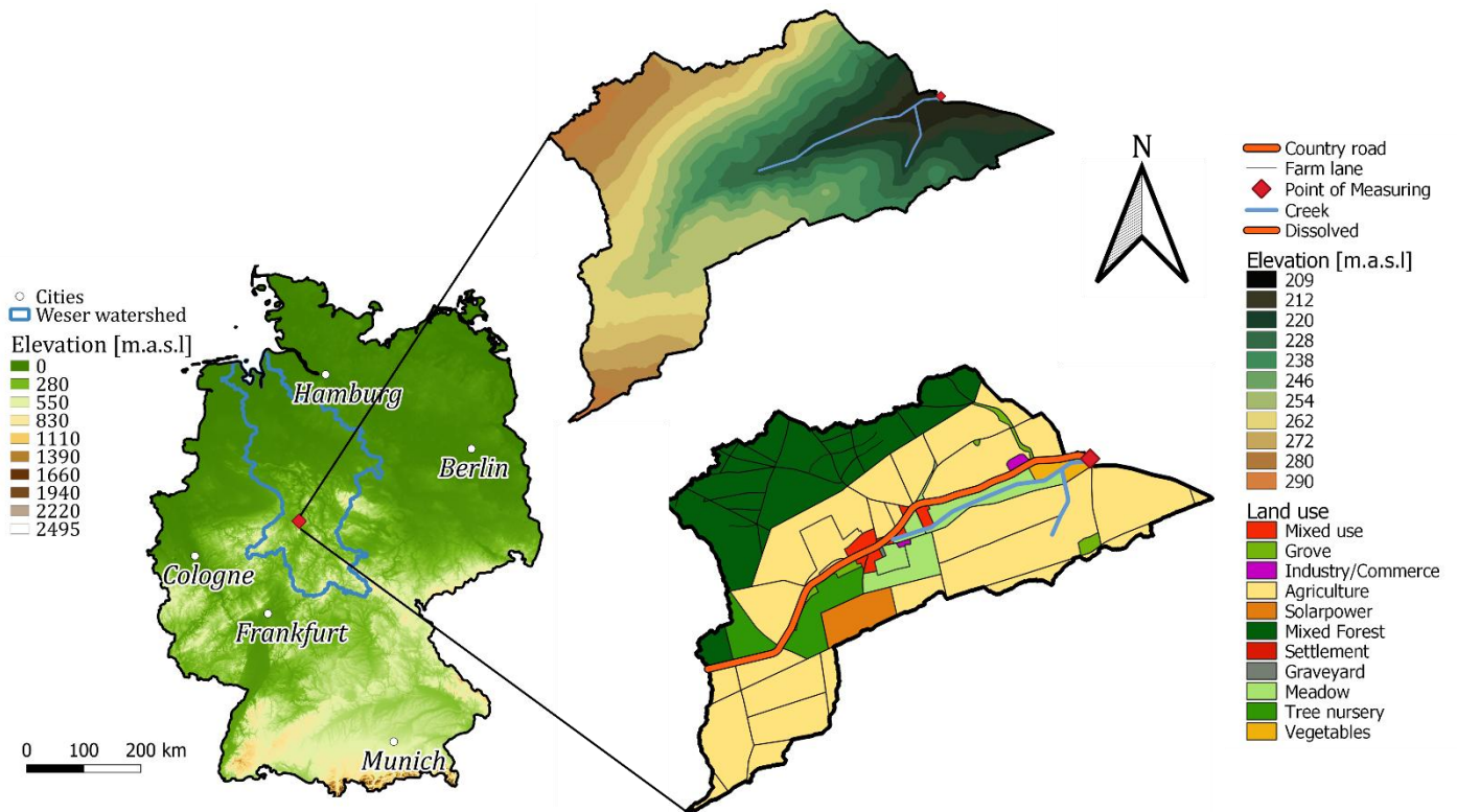
Figure 1: a) Overview, elevation map of Germany; b) Study area, digital elevation model (elevation in meters above sea level (m.a.s.l.)), raster cell resolution 1m. c) Study area, land-use, resolution 1:10000.
