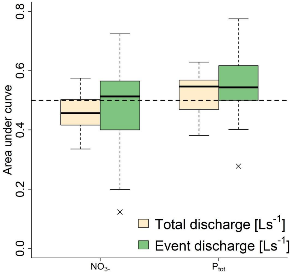
360 Figure 8: Boxplots of the values of area under the curve, for event and total discharge NCL functions of \text{NO}_3^- and \text{P}_{\text{tot}} . High and low values indicate flushing or source depletion.
