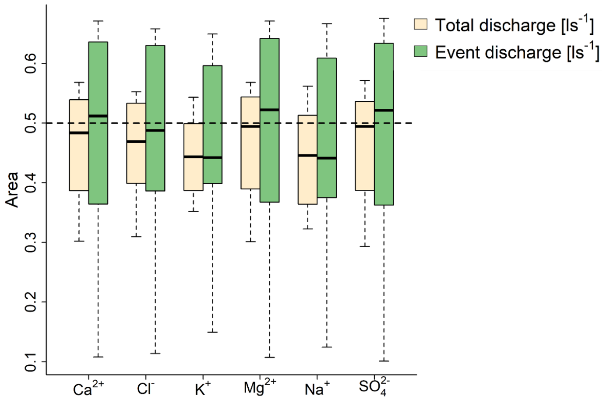
415 Figure 10: Boxplots of areas under the curve for each sampled ion species, the dashed line at 0.5 represents constant export behavior.
