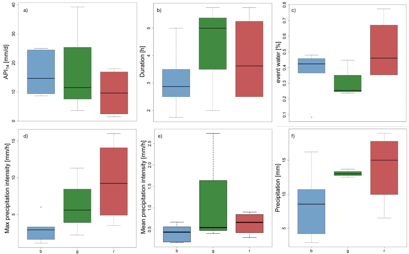
300 Figure 6: Boxplots of hydrological parameters for each cluster of Fig. 4 (b), x-values correspond to the cluster color (blue, green, red); a) API 14 [mm/d]; b) event length [h]; c) mean event water [%]; d) maximum precipitation intensity in one hour [mm/h]; e) mean precipitation intensity [mm/h]; f) total amount of precipitation per event [mm].
