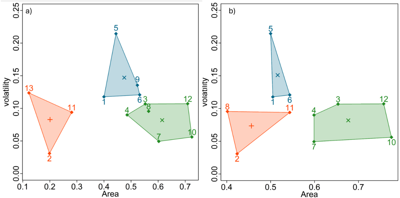
Figure 9: K-Means cluster analysis for volatility of event water discharge functions and area under the curve of fitted NCL functions per event. a) Nitrate load, b) \text{P}_{\text{tot}} load. Centroids of each cluster are marked with x.
