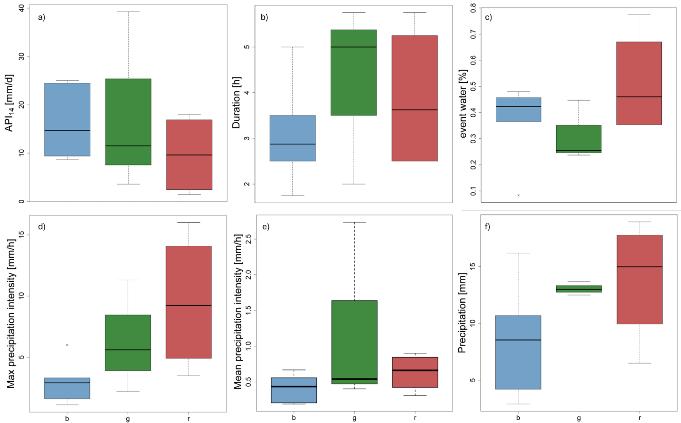
300 Figure 6: Boxplots of hydrological parameters for each cluster of Fig. 4 (b), x-values correspond to the cluster color (blue, green, red); a) API 14 [mm/d]; b) event length [h]; c) mean event water [%]; d) maximum precipitation intensity in one hour [mm/h]; e) mean precipitation intensity [mm/h]; f) total amount of precipitation per event [mm].
