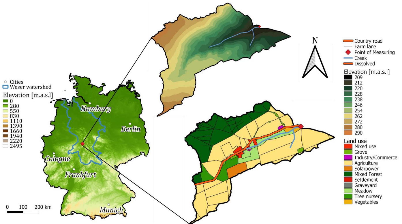
Figure 1: a) Overview, elevation map of Germany; b) Study area, digital elevation model (elevation in m.a.s.l.), raster cell resolution 1m. c) Study area, land-use, resolution 1:10000.
