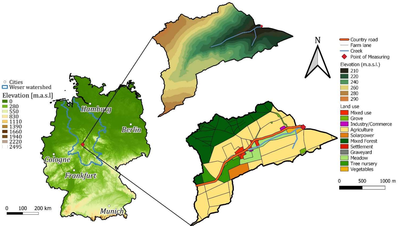
95 Figure 1: a) Overview, elevation map of Germany; b) Study area, digital elevation model (elevation in m.a.s.l.), raster cell resolution 1m. c) Study area, land-use, resolution 1:10000.
