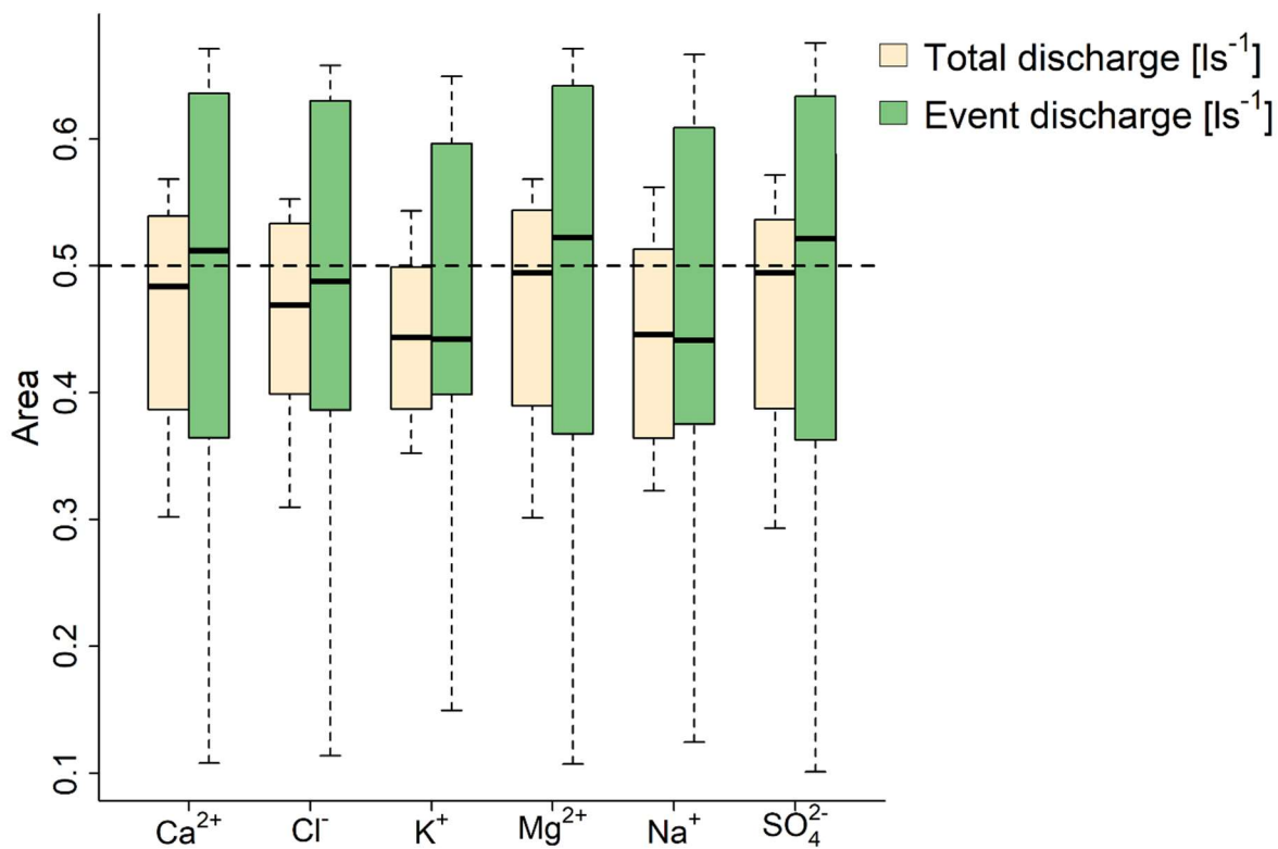
455 Figure 10: Boxplots of areas under the curve for each sampled ion species, the dashed line at 0.5 represents linear-constant export behavior.
