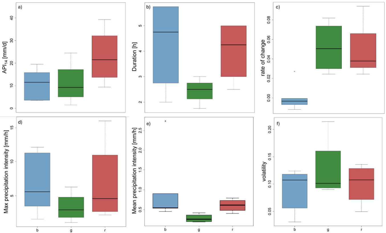
Figure 5: Boxplots of hydrological parameters for each cluster of Fig. 4 (a), x-axis values correspond to the cluster color (blue, green); a) API 14 [mm/d]; b) event duration [h]; c) mean rate of change [L/s 2 ][-]; d) maximum precipitation intensity in one hour [mm/h]; e) mean precipitation intensity [mm/h]; f) volatility [L/s 2 ][-].
