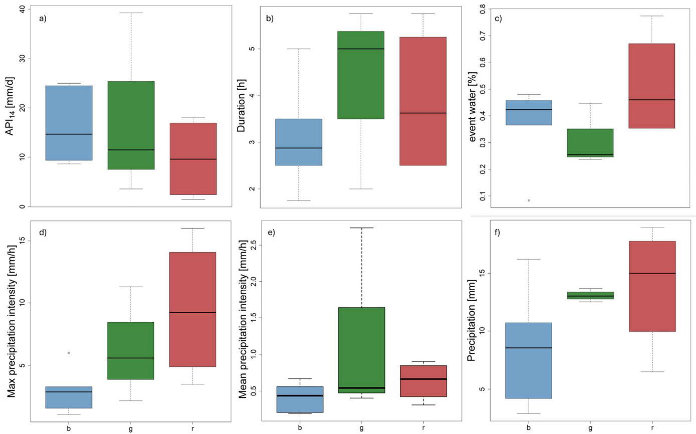
Figure 6: Boxplots of hydrological parameters for each cluster of Fig. 4 (b), x-values correspond to the cluster color (blue, green, red); a) API 14 [mm/d]; b) event length [h]; c) mean event water [%]; d) maximum precipitation intensity in one hour [mm/h]; e) mean precipitation intensity [mm/h]; f) total amount of precipitation per event [mm].
