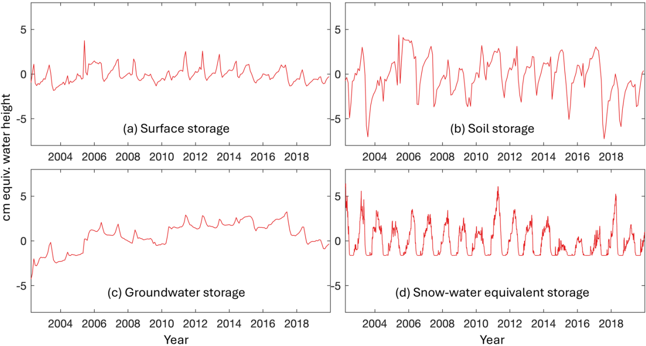
305 Figure 5: Cumulative HGS-based anomalies for (a) surface water storage, (b) soil moisture storage, and (c) groundwater storage, centred around the mean of the GRACE/GRACE-FO baseline period (Jan. 2004 – Dec. 2009). (d) Snow-water equivalent storage is presented as an anomaly with respect to the same baseline but is not cumulated over the availability period.
