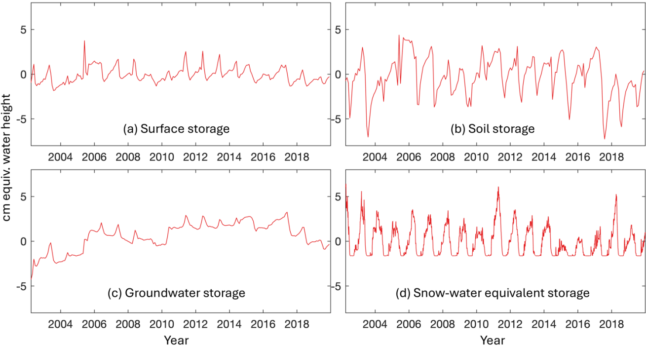
300 Figure 5: Cumulative HGS-based anomalies for (a) surface water storage, (b) soil moisture storage, and (c) groundwater storage, centred around the mean of the GRACE/GRACE-FO baseline period (Jan. 2004 – Dec. 2009). (d) Snow-water equivalent storage is presented as an anomaly with respect to the same baseline but is not cumulated over the availability period.
