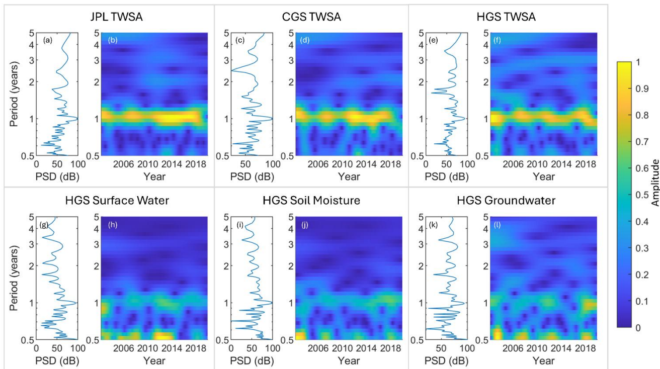
Figure 7: Lomb-Scargle periodograms (power spectral density (PSD), left) and continuous wavelet transforms (right) of the JPL TWSA (a, b), CGS TWSA (c, d), HydroGeoSphere TWSA (e, f), HydroGeoSphere surface water (g, h), HydroGeoSphere soil moisture (i, j), and HydroGeoSphere groundwater (k, l). Amplitude and PSD have been scaled from 0-1 and 0-100 dB, respectively.
