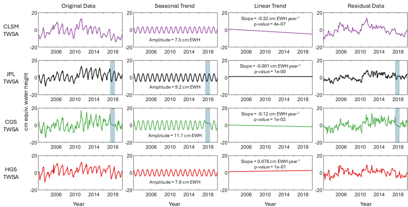
Figure 4: Signal decomposition of terrestrial water storage anomalies from the GLDAS CLSM product, JPL GRACE/GRACE-FO mascon solutions, CGS GRACE/GRACE-FO solutions, and the HydroGeoSphere model. Shading indicates gap between GRACE and GRACE-FO missions.
