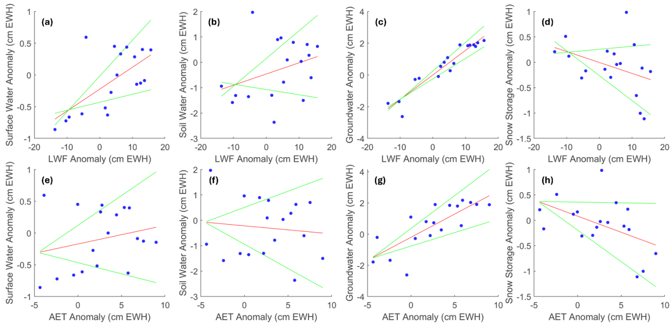
Figure 8: Annual anomaly (cm equivalent water height) in four components of water storage, namely surface water (a, e), soil storage (b, f), groundwater (c, g), and snow water equivalent (d, h), as a function of the annual anomaly in two drivers of hydrological change, liquid water flux (LWF) (a-d) and actual evapotranspiration (AET) (e-h). Linear trends (red) and the respective 95% confidence intervals (green).
