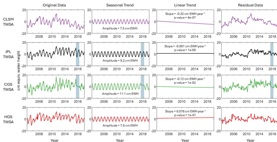
Figure 4: Signal decomposition of terrestrial water storage anomalies from the GLDAS CLSM product, JPL GRACE/GRACE-FO mascon solutions, CGS GRACE/GRACE-FO solutions, and the HydroGeoSphere model. Shading indicates gap between GRACE and GRACE-FO missions.
