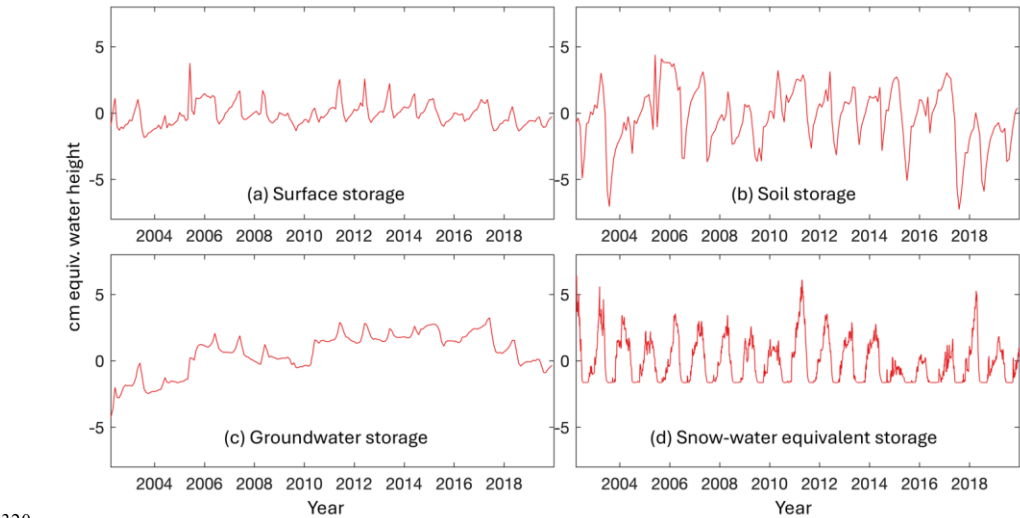
320 Figure 5: Cumulative HGS-based anomalies for (a) surface water storage, (b) soil moisture storage, and (c) groundwater storage, centred around the mean of the GRACE/GRACE-FO baseline period (Jan. 2004 – Dec. 2009). (d) Snow-water equivalent storage is presented as an anomaly with respect to the same baseline but is not cumulated over the availability period.
